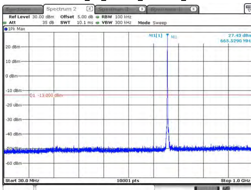
CH133147_5M_16-QAM_Below 1G_1RB12
