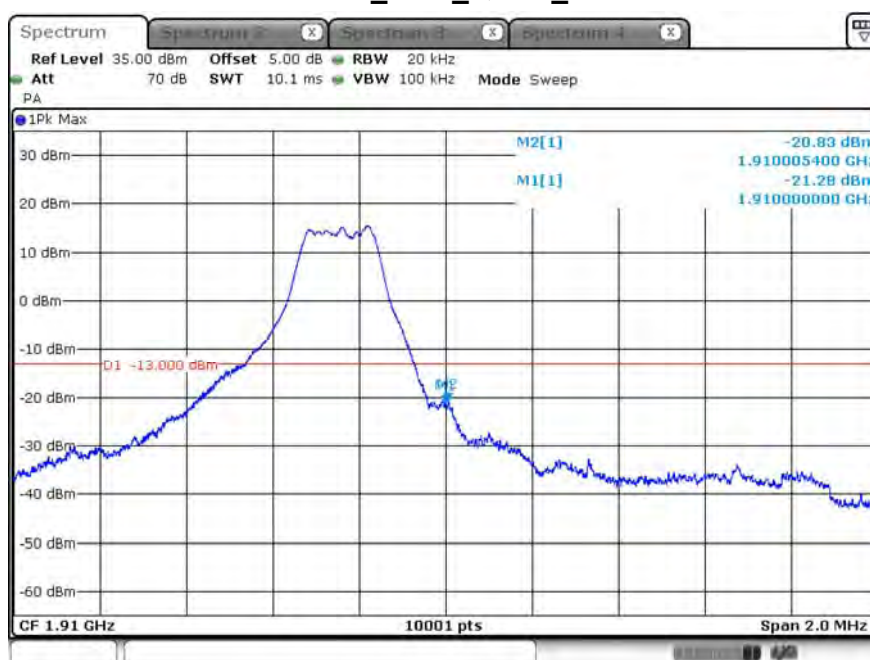
CH19193_1.4M_QPSK_1RB5
