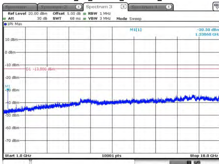
CH133147_5M_16-QAM_Above 1G_1RB12
