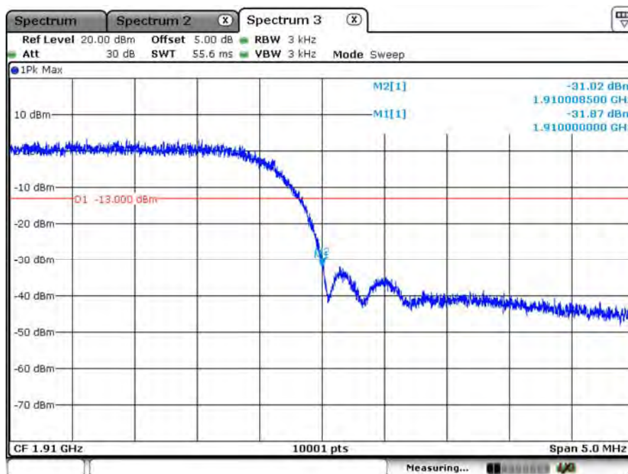
WCDMA_Band 2_RMC_1907.6MHz
