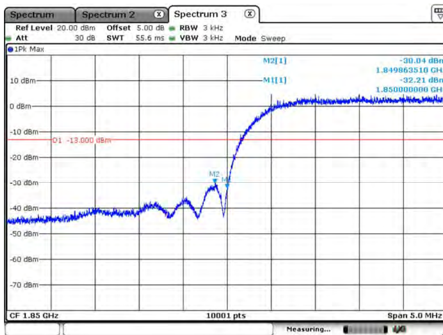
WCDMA_Band 2_RMC_1852.4MHz
