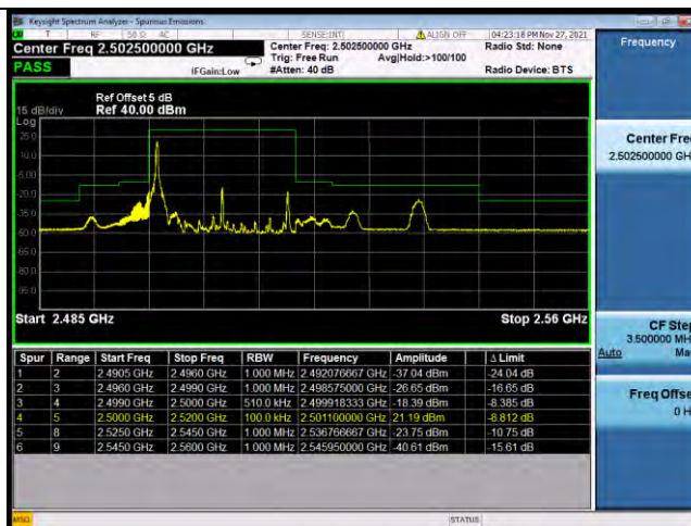
Band7-20MHz-16QAM -20850-27RB#0
