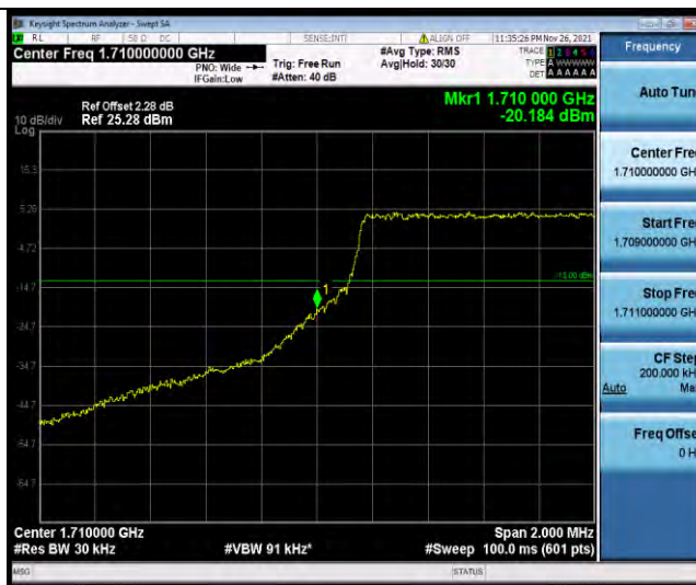
Band4-1.4MHz-16QAM-20393-1RB#5
