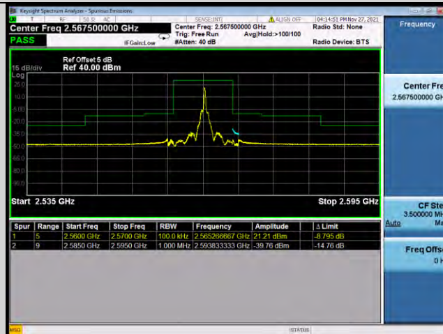
Band7-10MHz-16QAM -21400-27RB#0
