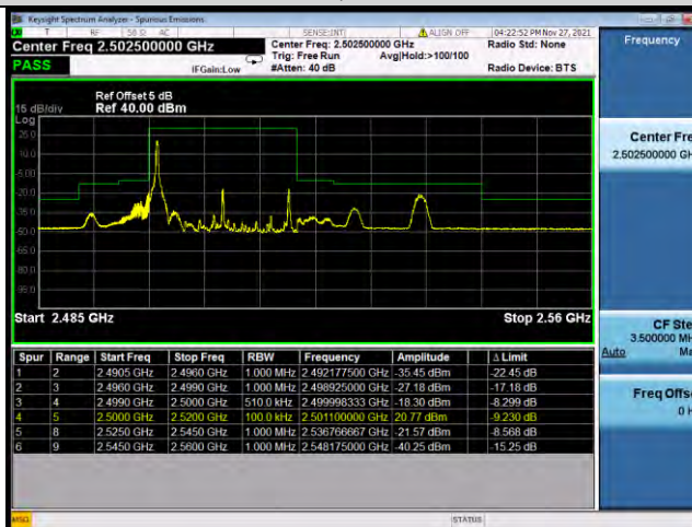
Band7-20MHz-QPSK-20850-100RB#0
