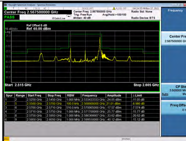
Band7-20MHz-QPSK-21350-100RB#0
