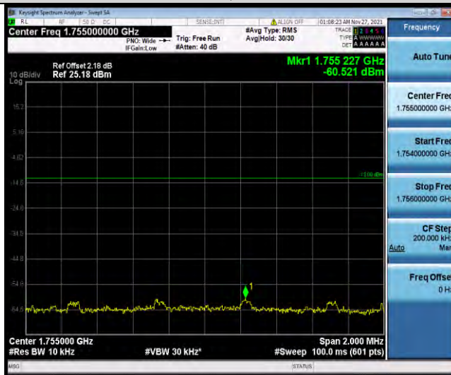
Band4-20MHz-16QAM-20300-27RB#0
