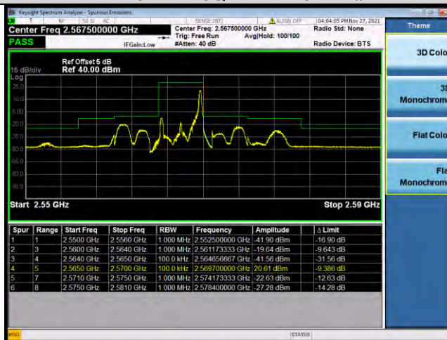
Band7-5MHz-16QAM-21425-25RB#0
