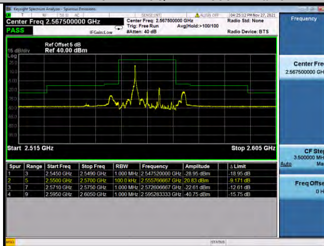
Band7-20MHz-16QAM -21350-27RB#0
