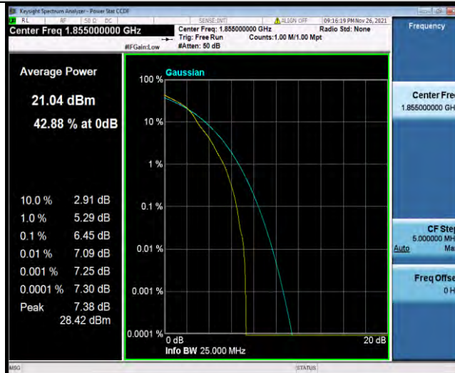
Band2-10MHz-16QAM-18650-27RB#0
