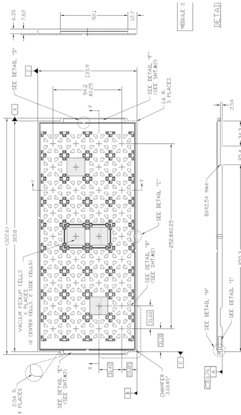
Figure 38: Tray Drawing
