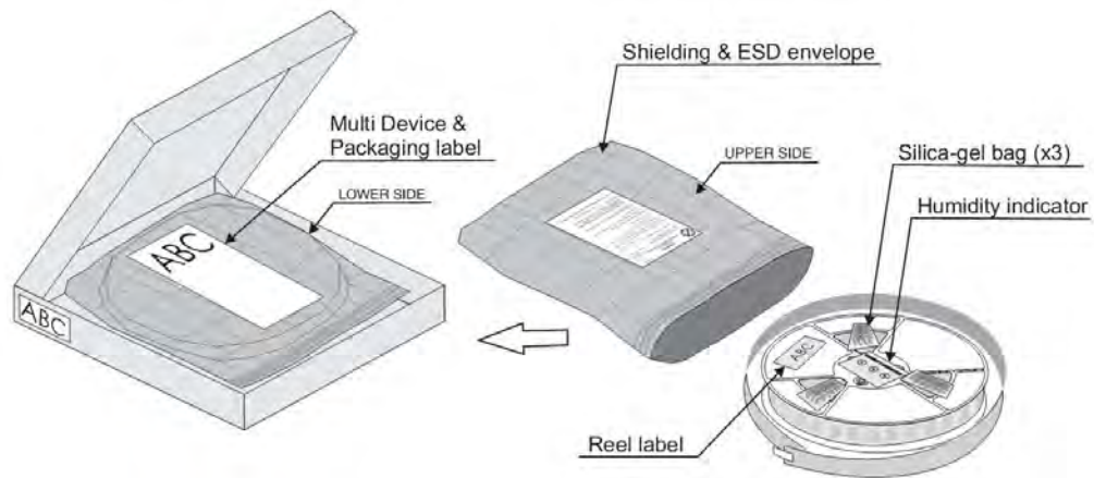
Figure 43: Reel Box Detail
