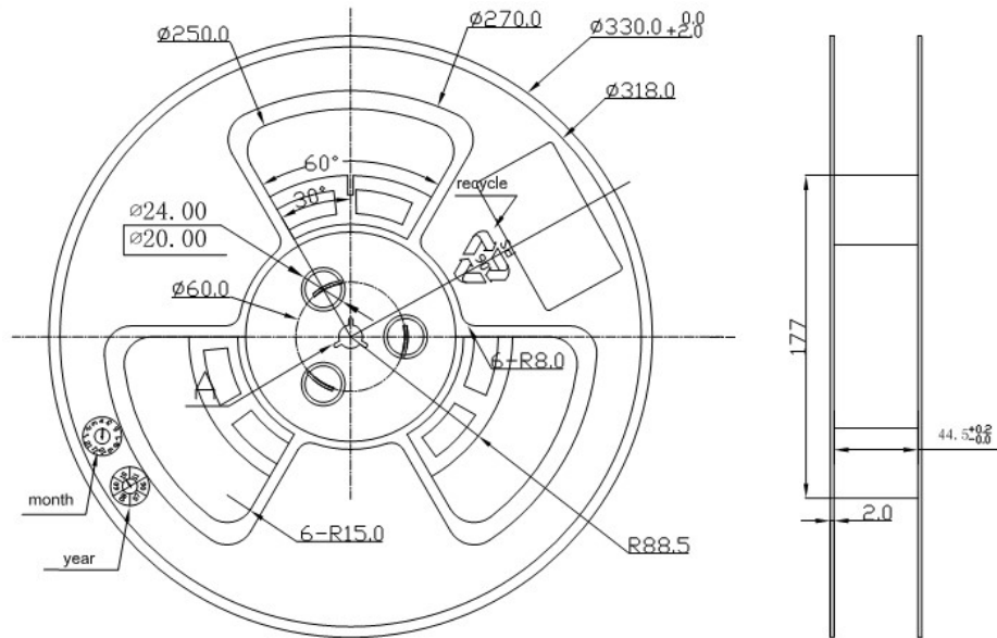
Figure 41: Reel Detail
