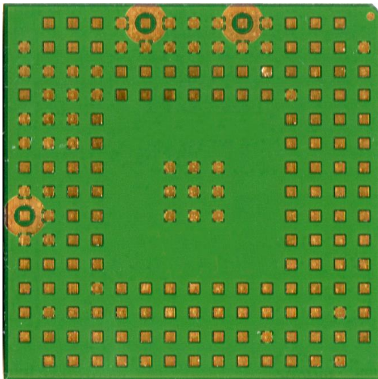
LE910C4-WWX and LE910C1-WWX Bottom
