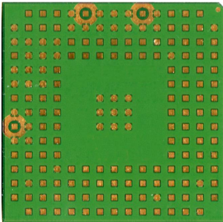
LE910C1-WWX Bottom
