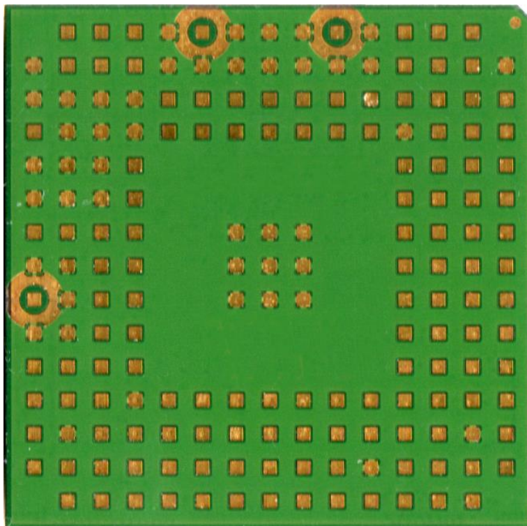
LE910C4-WWX Bottom
