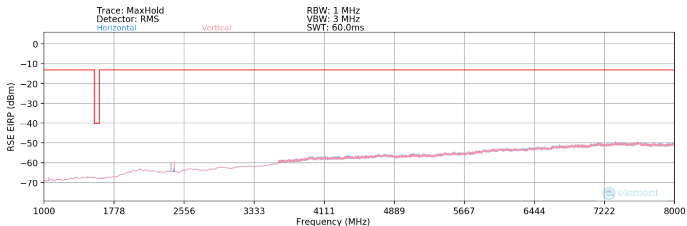
Plot 6-2. Radiated Spurious Plot (LTE Band 14 – Mid Channel – Above 1GHz)
