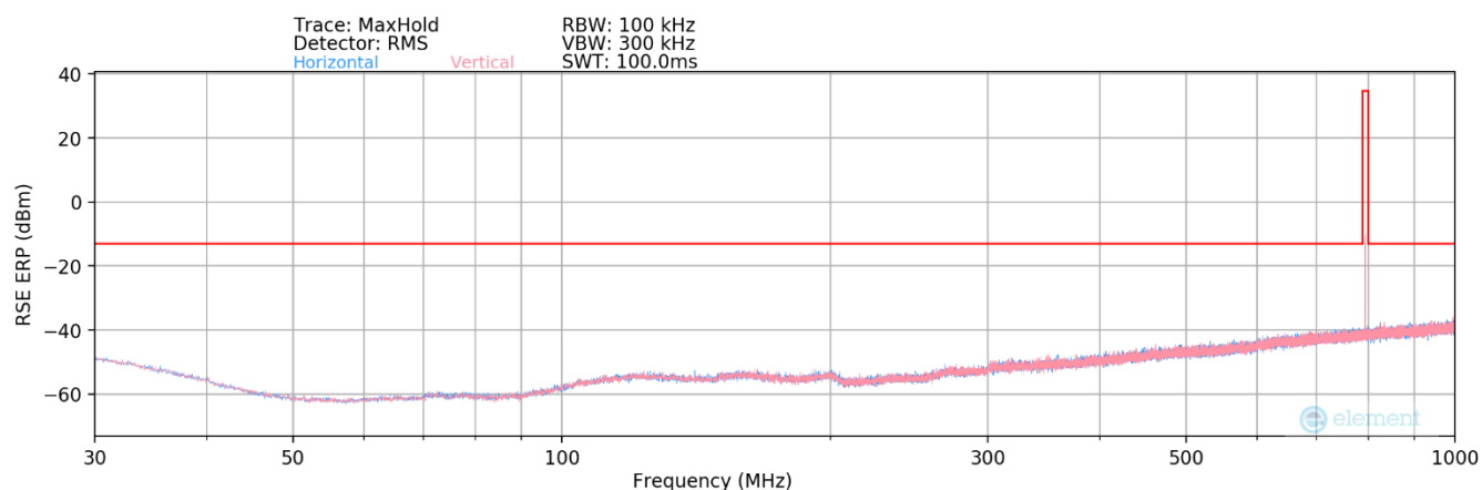
Plot 6-1. Radiated Spurious Plot (LTE Band 14 – Mid Channel – Below 1GHz)
