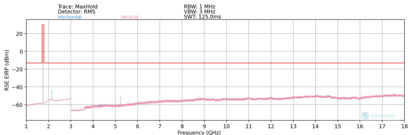
Plot 6-8. Radiated Spurious Plot (LTE Band 66/4 – Mid Channel – Above 1GHz)
