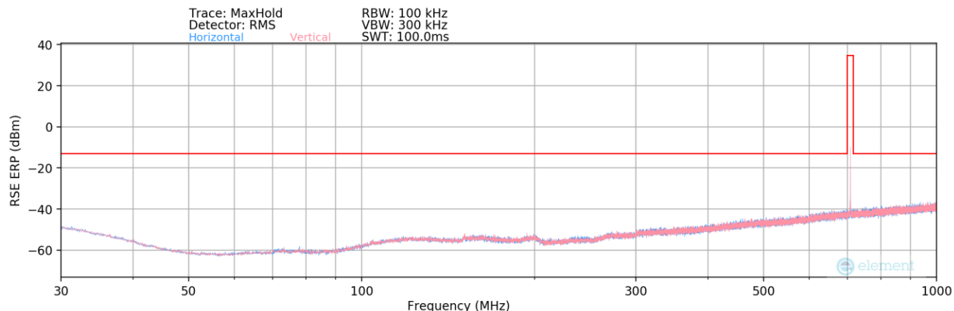
Plot 6-3. Radiated Spurious Plot (LTE Band 12 – Mid Channel – Below 1GHz)
