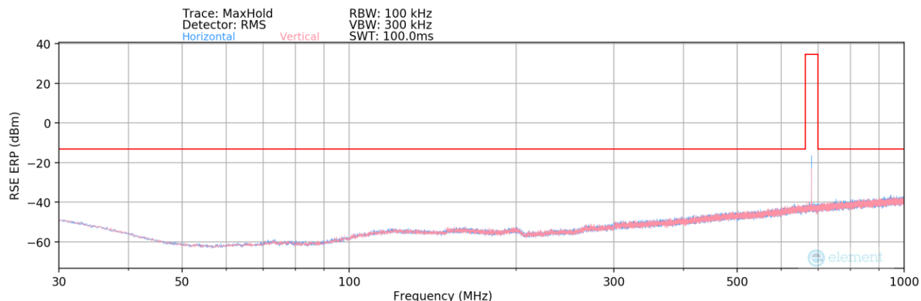
Plot 6-1. Radiated Spurious Plot (LTE Band 71 – Mid Channel – Below 1GHz)
