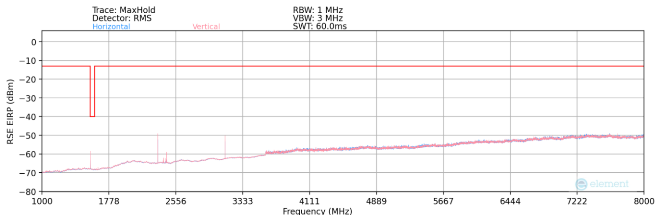
Plot 6-6. Radiated Spurious Plot (LTE Band 13 – Mid Channel – Above 1GHz)
