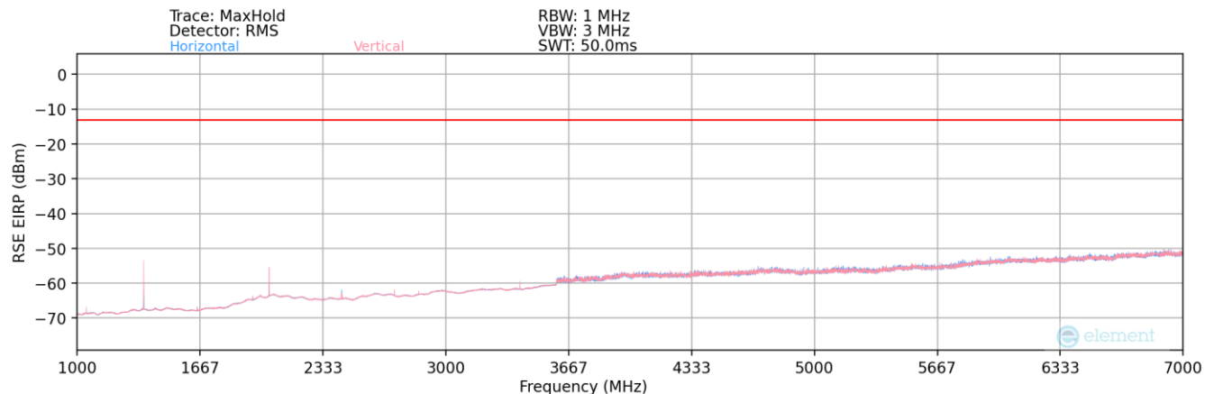
Plot 6-2. Radiated Spurious Plot (LTE Band 71 – Mid Channel – Above 1GHz)
