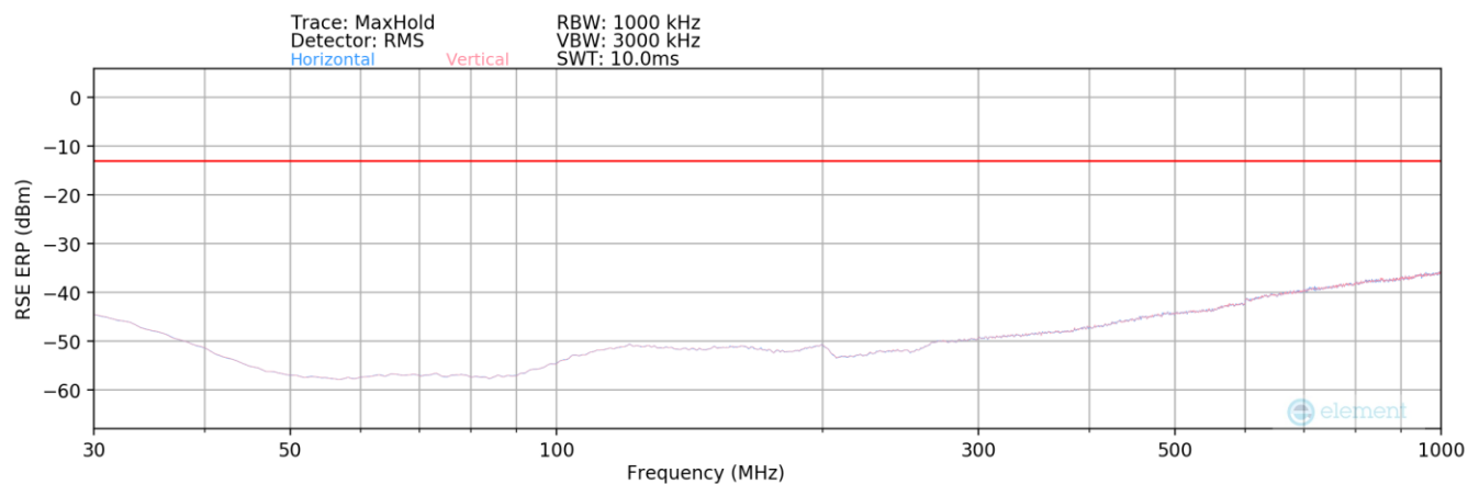
Plot 6-7. Radiated Spurious Plot (LTE Band 66/4 – Mid Channel – Below 1GHz)
