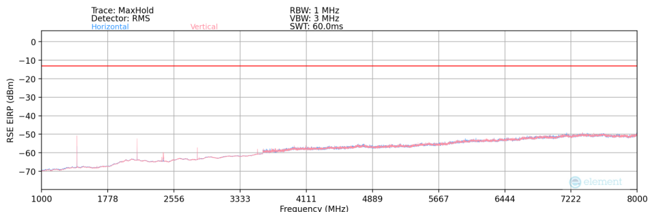
Plot 6-4. Radiated Spurious Plot (LTE Band 12 – Mid Channel – Above 1GHz)
