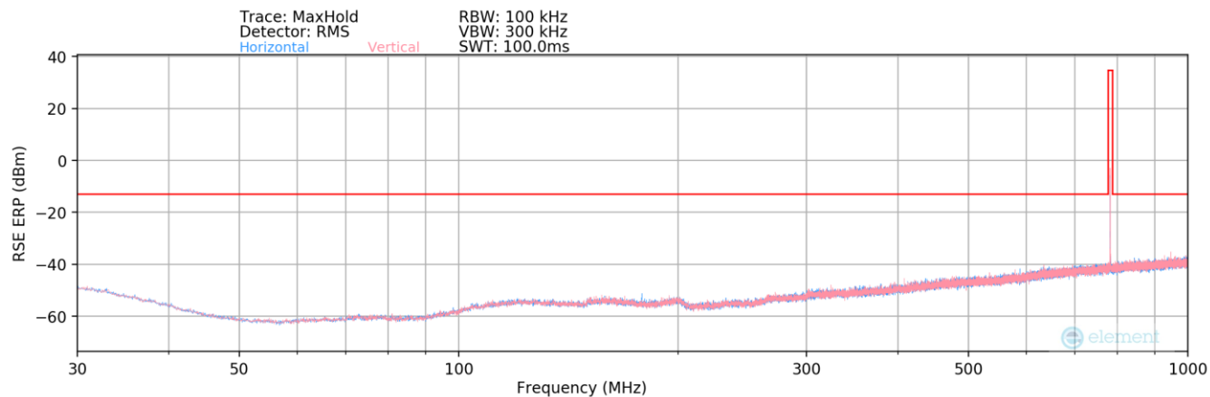
Plot 6-5. Radiated Spurious Plot (LTE Band 13 – Mid Channel – Below 1GHz)
