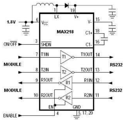
Figure 16: RS232 Level Adaption Circuitry Example
