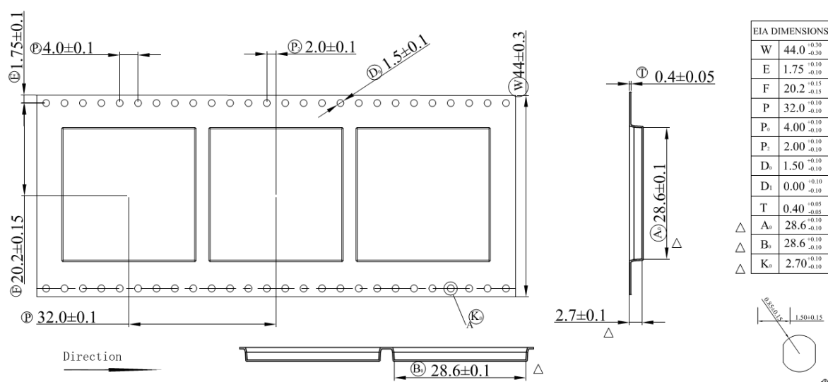
Figure 43: Carrier Tape Detail
