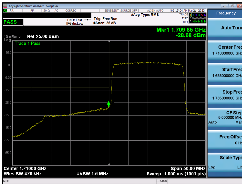
Plot 7-62. Lower Band Edge Plot (LTE Band 66/4 - 20MHz QPSK – Full RB)
