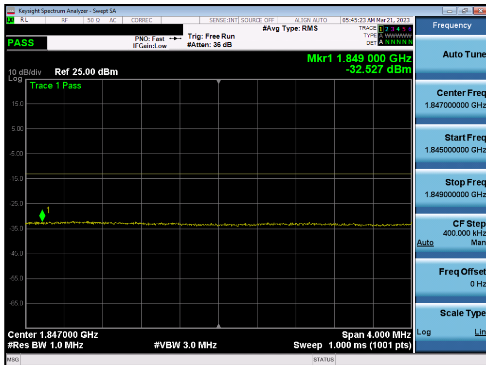
Plot 7-27. Extended Lower Band Edge Plot (LTE Band 2 - 15MHz QPSK – Full RB)
