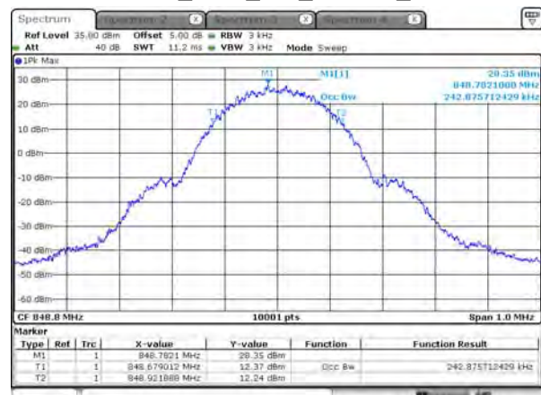
99% BW_GSM_850_EGPRS_848.8
