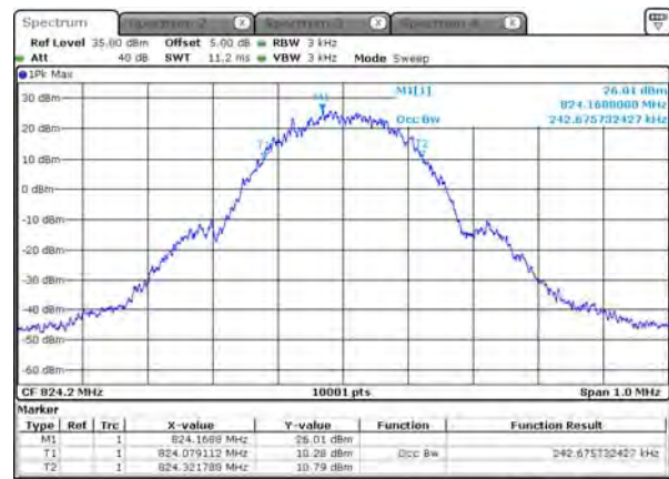
99% BW_GSM_850_EGPRS_824.2
