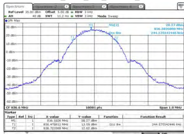
99% BW_GSM_850_EGPRS_836.6
