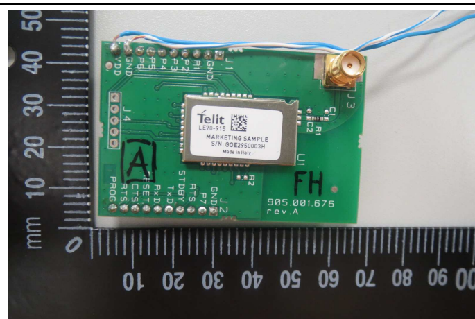
Front view of module
