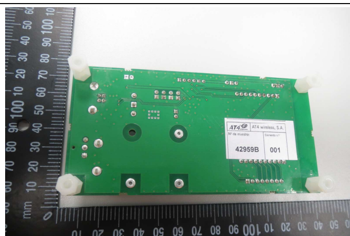
Rear view of test board
