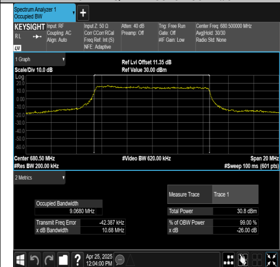
Band71-10MHz-16QAM-133172-27RB#0-PASS
