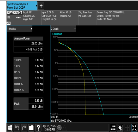
Band71-20MHz-16QAM-133322-27RB#0-PASS
