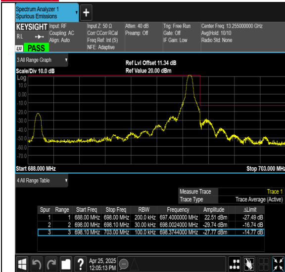
Band71-10MHz-16QAM-133172-1RB#0-PASS
