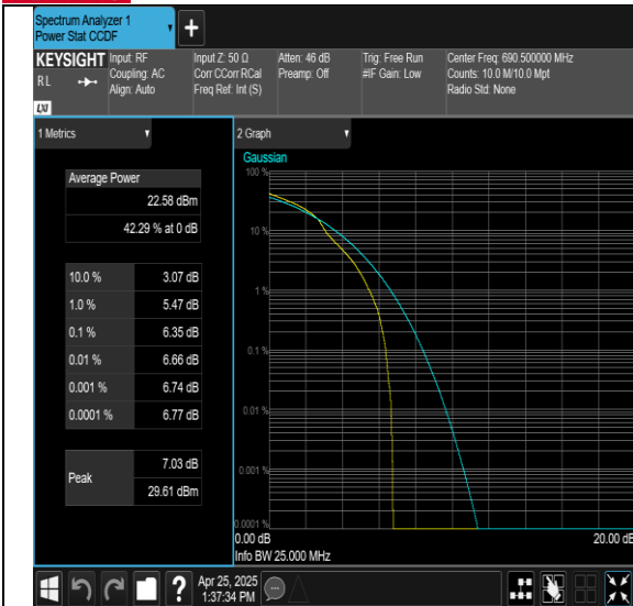
Band71-20MHz-QPSK-133222-1RB#0-PASS
