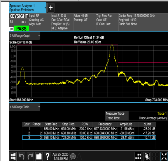
Band71-15MHz-QPSK-133197-1RB#0-PASS
