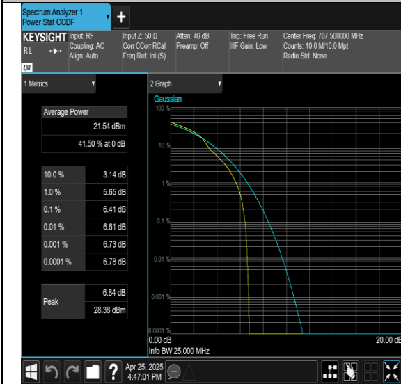
Band12-3MHz-16QAM-23165-1RB#0-PASS
