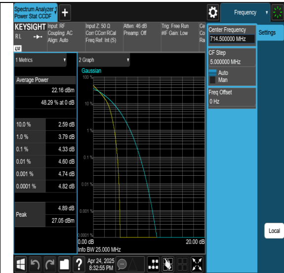
Band12-3MHz-16QAM-23025-15RB#0-PASS
