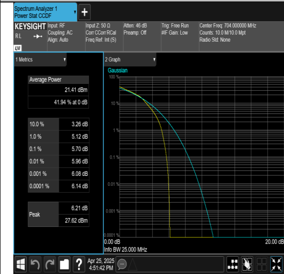
Band12-10MHz-16QAM-23095-27RB#0-PASS
