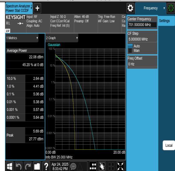
Band12-5MHz-QPSK-23095-25RB#0-PASS
