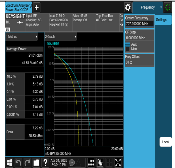
Band12-3MHz-QPSK-23165-15RB#0-PASS
