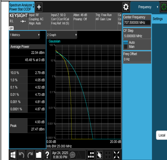
Band12-10MHz-QPSK-23130-1RB#0-PASS
