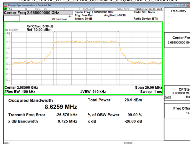
Band41_10MHz_DFT_s_OFDM_SCS30kHz_64QAM_RB24_0_CH537000
