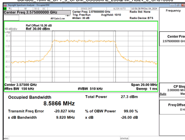
Band38_10MHz_DFT_s_OFDM_SCS30kHz_256QAM_RB24_0_CH515000
