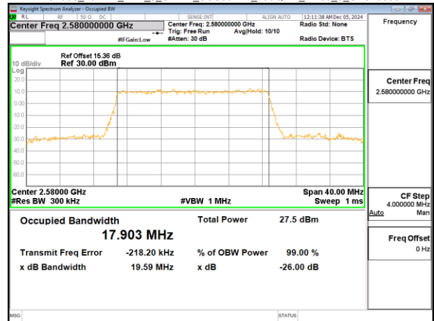
Band38_20MHz_DFT_s_OFDM_SCS30kHz_256QAM_RB50_0_CH516000
