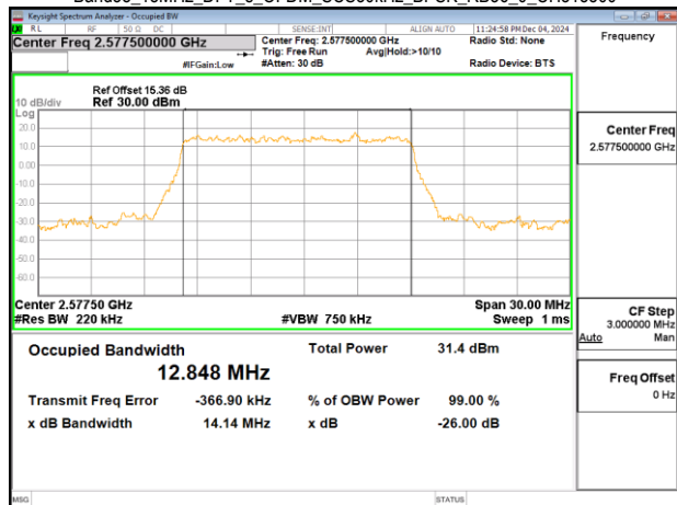
Band38_15MHz_DFT_s_OFDM_SCS30kHz_BPSK_RB36_0_CH515500
