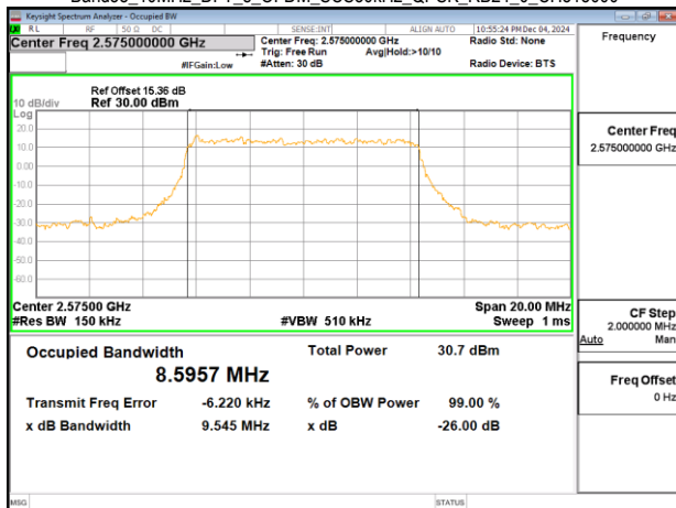
Band38_10MHz_DFT_s_OFDM_SCS30kHz_QPSK_RB24_0_CH515000
