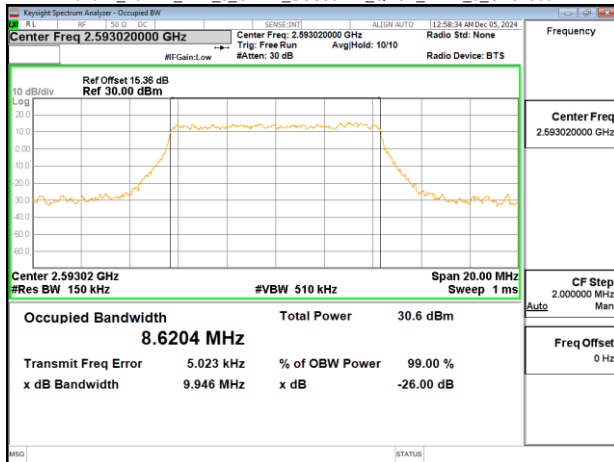
Band41_10MHz_DFT_s_OFDM_SCS30kHz_QPSK_RB24_0_CH518604
