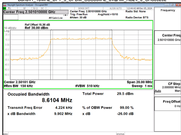
Band41_10MHz_DFT_s_OFDM_SCS30kHz_64QAM_RB24_0_CH500202
