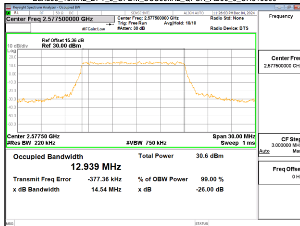
Band38_15MHz_DFT_s_OFDM_SCS30kHz_QPSK_RB36_0_CH515500
