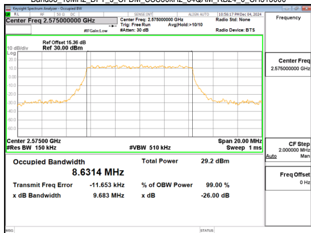
Band38_10MHz_DFT_s_OFDM_SCS30kHz_64QAM_RB24_0_CH515000
