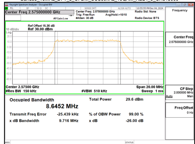
Band38_10MHz_DFT_s_OFDM_SCS30kHz_16QAM_RB24_0_CH515000
