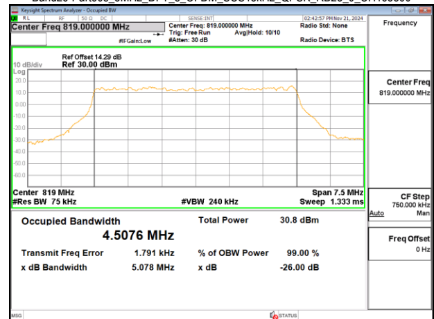
Band26-Part90s_5MHz_DFT_s_OFDM_SCS15kHz_QPSK_RB25_0_CH163800
