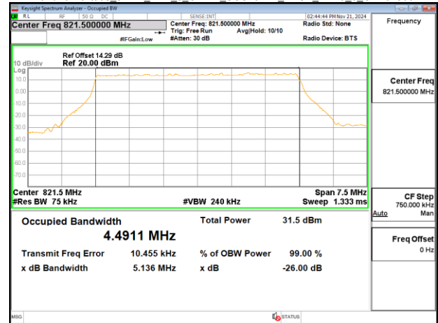
Band26-Part90s_5MHz_DFT_s_OFDM_SCS15kHz_QPSK_RB25_0_CH163300
