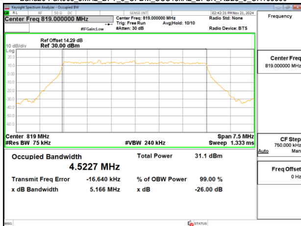
Band26-Part90s_5MHz_DFT_s_OFDM_SCS15kHz_BPSK_RB25_0_CH163800
