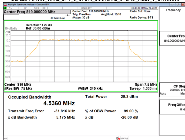
Band26-Part90s_5MHz_DFT_s_OFDM_SCS15kHz_64QAM_RB25_0_CH163800
