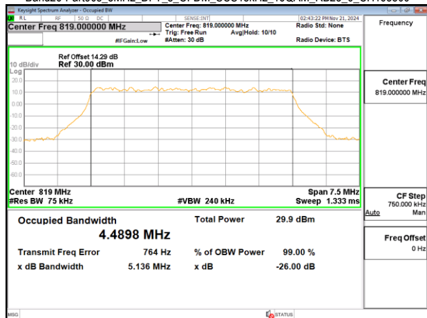
Band26-Part90s_5MHz_DFT_s_OFDM_SCS15kHz_16QAM_RB25_0_CH163800
