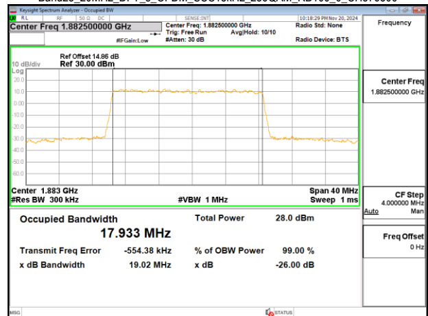
Band25_20MHz_DFT_s_OFDM_SCS15kHz_256QAM_RB100_0_CH376500
