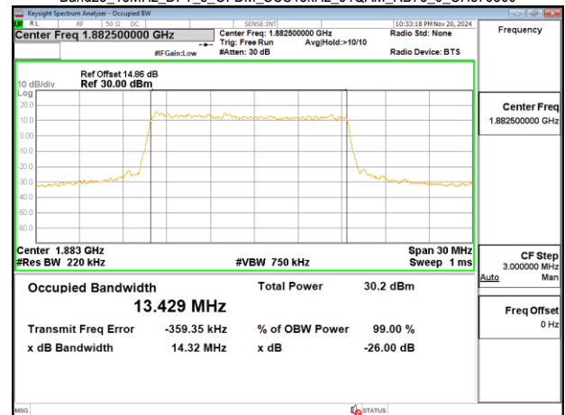
Band25_15MHz_DFT_s_OFDM_SCS15kHz_64QAM_RB75_0_CH376500
