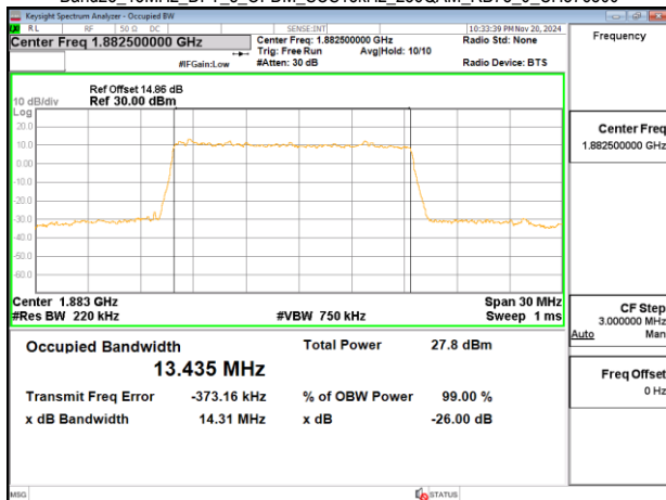
Band25_15MHz_DFT_s_OFDM_SCS15kHz_256QAM_RB75_0_CH376500
