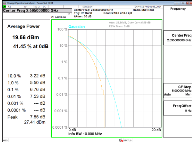
Band38_10MHz_DFT_s_OFDM_SCS30kHz_256QAM_RB24_0_CH519000
