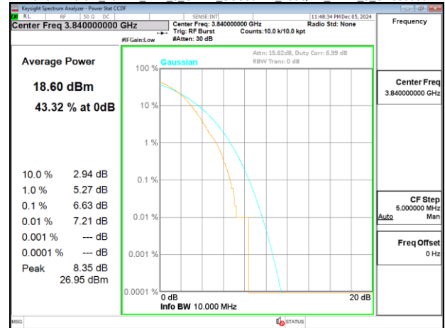
Band77-Part27_10MHz_DFT_s_OFDM_SCS30kHz_256QAM_RB24_0_CH656000
