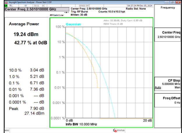
Band41_10MHz_DFT_s_OFDM_SCS30kHz_256QAM_RB24_0_CH501000
