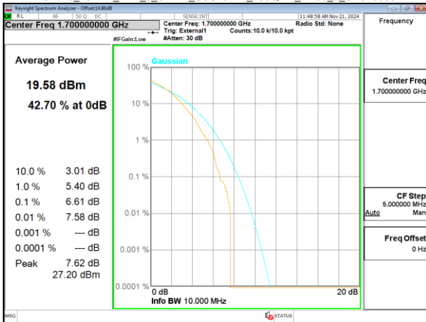
Band70_10MHz_DFT_s_OFDM_SCS15kHz_256QAM_RB50_0_CH340500
