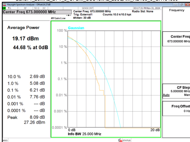
Band71_20MHz_DFT_s_OFDM_SCS15kHz_256QAM_RB100_0_CH134600
