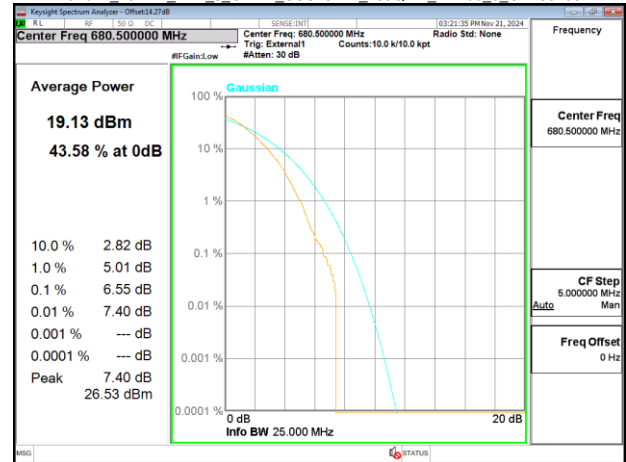
Band71_20MHz_DFT_s_OFDM_SCS15kHz_256QAM_RB100_0_CH137600
