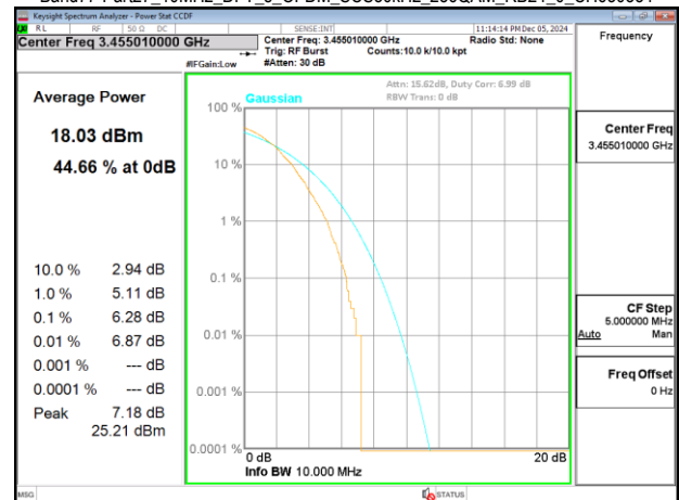
Band77-Part27_10MHz_DFT_s_OFDM_SCS30kHz_256QAM_RB24_0_CH630334
