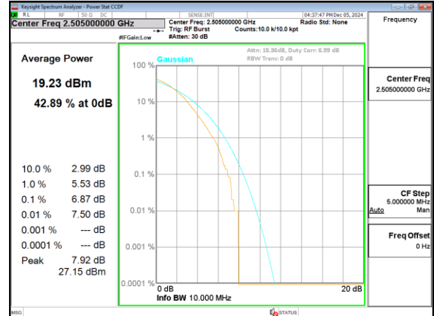
Band41_10MHz_DFT_s_OFDM_SCS30kHz_256QAM_RB24_0_CH501000
