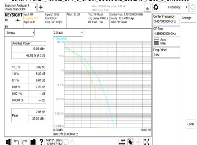
Band77-Part27_15MHz_DFT_s_OFDM_SCS30kHz_256QAM_RB36_0_CH630500
