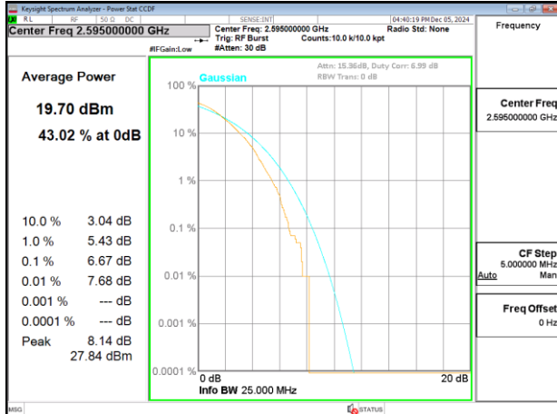
Band38_20MHz_DFT_s_OFDM_SCS30kHz_256QAM_RB50_0_CH519000
