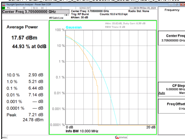
Band77-Part27_10MHz_DFT_s_OFDM_SCS30kHz_256QAM_RB24_0_CH647000
