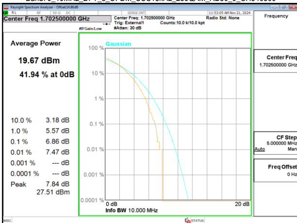
Band70_10MHz_DFT_s_OFDM_SCS15kHz_256QAM_RB50_0_CH340500
