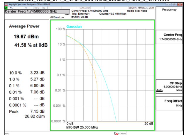
Band66_15MHz_DFT_s_OFDM_SCS15kHz_256QAM_RB75_0_CH349000
