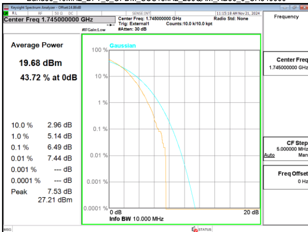
Band66_10MHz_DFT_s_OFDM_SCS15kHz_256QAM_RB50_0_CH349000
