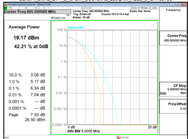
Band71_5MHz_DFT_s_OFDM_SCS15kHz_256QAM_RB25_0_CH133100
