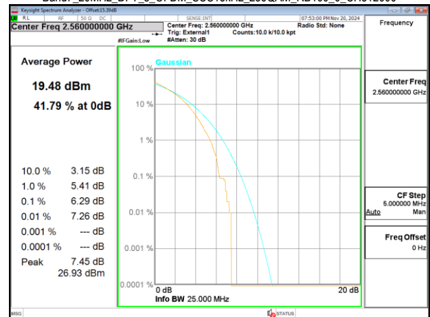
Band7_20MHz_DFT_s_OFDM_SCS15kHz_256QAM_RB100_0_CH512000
