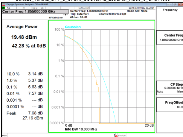
Band25_10MHz_DFT_s_OFDM_SCS15kHz_256QAM_RB50_0_CH371000
