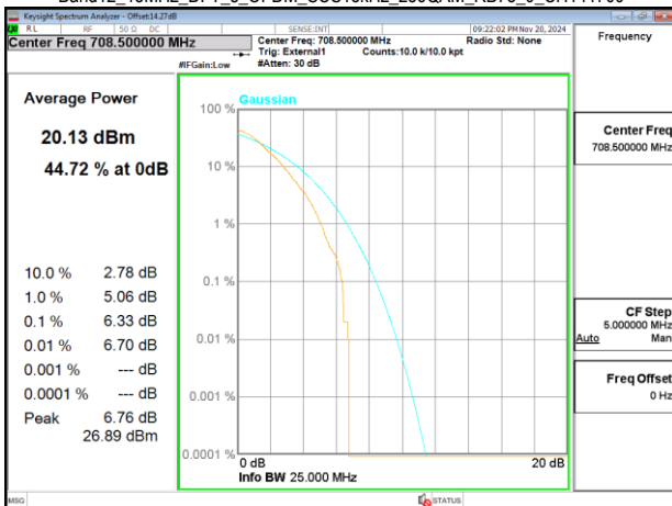
Band12_15MHz_DFT_s_OFDM_SCS15kHz_256QAM_RB75_0_CH141700
