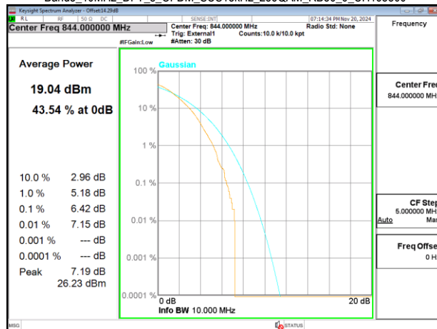
Band5_10MHz_DFT_s_OFDM_SCS15kHz_256QAM_RB50_0_CH168800
