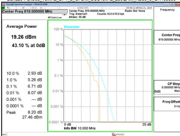
Band26-Part90s_10MHz_DFT_s_OFDM_SCS15kHz_256QAM_RB50_0_CH163800
