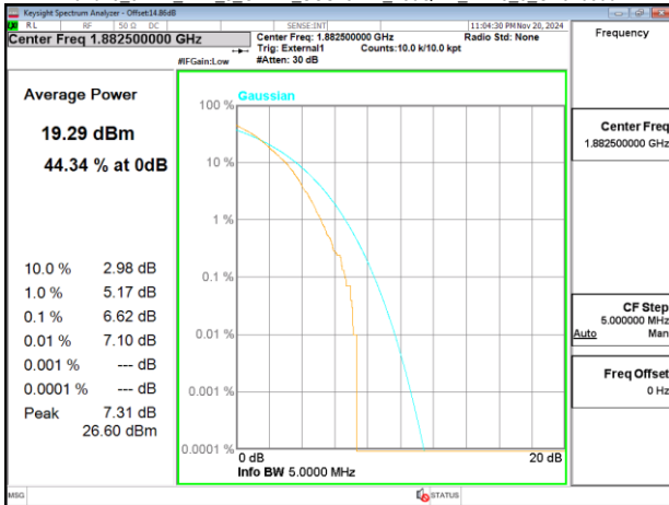
Band25_5MHz_DFT_s_OFDM_SCS15kHz_256QAM_RB25_0_CH382500
