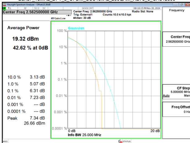
Band7_15MHz_DFT_s_OFDM_SCS15kHz_256QAM_RB75_0_CH512500
