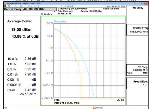
Band26_5MHz_DFT_s_OFDM_SCS15kHz_256QAM_RB25_0_CH169300
