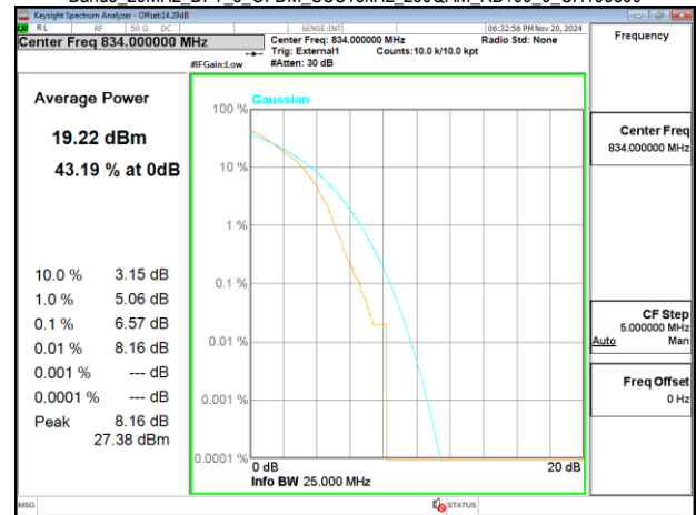
Band5_20MHz_DFT_s_OFDM_SCS15kHz_256QAM_RB100_0_CH167800
