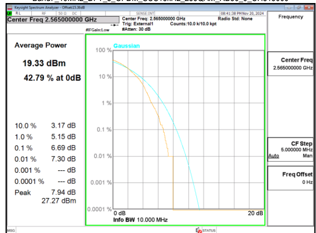
Band7_10MHz_DFT_s_OFDM_SCS15kHz_256QAM_RB50_0_CH513000
