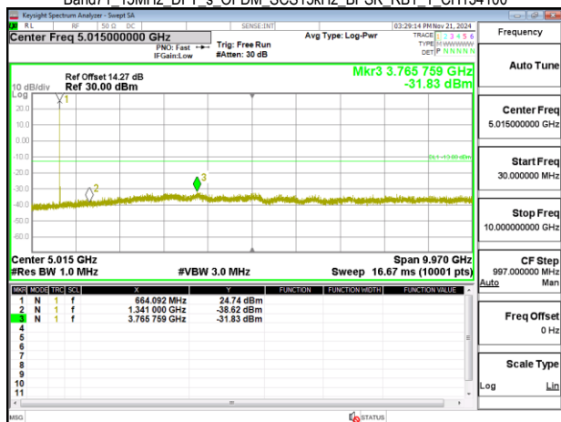
Band71_15MHz_DFT_s_OFDM_SCS15kHz_BPSK_RB1_1_CH136100
