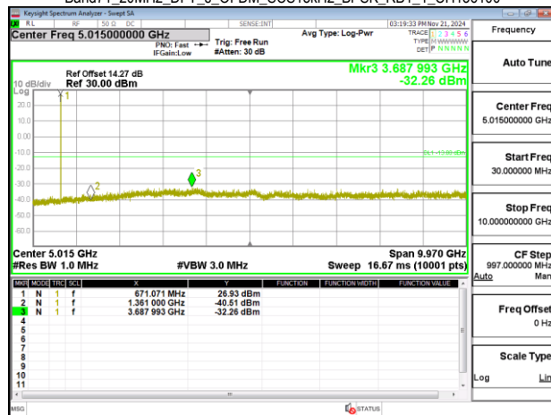
Band71_20MHz_DFT_s_OFDM_SCS15kHz_BPSK_RB1_1_CH138700
