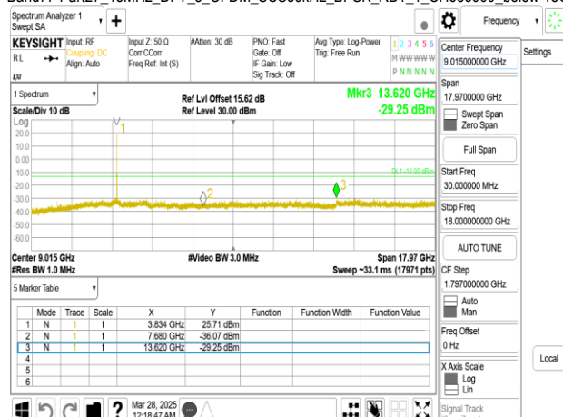
Band77-Part27_15MHz_DFT_s_OFDM_SCS30kHz_BPSK_RB1_1_CH656000_below 18G
