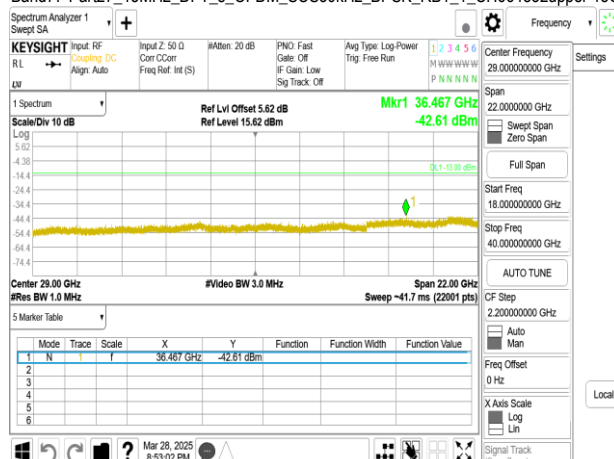
Band77-Part27_15MHz_DFT_s_OFDM_SCS30kHz_BPSK_RB1_1_CH664832upper 18G
