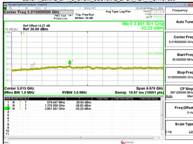
Band71_20MHz_DFT_s_OFDM_SCS15kHz_BPSK_RB1_1_CH138700
