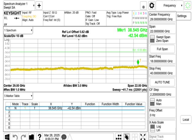
Band77-Part27_20MHz_DFT_s_OFDM_SCS30kHz_BPSK_RB1_1_CH664666upper 18G
