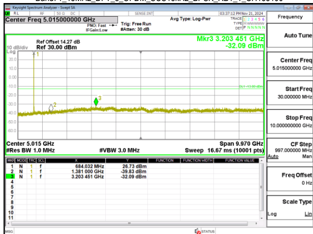
Band71_15MHz_DFT_s_OFDM_SCS15kHz_BPSK_RB1_1_CH138100
