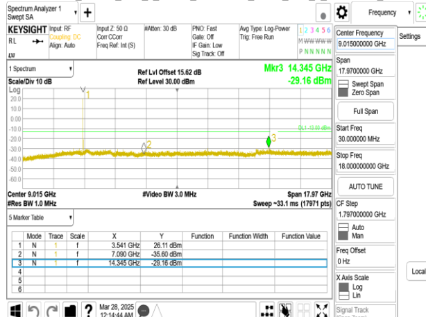
Band77-Part27_10MHz_DFT_s_OFDM_SCS30kHz_BPSK_RB1_1_CH636332upper 18G
