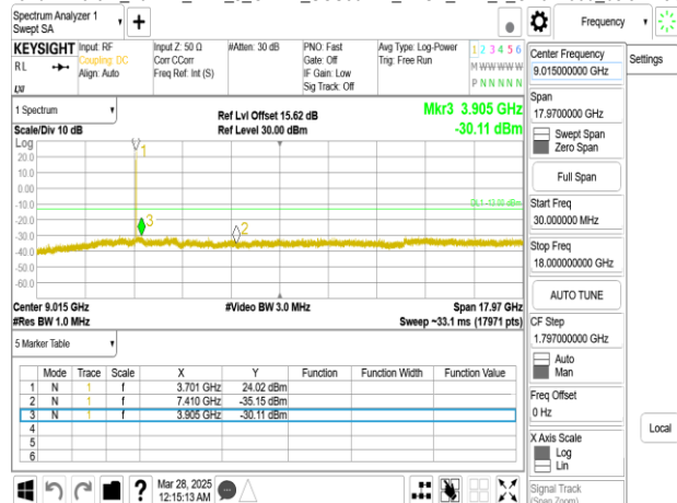
Band77-Part27_10MHz_DFT_s_OFDM_SCS30kHz_BPSK_RB1_1_CH647000upper 18G
