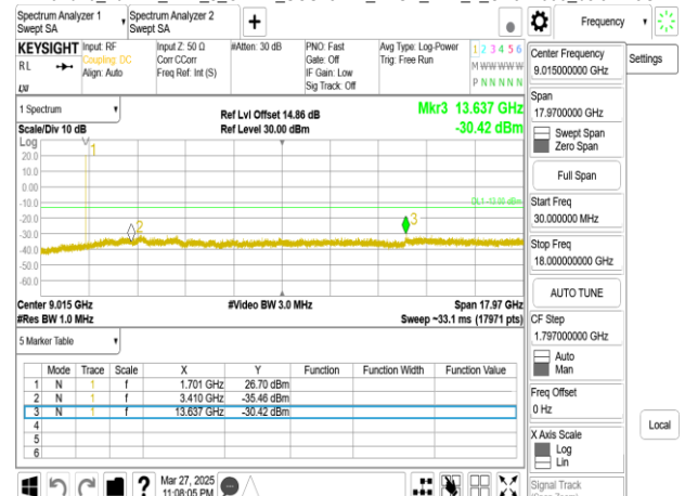
Band70_15MHz_DFT_s_OFDM_SCS15kHz_BPSK_RB1_1_CH340500_below 18G
