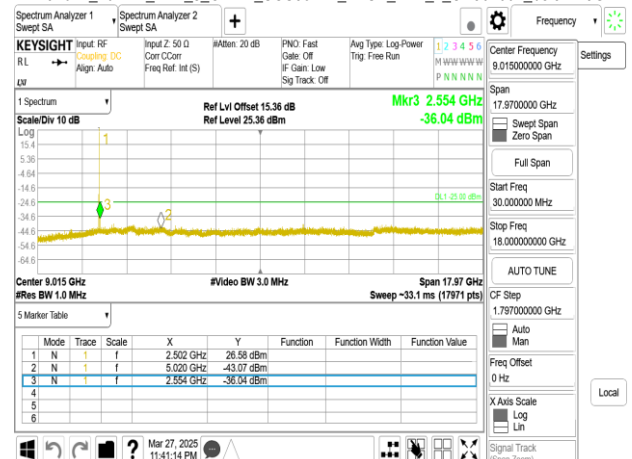
Band41_20MHz_DFT_s_OFDM_SCS30kHz_BPSK_RB1_1_CH502002_below 18G
