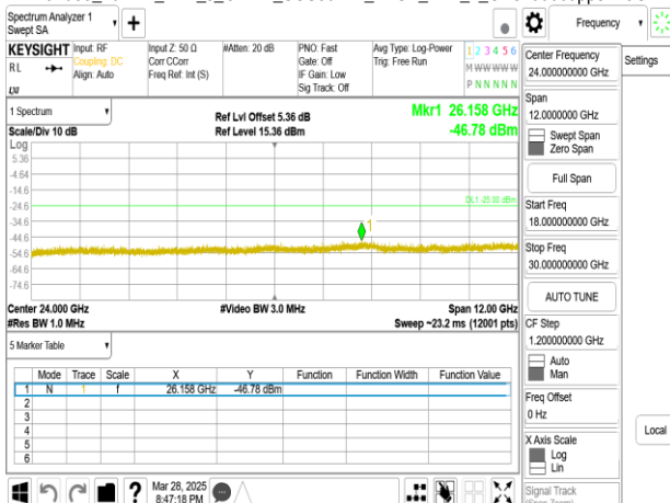
Band38_20MHz_DFT_s_OFDM_SCS30kHz_BPSK_RB1_1_CH519000upper 18G
