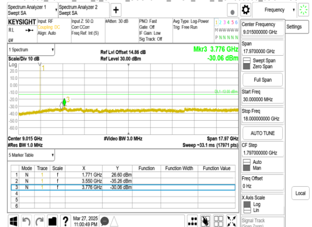
Band66_15MHz_DFT_s_OFDM_SCS15kHz_BPSK_RB1_1_CH343500_below 18G
