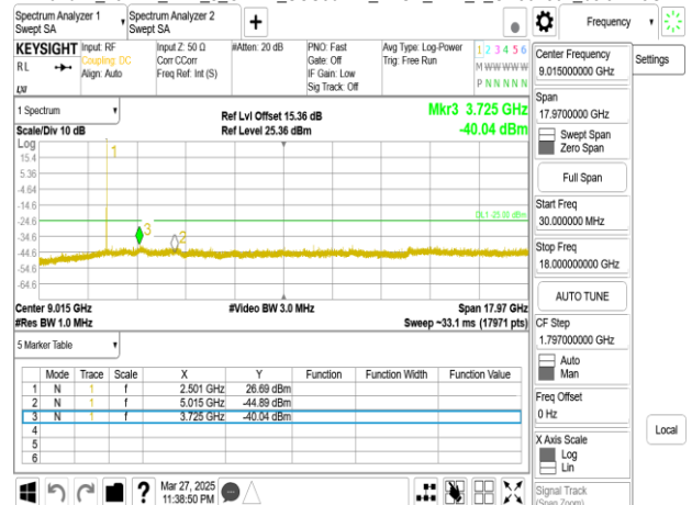
Band41_15MHz_DFT_s_OFDM_SCS30kHz_BPSK_RB1_1_CH501504upper 18G
