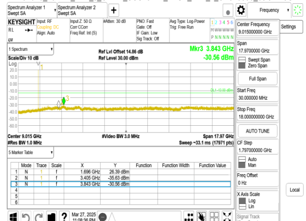
Band70_15MHz_DFT_s_OFDM_SCS15kHz_BPSK_RB1_1_CH340500_below 18G
