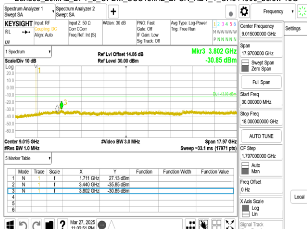
Band66_20MHz_DFT_s_OFDM_SCS15kHz_BPSK_RB1_1_CH344000_below 18G
