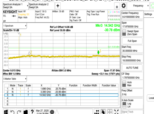
Band70_5MHz_DFT_s_OFDM_SCS15kHz_BPSK_RB1_1_CH339500_below 18G
