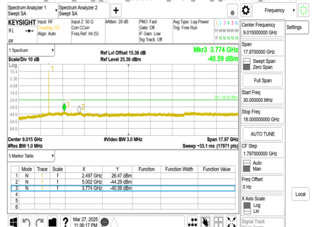
Band41_10MHz_DFT_s_OFDM_SCS30kHz_BPSK_RB1_1_CH500202 below 18G
