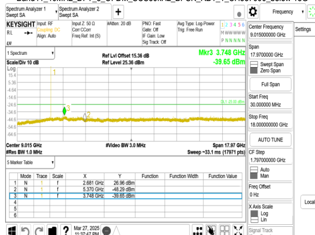
Band41_10MHz_DFT_s_OFDM_SCS30kHz_BPSK_RB1_1_CH537000_below 18G
