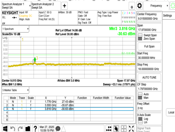
Band66_10MHz_DFT_s_OFDM_SCS15kHz_BPSK_RB1_1_CH343000_below 18G
