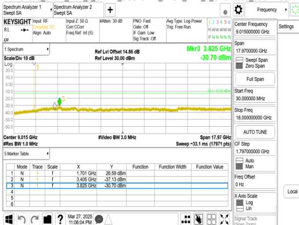
Band70_5MHz_DFT_s_OFDM_SCS15kHz_BPSK_RB1_1_CH341500_below 18G
