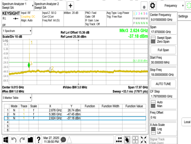
Band41_15MHz_DFT_s_OFDM_SCS30kHz_BPSK_RB1_1_CH536496upper 18G
