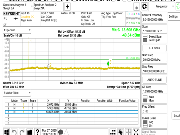
Band41_20MHz_DFT_s_OFDM_SCS30kHz_BPSK_RB1_1_CH535998upper 18G
