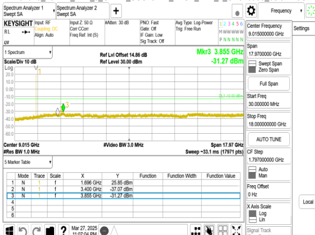
Band70_10MHz_DFT_s_OFDM_SCS15kHz_BPSK_RB1_1_CH340000_below 18G
