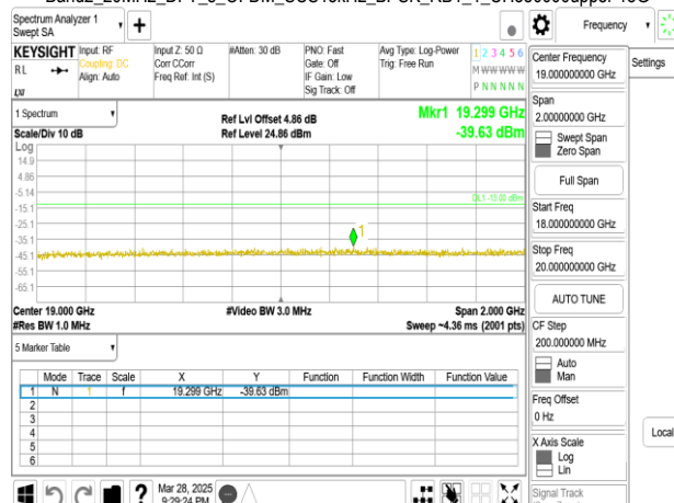
Band2_20MHz_DFT_s_OFDM_SCS15kHz_BPSK_RB1_1_CH380000upper 18G
