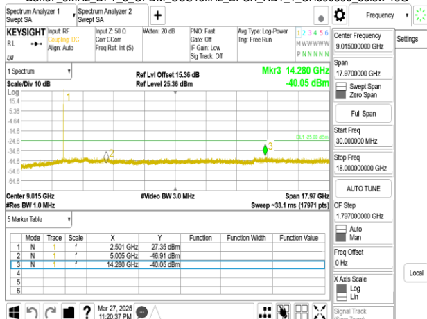
Band7_5MHz_DFT_s_OFDM_SCS15kHz_BPSK_RB1_1_CH500500upper 18G
