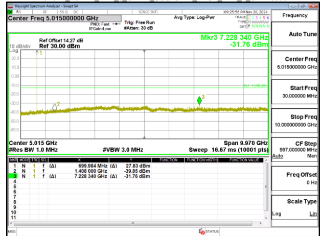
Band12_10MHz_DFT_s_OFDM_SCS15kHz_BPSK_RB1_1_CH141500
