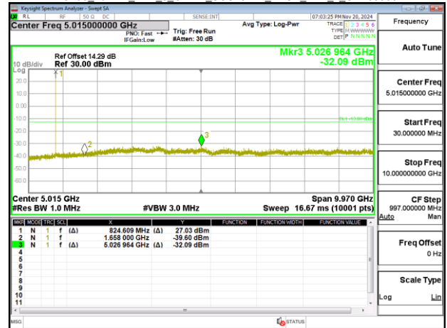
Band5_10MHz_DFT_s_OFDM_SCS15kHz_BPSK_RB1_1_CH167300
