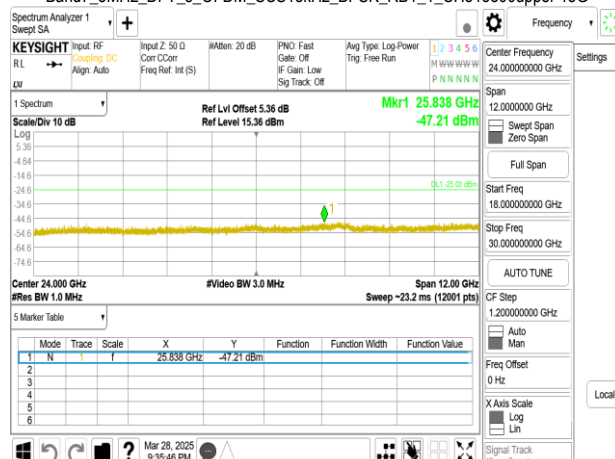
Band7_5MHz_DFT_s_OFDM_SCS15kHz_BPSK_RB1_1_CH513500upper 18G
