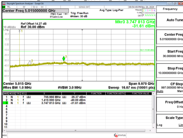
Band12_5MHz_DFT_s_OFDM_SCS15kHz_BPSK_RB1_1_CH142700
