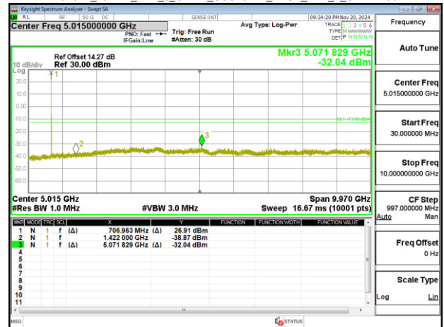
Band12_10MHz_DFT_s_OFDM_SCS15kHz_BPSK_RB1_1_CH142200
