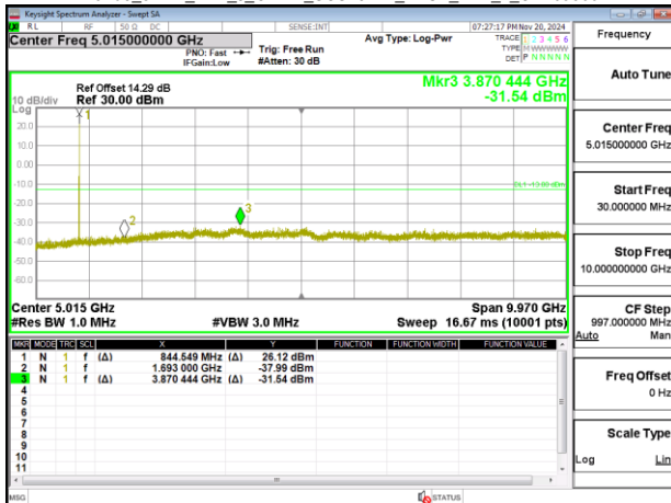
Band5_5MHz_DFT_s_OFDM_SCS15kHz_BPSK_RB1_1_CH169300
