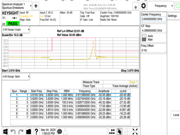
Band77-Part27_20MHz_CP_OFDM_SCS30kHz_QPSK_RB51_0_CH6566000
