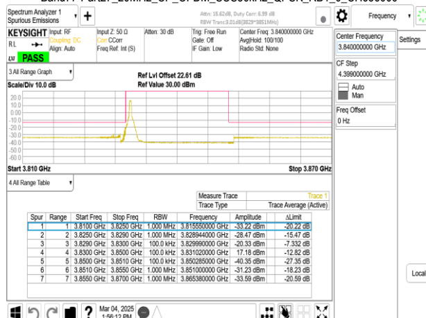
Band77-Part27_20MHz_CP_OFDM_SCS30kHz_QPSK_RB1_0_CH656000
