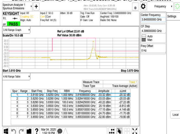
Band77-Part27_20MHz_DFT_s_OFDM_SCS30kHz_BPSK_RB50_0_CH656000
