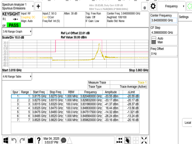
Band77-Part27_15MHz_CP_OFDM_SCS30kHz_QPSK_RB38_0_CH656000
