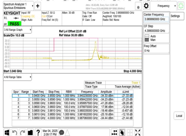
Band77-Part27_20MHz_CP_OFDM_SCS30kHz_QPSK_RB51_0_CH664666
