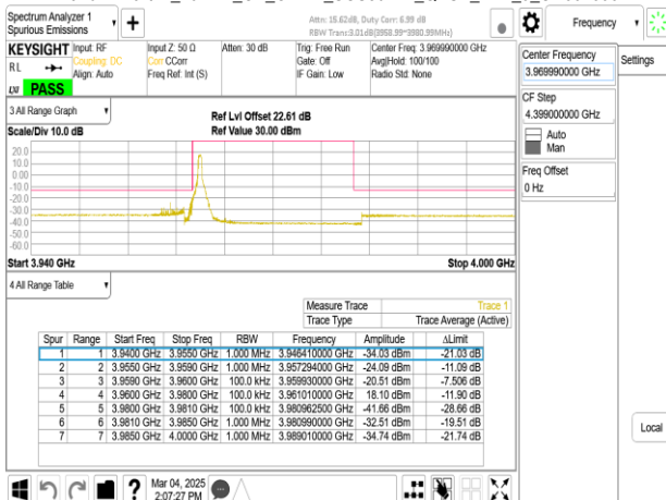
Band77-Part27_20MHz_CP_OFDM_SCS30kHz_QPSK_RB1_0_CH664666
