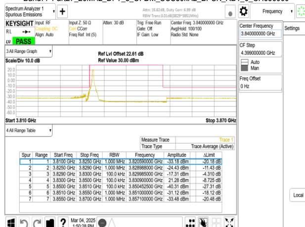
Band77-Part27_20MHz_DFT_s_OFDM_SCS30kHz_BPSK_RB1_0_CH656000
