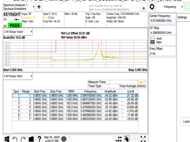
Band77-Part27_15MHz_DFT_s_OFDM_SCS30kHz_BPSK_RB36_0_CH664832
