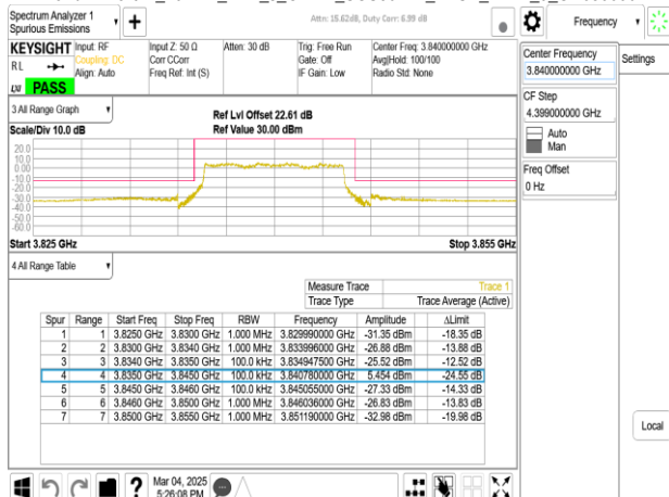
Band77-Part27_10MHz_DFT_s_OFDM_SCS30kHz_BPSK_RB1_0_CH656000
