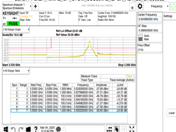
Band77-Part27_10MHz_CP_OFDM_SCS30kHz_QPSK_RB24_0_CH636332
