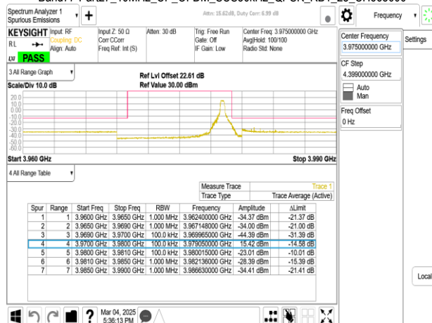
Band77-Part27_10MHz_CP_OFDM_SCS30kHz_QPSK_RB24_0_CH665000
