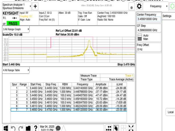
Band77-Part27_10MHz_CP_OFDM_SCS30kHz_QPSK_RB24_0_CH630334
