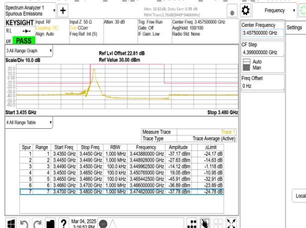
Band77-Part27_15MHz_DFT_s_OFDM_SCS30kHz_BPSK_RB1_0_CH630500
