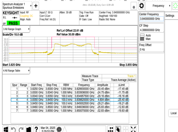
Band77-Part27_10MHz_CP_OFDM_SCS30kHz_QPSK_RB1_0_CH656000
