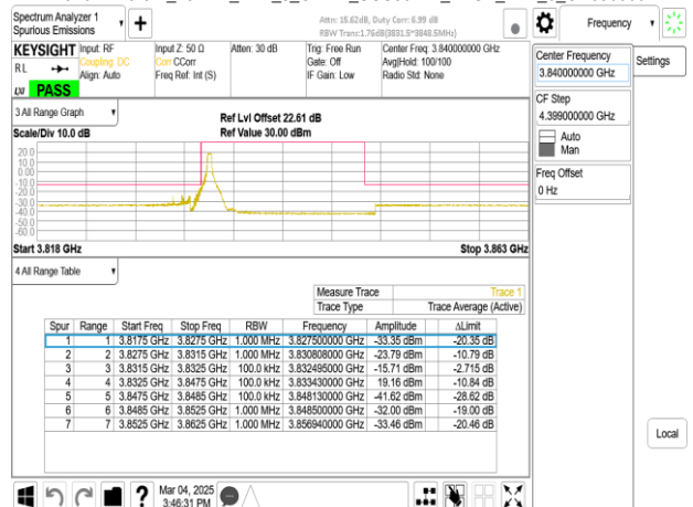
Band77-Part27_15MHz_DFT_s_OFDM_SCS30kHz_BPSK_RB1_0_CH656000
