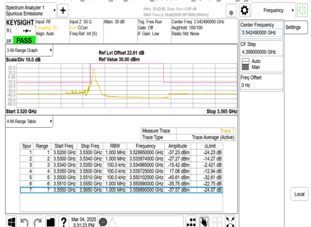
Band77-Part27_15MHz_CP_OFDM_SCS30kHz_QPSK_RB1_0_CH636166
