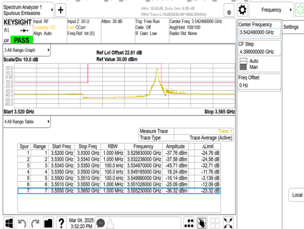
Band77-Part27_15MHz_CP_OFDM_SCS30kHz_QPSK_RB38_0_CH636166
