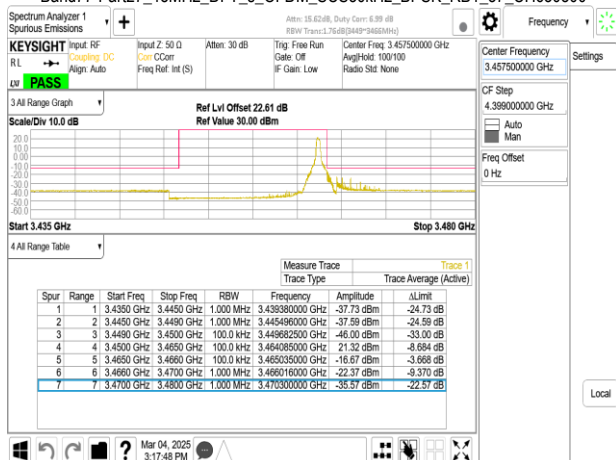
Band77-Part27_15MHz_DFT_s_OFDM_SCS30kHz_BPSK_RB36_0_CH630500
