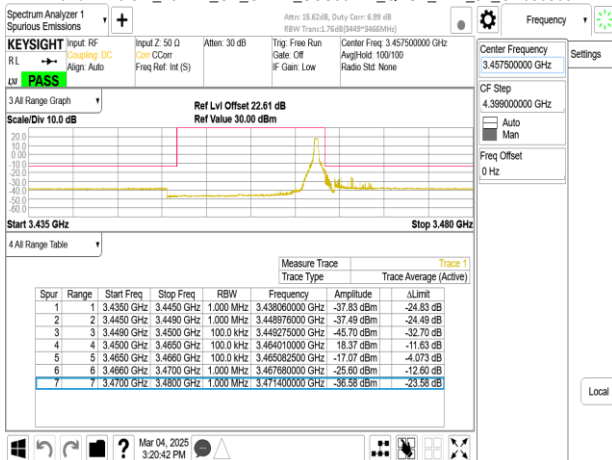
Band77-Part27_15MHz_CP_OFDM_SCS30kHz_QPSK_RB38_0_CH630500
