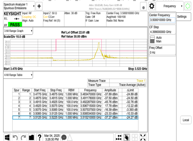
Band77-Part27_15MHz_CP_OFDM_SCS30kHz_QPSK_RB38_0_CH633334
