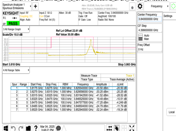
Band77-Part27_15MHz_DFT_s_OFDM_SCS30kHz_BPSK_RB36_0_CH656000
