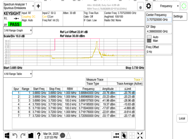
Band77-Part27_15MHz_DFT_s_OFDM_SCS30kHz_BPSK_RB36_0_CH647168
