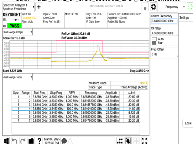
Band77-Part27_10MHz_CP_OFDM_SCS30kHz_QPSK_RB24_0_CH656000
