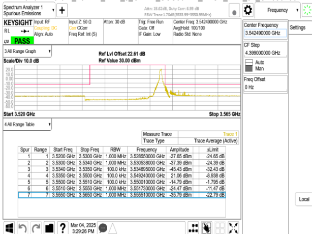
Band77-Part27_15MHz_DFT_s_OFDM_SCS30kHz_BPSK_RB36_0_CH636166
