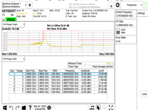
Band77-Part27_15MHz_DFT_s_OFDM_SCS30kHz_BPSK_RB1_0_CH664832
