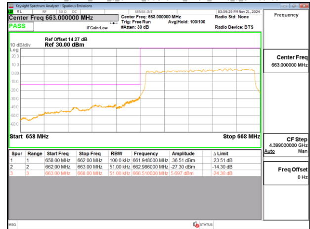
Band71_5MHz_DFT_s_OFDM_SCS15kHz_BPSK_RB1_24_CH133100
