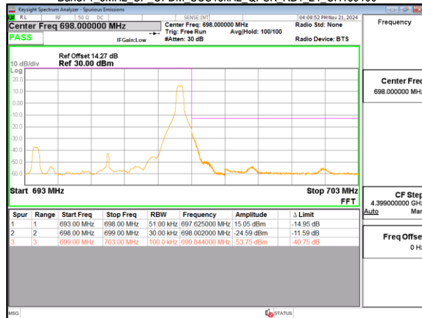
Band71_5MHz_CP_OFDM_SCS15kHz_QPSK_RB25_0_CH139100
