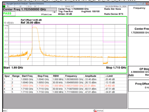
Band70_15MHz_DFT_s_OFDM_SCS15kHz_BPSK_RB1_0_CH340500
