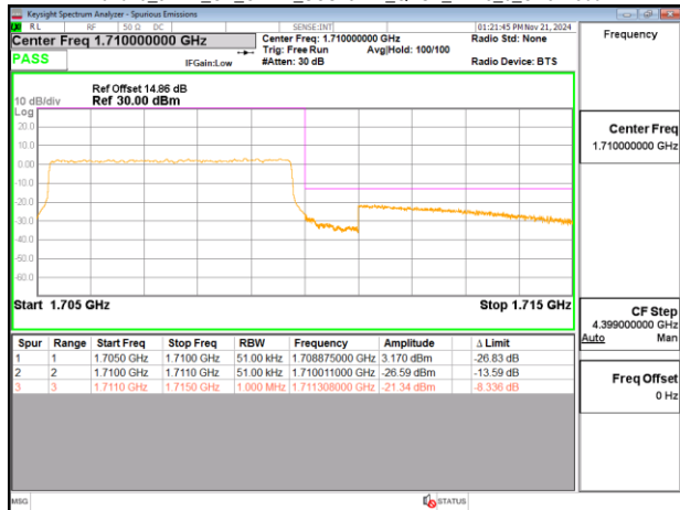
Band70_5MHz_CP_OFDM_SCS15kHz_QPSK_RB25_0_CH341500
