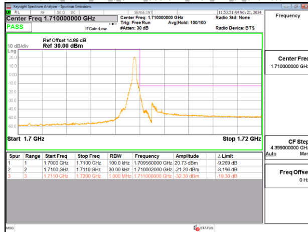
Band70_10MHz_DFT_s_OFDM_SCS15kHz_BPSK_RB1_51_CH341000
