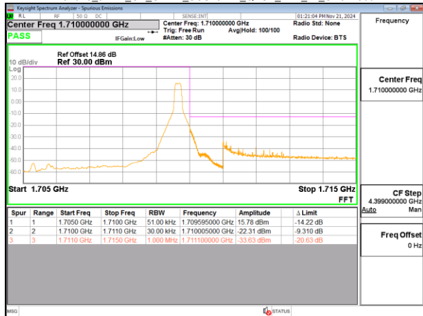
Band70_5MHz_CP_OFDM_SCS15kHz_QPSK_RB25_0_CH341500
