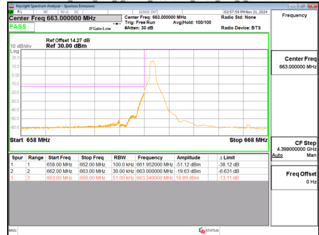
Band71_5MHz_DFT_s_OFDM_SCS15kHz_BPSK_RB25_0_CH133100
