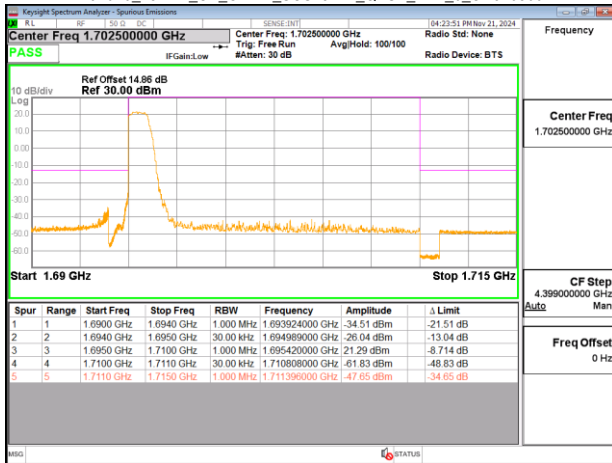
Band70_15MHz_CP_OFDM_SCS15kHz_QPSK_RB79_0_CH340500
