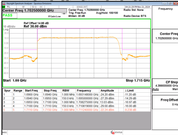
Band70_15MHz_CP_OFDM_SCS15kHz_QPSK_RB1_0_CH340500
