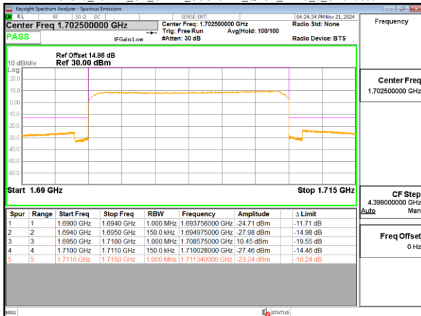
Band70_15MHz_CP_OFDM_SCS15kHz_QPSK_RB79_0_CH340500
