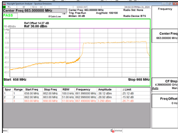
Band71_5MHz_CP_OFDM_SCS15kHz_QPSK_RB25_0_CH133100
