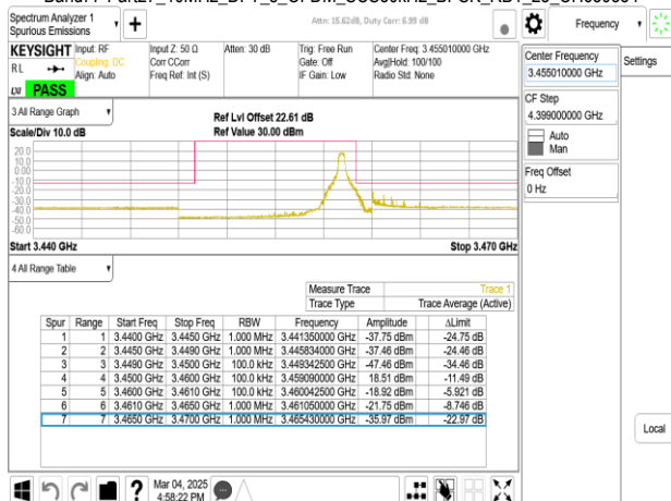
Band77-Part27_10MHz_DFT_s_OFDM_SCS30kHz_BPSK_RB24_0_CH630334
