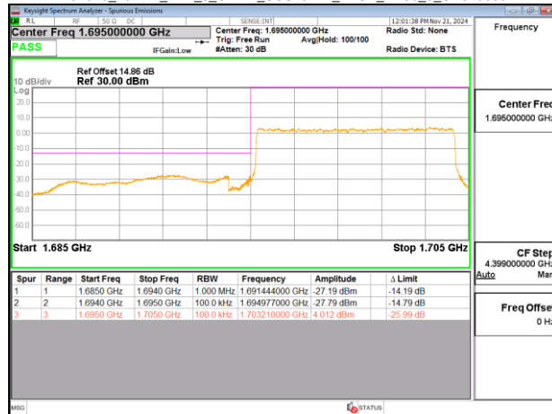
Band70_10MHz_DFT_s_OFDM_SCS15kHz_BPSK_RB1_51_CH341000
