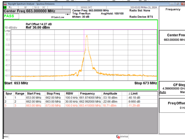
Band71_10MHz_DFT_s_OFDM_SCS15kHz_BPSK_RB1_0_CH133600
