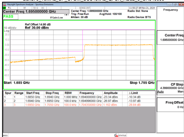
Band70_10MHz_CP_OFDM_SCS15kHz_QPSK_RB52_0_CH340000
