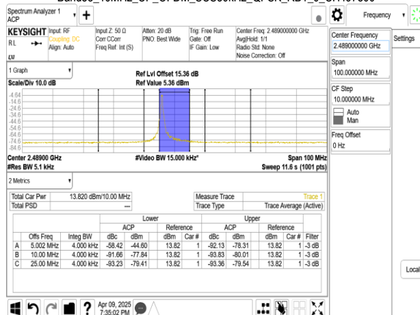
Band53_10MHz_CP_OFDM_SCS30kHz_QPSK_RB1_23_CH497800
