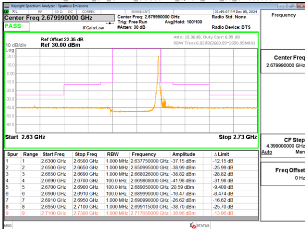
Band41_20MHz_CP_OFDM_SCS30kHz_QPSK_RB51_0_CH535998
