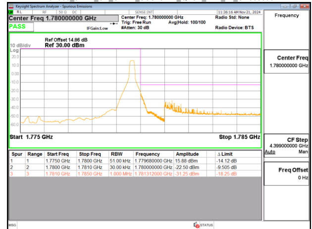
Band66_5MHz_CP_OFDM_SCS15kHz_QPSK_RB1_24_CH355500
