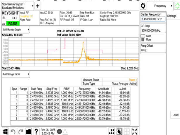
Band53_10MHz_CP_OFDM_SCS30kHz_QPSK_RB24_0_CH498000
