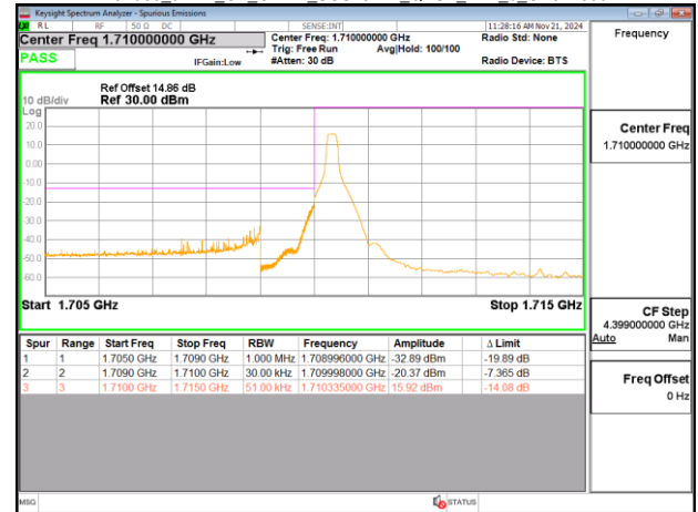
Band66_5MHz_CP_OFDM_SCS15kHz_QPSK_RB25_0_CH342500
