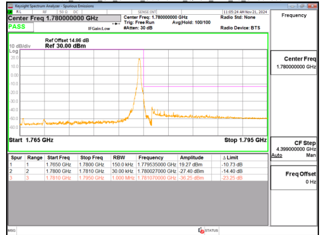
Band66_15MHz_CP_OFDM_SCS15kHz_QPSK_RB79_0_CH354500
