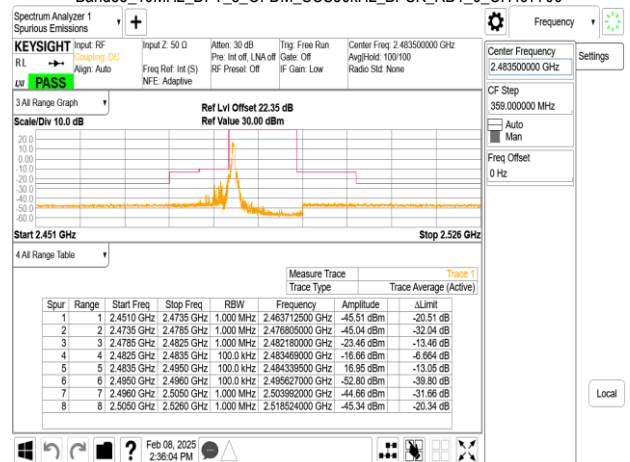
Band53_10MHz_DFT_s_OFDM_SCS30kHz_BPSK_RB24_0_CH497700
