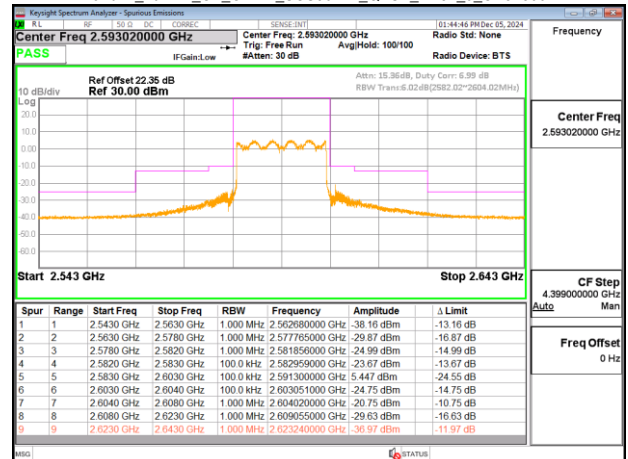
Band41_20MHz_CP_OFDM_SCS30kHz_QPSK_RB51_0_CH518604
