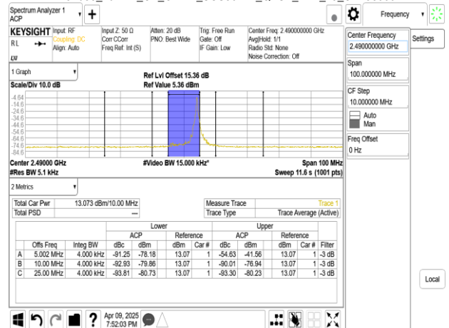
Band53_10MHz_CP_OFDM_SCS30kHz_QPSK_RB24_0_CH498000
