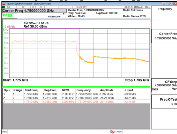
Band66_5MHz_DFT_s_OFDM_SCS15kHz_BPSK_RB25_0_CH355500
