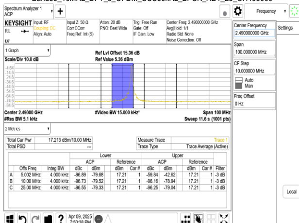
Band53_10MHz_DFT_s_OFDM_SCS30kHz_BPSK_RB1_23_CH498000
