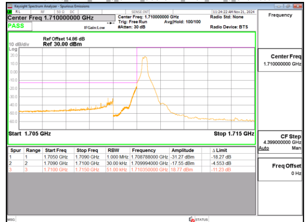
Band66_5MHz_DFT_s_OFDM_SCS15kHz_BPSK_RB1_0_CH342500
