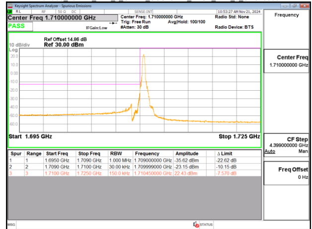
Band66_15MHz_DFT_s_OFDM_SCS15kHz_BPSK_RB75_0_CH343500
