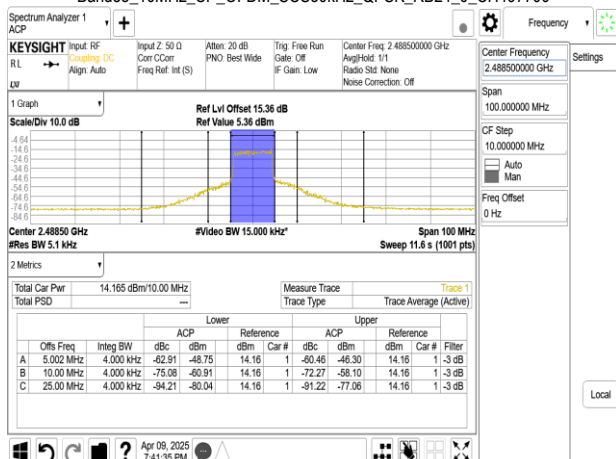
Band53_10MHz_CP_OFDM_SCS30kHz_QPSK_RB24_0_CH497700
