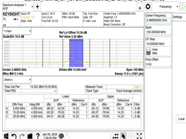
Band53_10MHz_CP_OFDM_SCS30kHz_QPSK_RB1_23_CH497700
