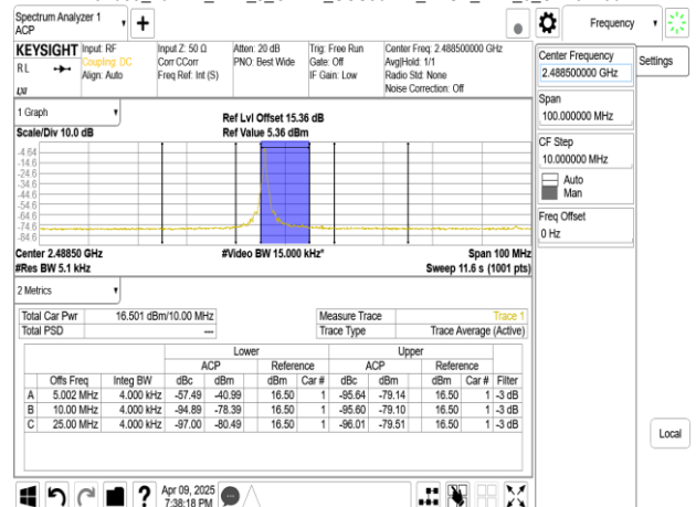
Band53_10MHz_DFT_s_OFDM_SCS30kHz_BPSK_RB1_0_CH497700
