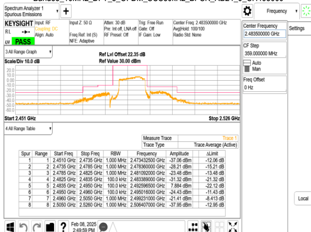
Band53_10MHz_DFT_s_OFDM_SCS30kHz_BPSK_RB1_0_CH498000
