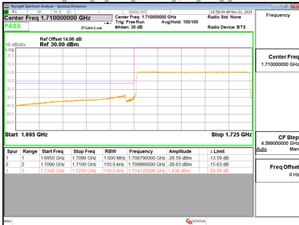
Band66_15MHz_CP_OFDM_SCS15kHz_QPSK_RB79_0_CH343500
