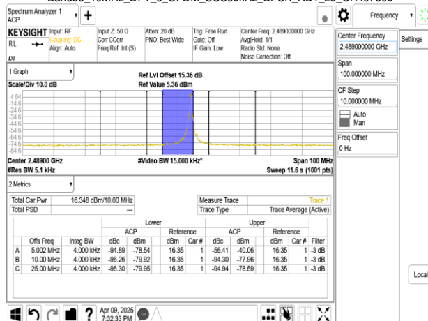
Band53_10MHz_DFT_s_OFDM_SCS30kHz_BPSK_RB24_0_CH497800
