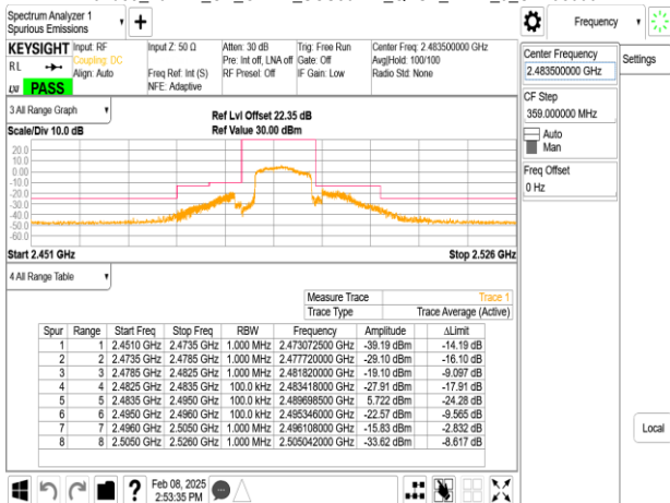
Band53_10MHz_CP_OFDM_SCS30kHz_QPSK_RB1_0_CH498000
