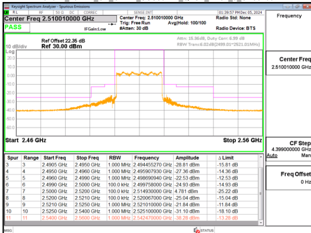
Band41_20MHz_CP_OFDM_SCS30kHz_QPSK_RB51_0_CH502002
