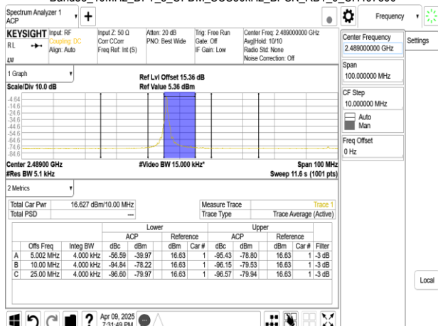
Band53_10MHz_DFT_s_OFDM_SCS30kHz_BPSK_RB1_0_CH497800
