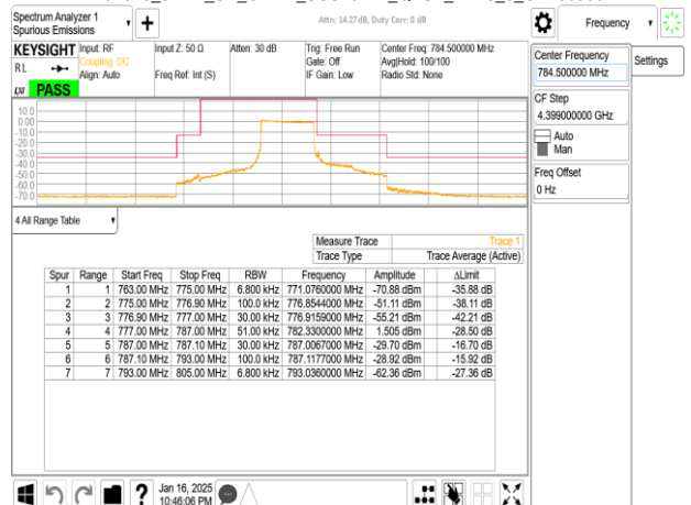
Band13_5MHz_CP_OFDM_SCS15kHz_QPSK_RB25_0_CH156900
