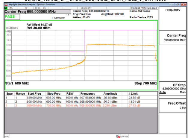
Band12_10MHz_CP_OFDM_SCS15kHz_QPSK_RB52_0_CH140800
