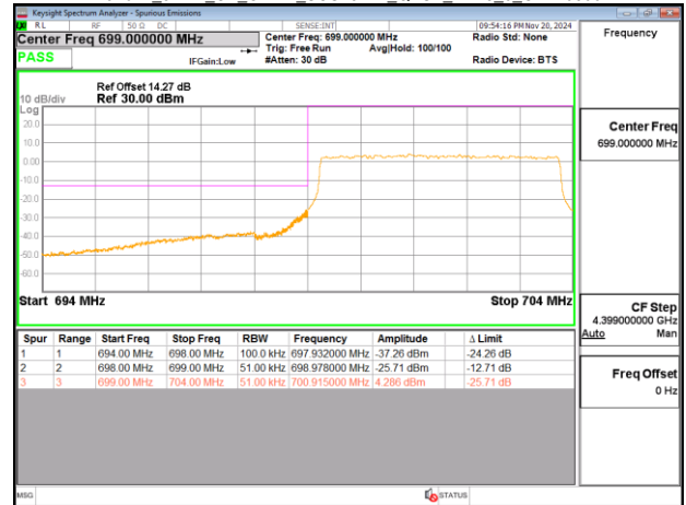
Band12_5MHz_CP_OFDM_SCS15kHz_QPSK_RB1_24_CH142700
