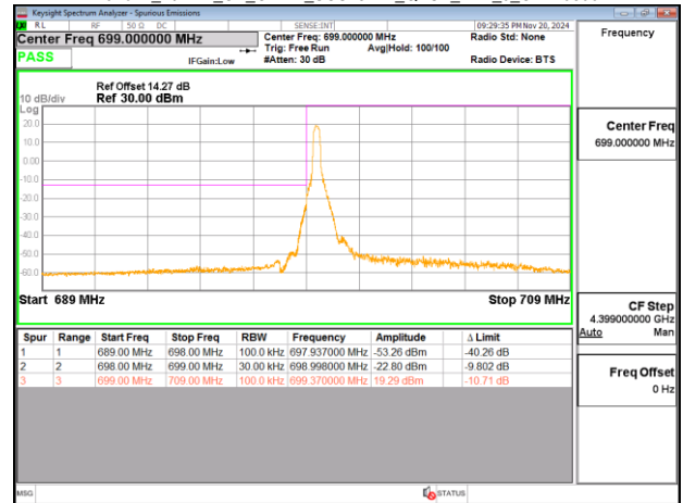
Band12_10MHz_CP_OFDM_SCS15kHz_QPSK_RB52_0_CH140800
