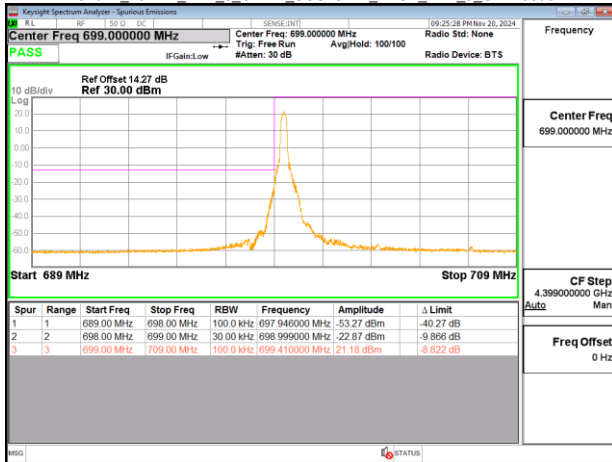
Band12_10MHz_DFT_s_OFDM_SCS15kHz_BPSK_RB50_0_CH140800
