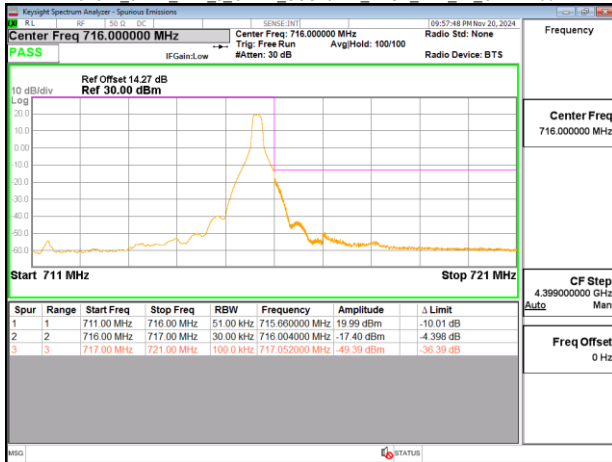
Band12_5MHz_DFT_s_OFDM_SCS15kHz_BPSK_RB25_0_CH142700
