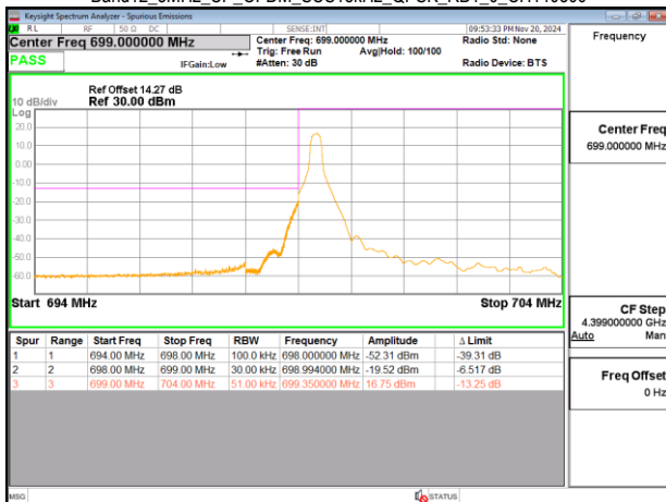
Band12_5MHz_CP_OFDM_SCS15kHz_QPSK_RB1_0_CH140300
