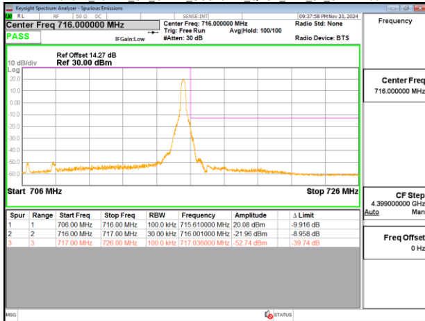
Band12_10MHz_CP_OFDM_SCS15kHz_QPSK_RB52_0_CH142200
