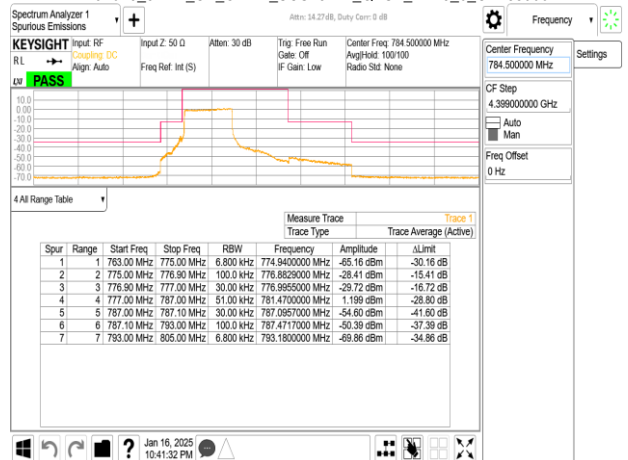
Band13_5MHz_CP_OFDM_SCS15kHz_QPSK_RB1_24_CH156900
