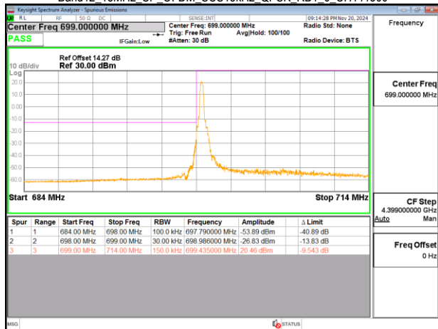
Band12_15MHz_CP_OFDM_SCS15kHz_QPSK_RB79_0_CH141300
