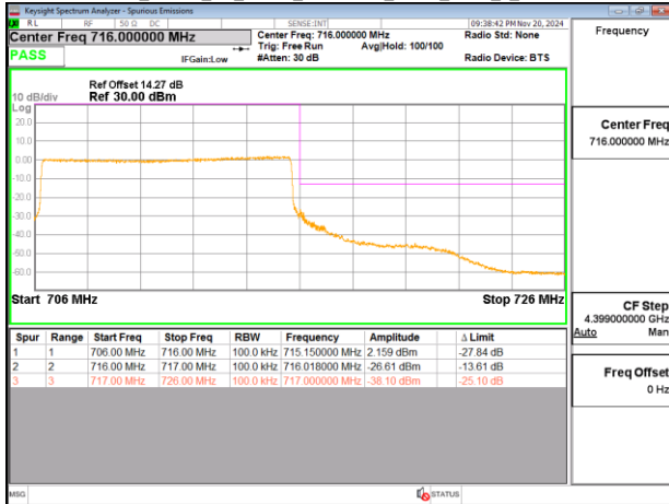
Band12_15MHz_DFT_s_OFDM_SCS15kHz_BPSK_RB1_0_CH141300
