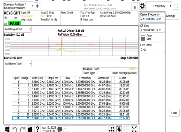
Band7_20MHz_DFT_s_OFDM_SCS15kHz_BPSK_RB1_0_CH502000
