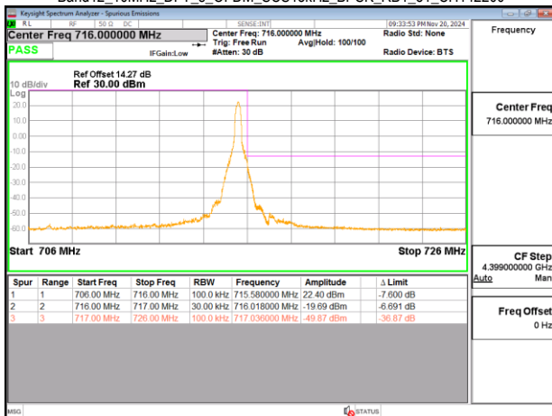
Band12_10MHz_DFT_s_OFDM_SCS15kHz_BPSK_RB1_51_CH142200
