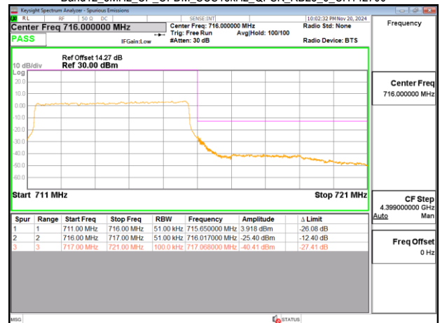
Band12_5MHz_CP_OFDM_SCS15kHz_QPSK_RB25_0_CH142700
