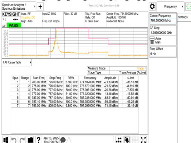
Band13_5MHz_CP_OFDM_SCS15kHz_QPSK_RB1_0_CH155900
