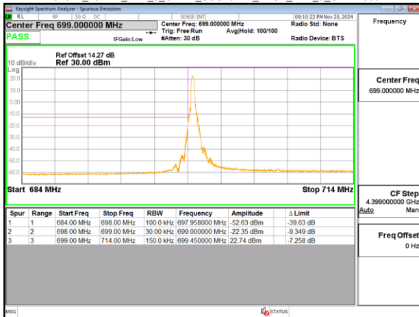
Band12_15MHz_DFT_s_OFDM_SCS15kHz_BPSK_RB1_0_CH141300
