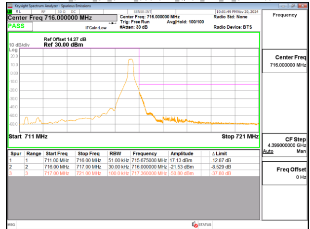
Band12_5MHz_CP_OFDM_SCS15kHz_QPSK_RB25_0_CH142700
