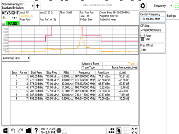
Band13_5MHz_DFT_s_OFDM_SCS15kHz_BPSK_RB25_0_CH156900
