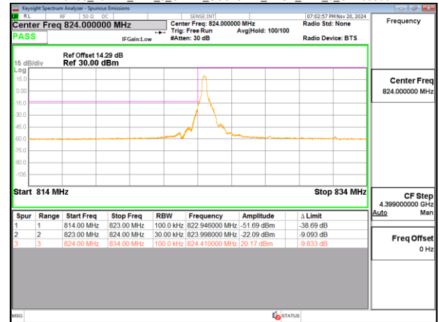
Band5_10MHz_DFT_s_OFDM_SCS15kHz_BPSK_RB50_0_CH165800
