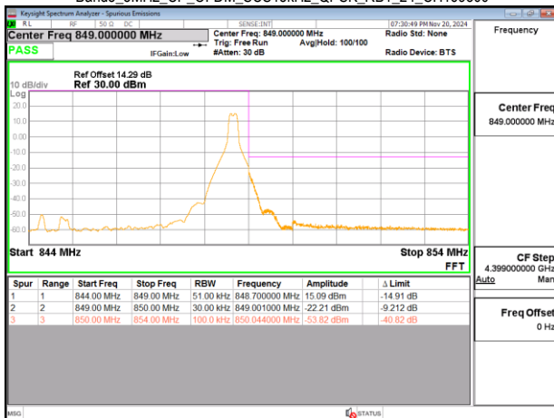
Band5_5MHz_CP_OFDM_SCS15kHz_QPSK_RB1_24_CH169300
