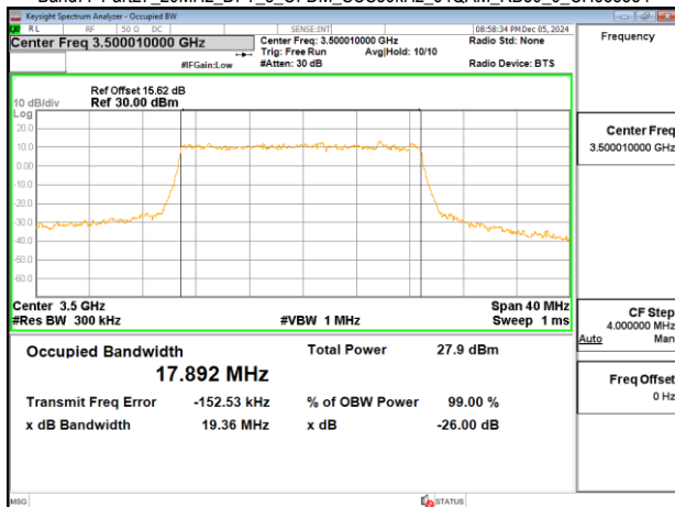
Band77-Part27_20MHz_DFT_s_OFDM_SCS30kHz_64QAM_RB50_0_CH633334
