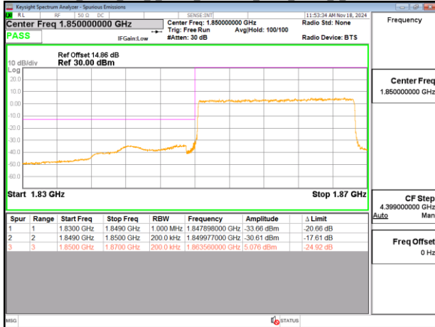
Band2 20MHz DFT s_OFDM_SCS15kHz BPSK RB1_0_CH372000
