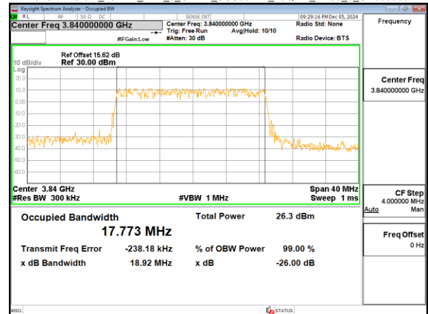
Band77-Part27_20MHz_DFT_s_OFDM_SCS30kHz_16QAM_RB50_0_CH656000
