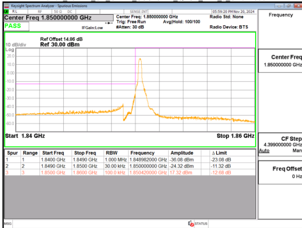
Band2_10MHz_CP_OFDM_SCS15kHz_QPSK_RB52_0_CH371000
