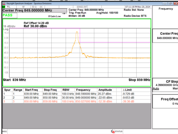
Band5_10MHz_DFT_s_OFDM_SCS15kHz_BPSK_RB50_0_CH168800
