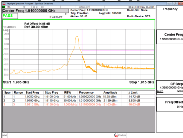
Band2_5MHz_CP_OFDM_SCS15kHz_QPSK_RB25_0_CH381500
