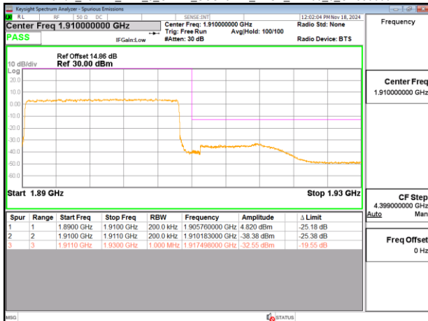
Band2 20MHz DFT s_OFDM_SCS15kHz BPSK RB100_0_CH380000
