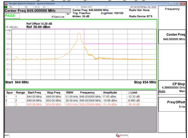
Band5_5MHz_DFT_s_OFDM_SCS15kHz_BPSK_RB25_0_CH169300
