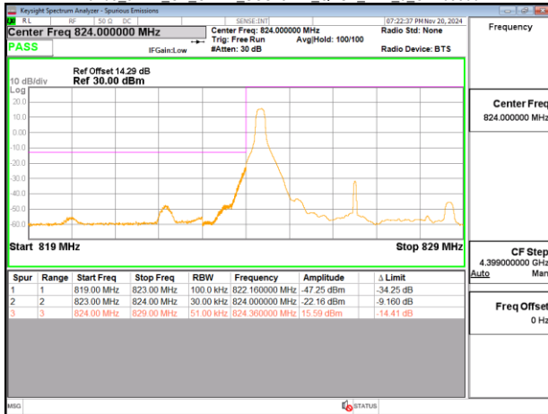
Band5_5MHz_CP_OFDM_SCS15kHz_QPSK_RB25_0_CH165300
