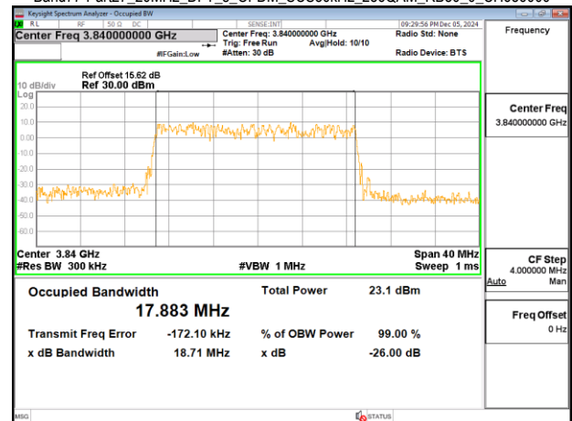
Band77-Part27_20MHz_DFT_s_OFDM_SCS30kHz_256QAM_RB50_0_CH656000
