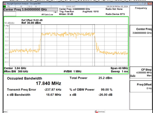
Band77-Part27_20MHz_DFT_s_OFDM_SCS30kHz_64QAM_RB50_0_CH656000
