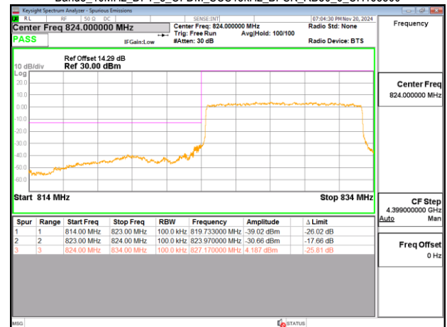
Band5_10MHz_DFT_s_OFDM_SCS15kHz_BPSK_RB50_0_CH165800
