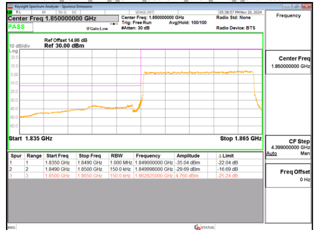
Band2_15MHz_DFT_s_OFDM_SCS15kHz_BPSK_RB75_0_CH371500
