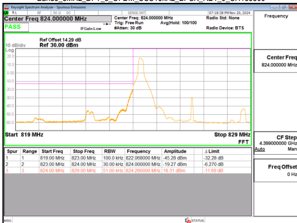
Band5_5MHz_DFT_s_OFDM_SCS15kHz_BPSK_RB1_0_CH165300
