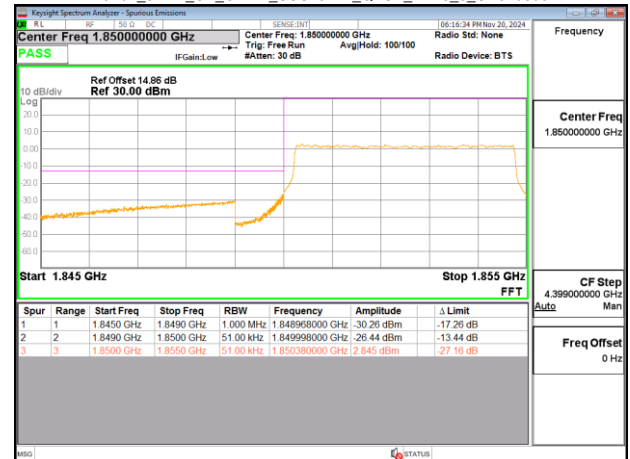
Band2_5MHz_CP_OFDM_SCS15kHz_QPSK_RB25_0_CH370500
