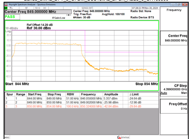
Band5_5MHz_DFT_s_OFDM_SCS15kHz_BPSK_RB25_0_CH169300
