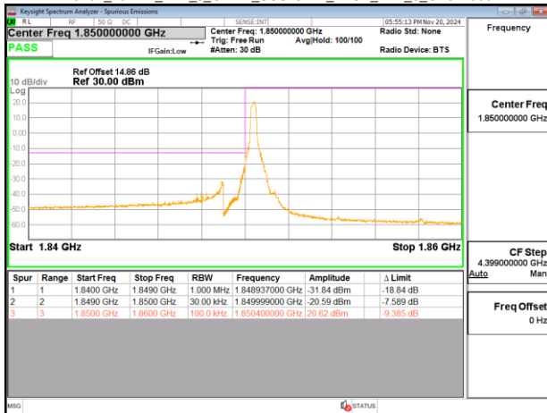
Band2_10MHz_DFT_s_OFDM_SCS15kHz_BPSK_RB1_0_CH371000
