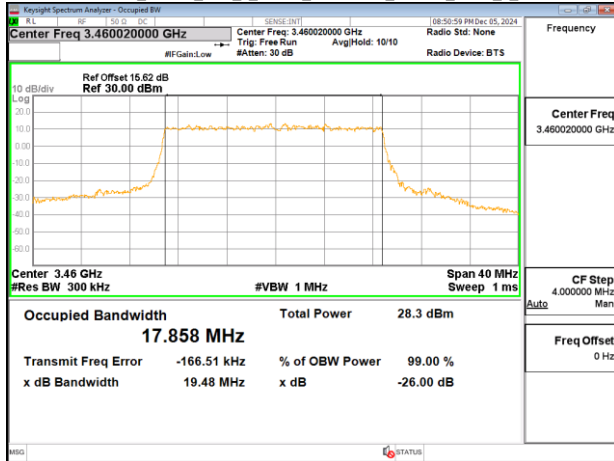
Band77-Part27_20MHz_DFT_s_OFDM_SCS30kHz_16QAM_RB50_0_CH633334
