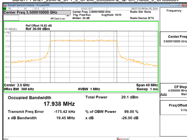
Band7-Part27_20MHz_DFT_s_OFDM_SCS30kHz_QPSK_RB50_0_CH633334
