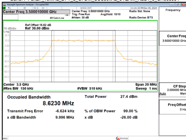
Band77-Part27_10MHz_DFT_s_OFDM_SCS30kHz_64QAM_RB24_0_CH633334
