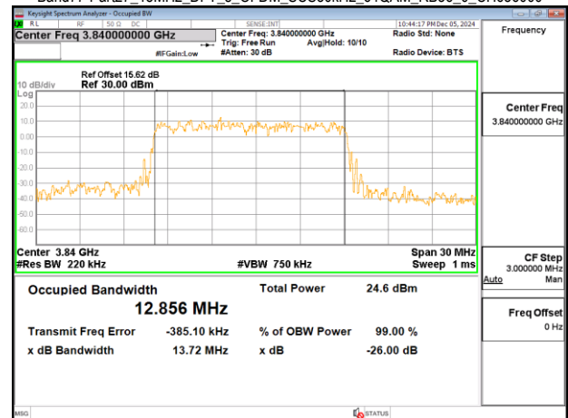
Band77-Part27_15MHz_DFT_s_OFDM_SCS30kHz_64QAM_RB36_0_CH656000
