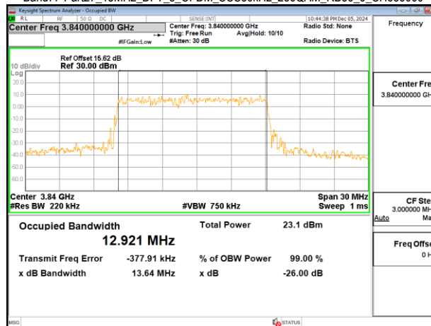
Band77-Part27_15MHz_DFT_s_OFDM_SCS30kHz_256QAM_RB36_0_CH656000
