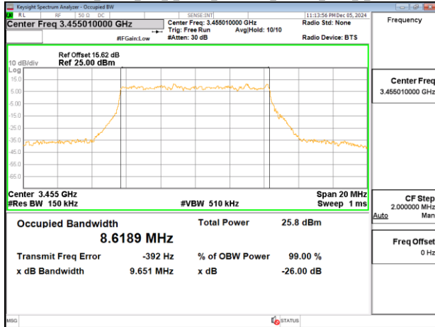
Band77-Part27_10MHz_DFT_s_OFDM_SCS30kHz_256QAM_RB24_0_CH633334
