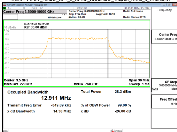
Band77-Part27_15MHz_DFT_s_OFDM_SCS30kHz_16QAM_RB36_0_CH633334
