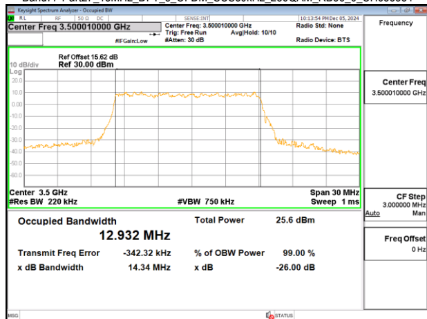
Band77-Part27_15MHz_DFT_s_OFDM_SCS30kHz_256QAM_RB36_0_CH633334
