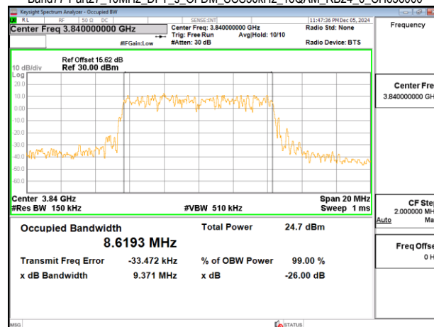
Band77-Part27_10MHz_DFT_s_OFDM_SCS30kHz_16QAM_RB24_0_CH656000
