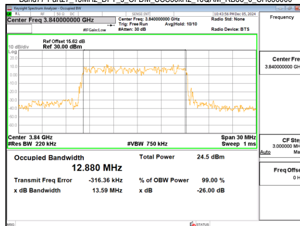
Band77-Part27_15MHz_DFT_s_OFDM_SCS30kHz_16QAM_RB36_0_CH656000
