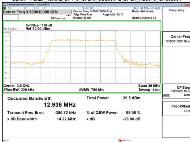
Band77-Part27_15MHz_DFT_s_OFDM_SCS30kHz_BPSK_RB36_0_CH633334
