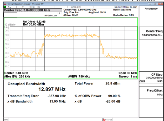
Band77-Part27_15MHz_DFT_s_OFDM_SCS30kHz_BPSK_RB36_0_CH656000
