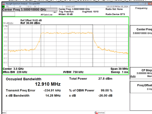
Band77-Part27_15MHz_DFT_s_OFDM_SCS30kHz_64QAM_RB36_0_CH633334
