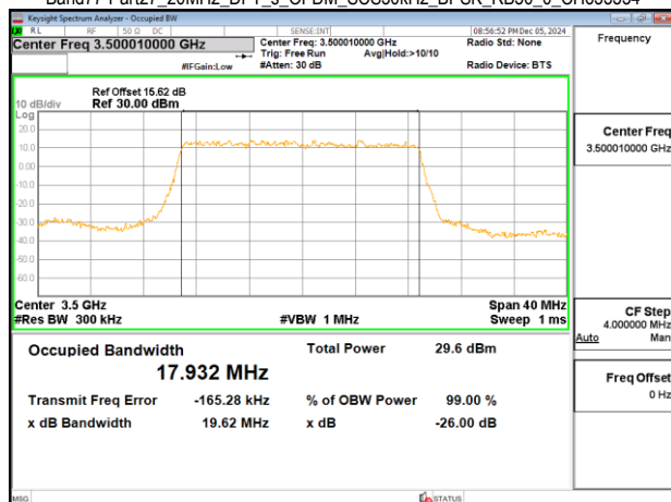
Band77-Part27_20MHz_DFT_s_OFDM_SCS30kHz_BPSK_RB50_0_CH633334
