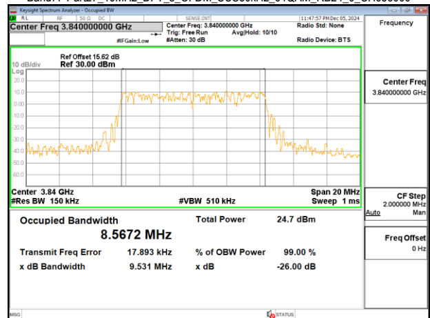
Band77-Part27_10MHz_DFT_s_OFDM_SCS30kHz_64QAM_RB24_0_CH656000
