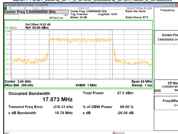
Band77-Part27_20MHz_DFT_s_OFDM_SCS30kHz_BPSK_RB50_0_CH656000
