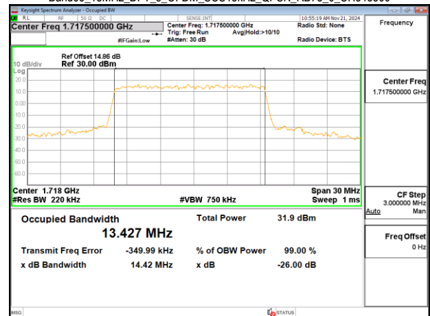
Band66_15MHz_DFT_s_OFDM_SCS15kHz_QPSK_RB75_0_CH343500
