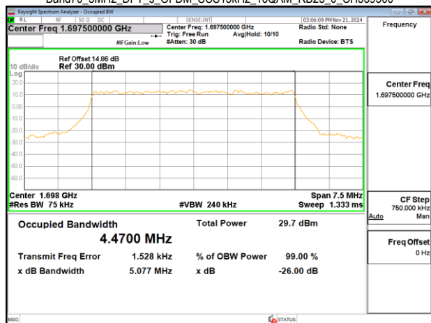
Band70_5MHz_DFT_s_OFDM_SCS15kHz_16QAM_RB25_0_CH339500
