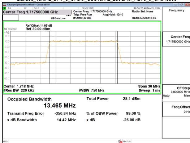
Band66_15MHz_DFT_s_OFDM_SCS15kHz_256QAM_RB75_0_CH343500
