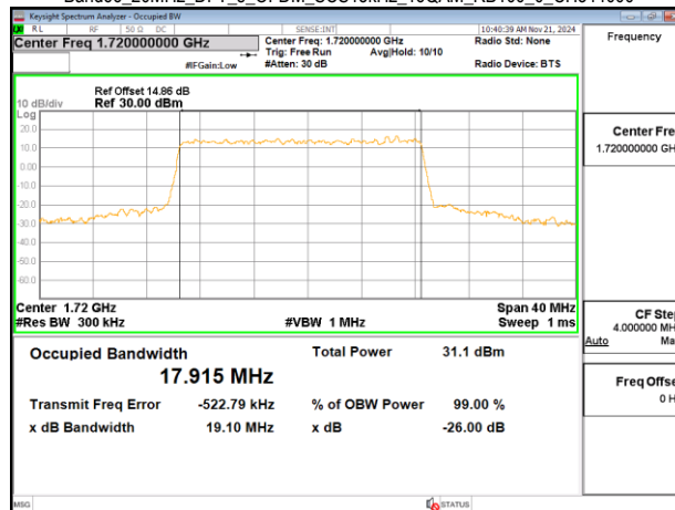
Band66_20MHz_DFT_s_OFDM_SCS15kHz_16QAM_RB100_0_CH344000
