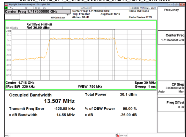
Band66_15MHz_DFT_s_OFDM_SCS15kHz_64QAM_RB75_0_CH343500
