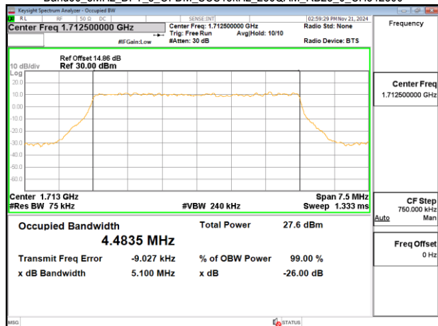
Band66_5MHz_DFT_s_OFDM_SCS15kHz_256QAM_RB25_0_CH342500
