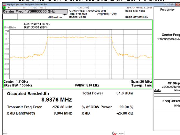
Band70_10MHz_DFT_s_OFDM_SCS15kHz_QPSK_RB50_0_CH340000
