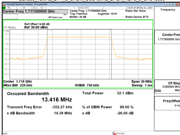
Band66_15MHz_DFT_s_OFDM_SCS15kHz_BPSK_RB75_0_CH343500
