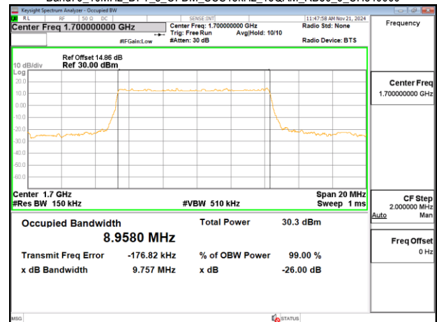
Band70_10MHz_DFT_s_OFDM_SCS15kHz_16QAM_RB50_0_CH340000
