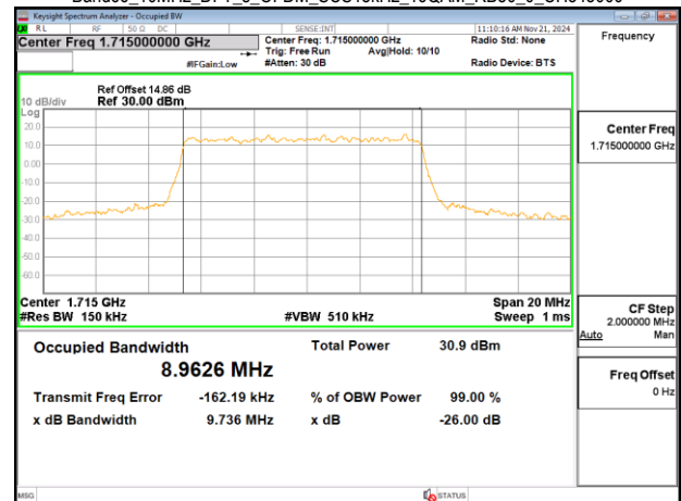
Band66 10MHz DFT s_OFDM_SCS15kHz_16QAM_RB50_0_CH343000
