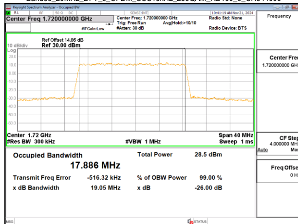
Band66_20MHz_DFT_s_OFDM_SCS15kHz_256QAM_RB100_0_CH344000
