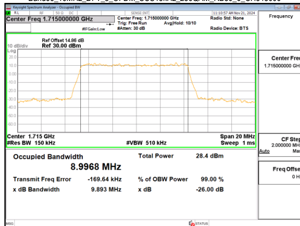
Band66_10MHz_DFT_s_OFDM_SCS15kHz_256QAM_RB50_0_CH343000
