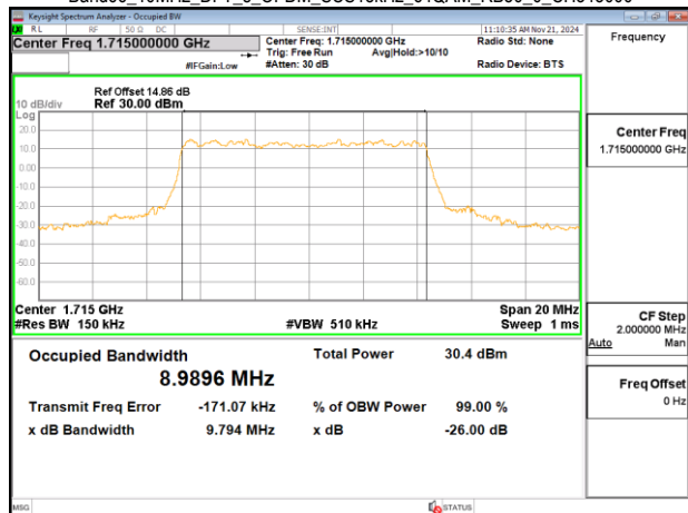
Band66_10MHz_DFT_s_OFDM_SCS15kHz_64QAM_RB50_0_CH343000
