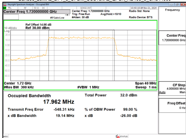
Band66_20MHz_DFT_s_OFDM_SCS15kHz_QPSK_RB100_0_CH344000
