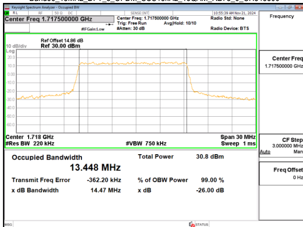
Band66_15MHz_DFT_s_OFDM_SCS15kHz_16QAM_RB75_0_CH343500
