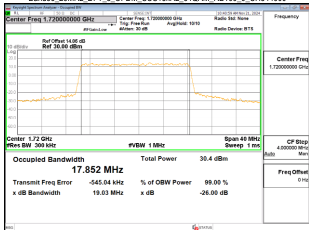
Band66_20MHz_DFT_s_OFDM_SCS15kHz_64QAM_RB100_0_CH344000
