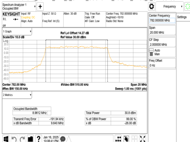
Band13_10MHz_DFT_s_OFDM_SCS15kHz_16QAM_RB50_0_CH156400
