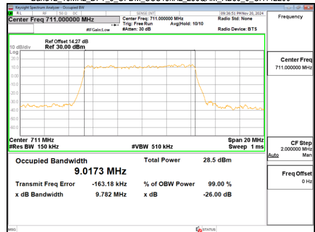
Band12_10MHz_DFT_s_OFDM_SCS15kHz_256QAM_RB50_0_CH142200
