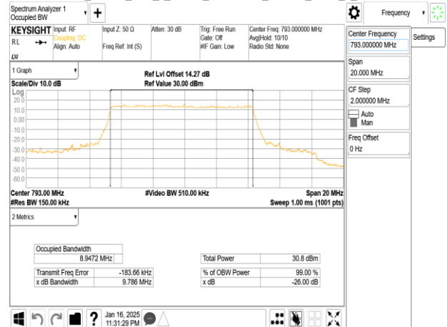
Band14_10MHz_DFT_s_OFDM_SCS15kHz_64QAM_RB50_0_CH158600
