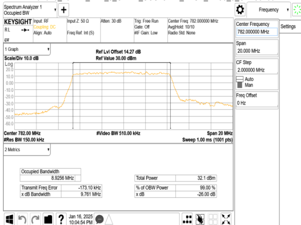
Band13_10MHz_DFT_s_OFDM_SCS15kHz_QPSK_RB50_0_CH156400
