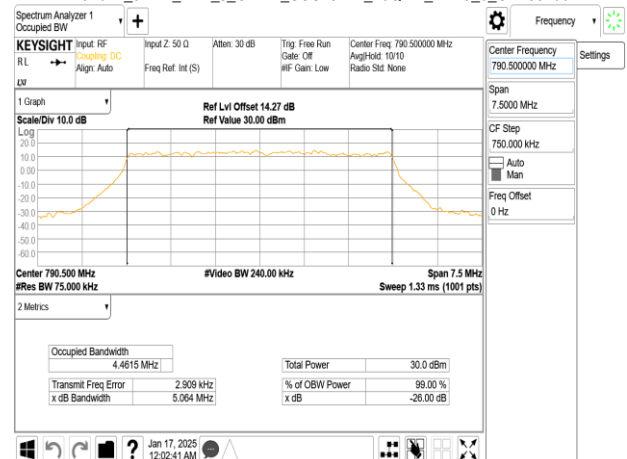
Band14_5MHz_DFT_s_OFDM_SCS15kHz_16QAM_RB25_0_CH158100
