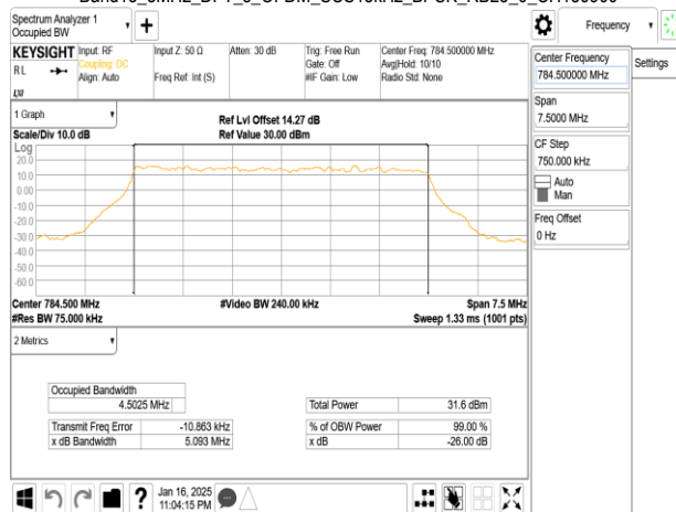
Band13_5MHz_DFT_s_OFDM_SCS15kHz_BPSK_RB25_0_CH156900
