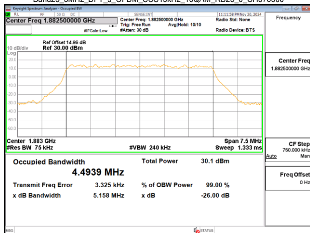
Band25_5MHz_DFT_s_OFDM_SCS15kHz_16QAM_RB25_0_CH376500
