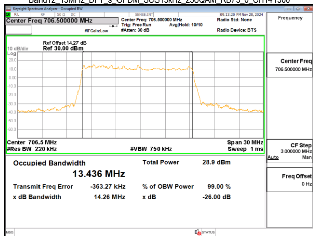
Band12_15MHz_DFT_s_OFDM_SCS15kHz_256QAM_RB75_0_CH141500
