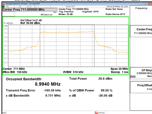
Band12_10MHz_DFT_s_OFDM_SCS15kHz_64QAM_RB50_0_CH142200
