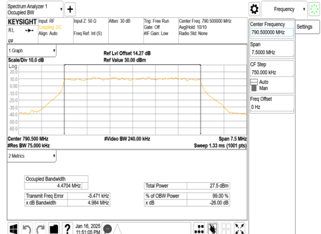
Band14_5MHz_DFT_s_OFDM_SCS15kHz_256QAM_RB25_0_CH158100
