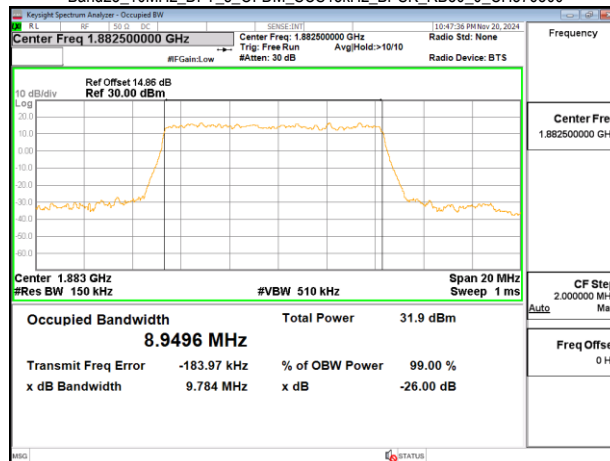
Band25_10MHz_DFT_s_OFDM_SCS15kHz_BPSK_RB50_0_CH376500
