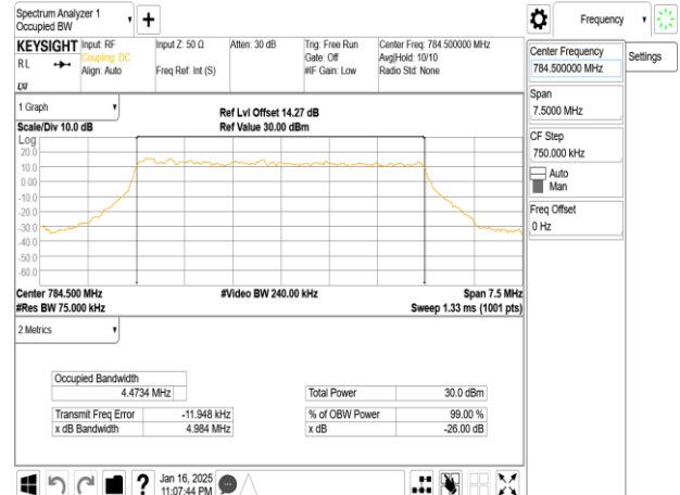
Band13_5MHz_DFT_s_OFDM_SCS15kHz_16QAM_RB25_0_CH156900
