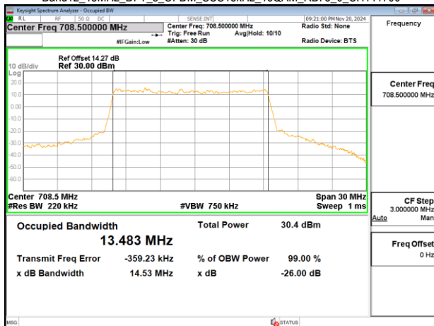
Band12_15MHz_DFT_s_OFDM_SCS15kHz_16QAM_RB75_0_CH141700
