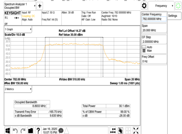
Band13_10MHz_DFT_s_OFDM_SCS15kHz_256QAM_RB50_0_CH156400
