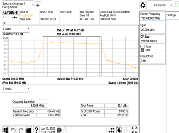
Band14_10MHz_DFT_s_OFDM_SCS15kHz_BPSK_RB50_0_CH158600
