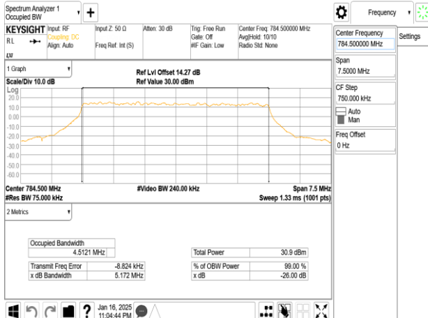
Band13_5MHz_DFT_s_OFDM_SCS15kHz_QPSK_RB25_0_CH156900
