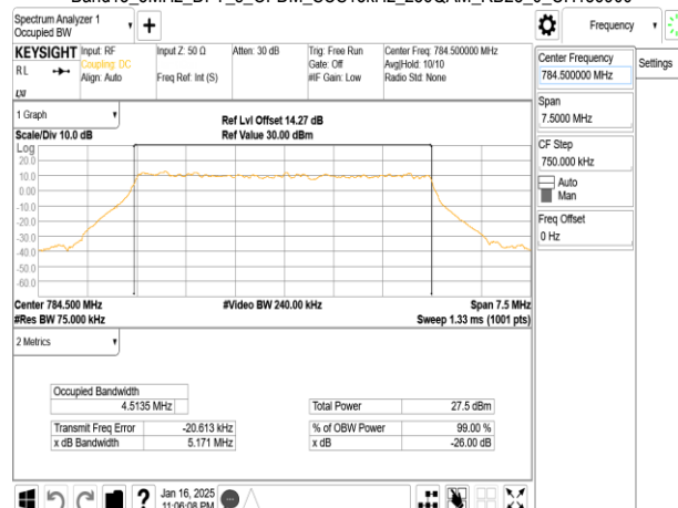
Band13_5MHz_DFT_s_OFDM_SCS15kHz_256QAM_RB25_0_CH156900
