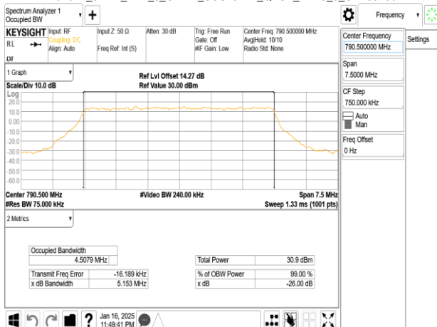
Band14_5MHz_DFT_s_OFDM_SCS15kHz_QPSK_RB25_0_CH158100
