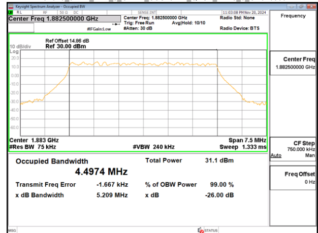
Band25_5MHz_DFT_s_OFDM_SCS15kHz_QPSK_RB25_0_CH376500
