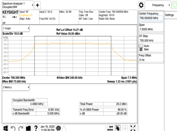
Band14_5MHz_DFT_s_OFDM_SCS15kHz_64QAM_RB25_0_CH158100
