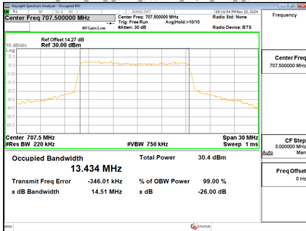
Band12_15MHz_DFT_s_OFDM_SCS15kHz_16QAM_RB75_0_CH141700
