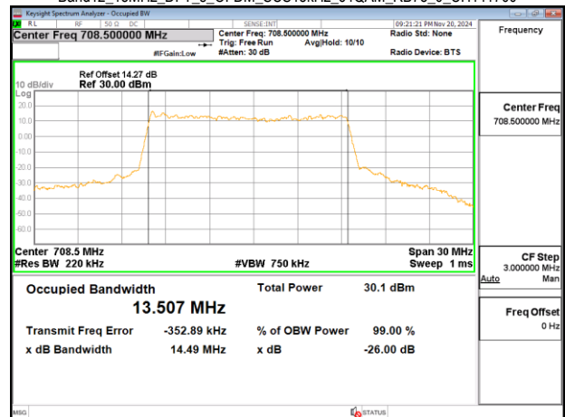
Band12_15MHz_DFT_s_OFDM_SCS15kHz_64QAM_RB75_0_CH141700
