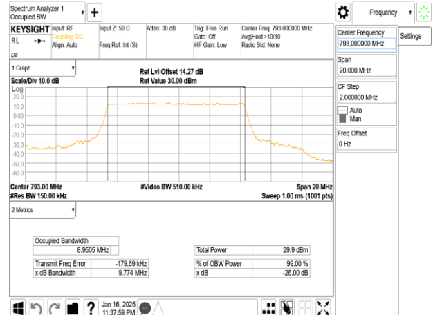
Band14_10MHz_DFT_s_OFDM_SCS15kHz_64QAM_RB50_0_CH158600
