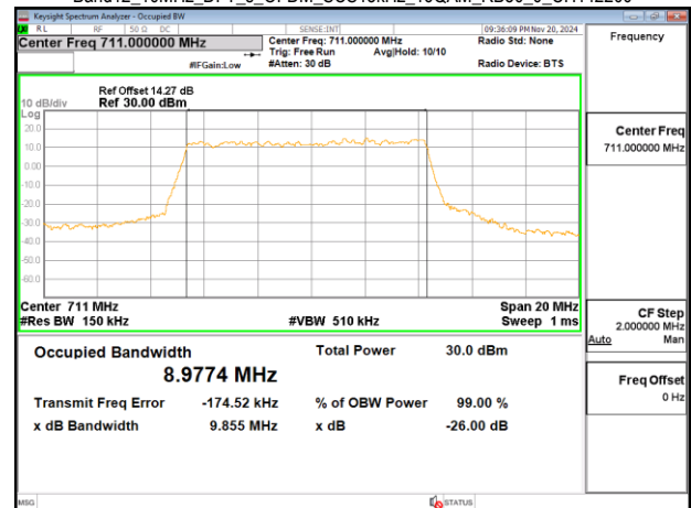
Band12_10MHz_DFT_s_OFDM_SCS15kHz_16QAM_RB50_0_CH142200
