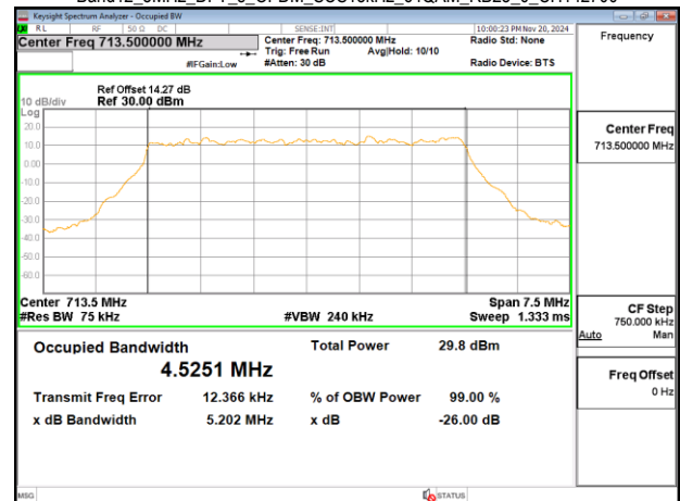
Band12_5MHz_DFT_s_OFDM_SCS15kHz_64QAM_RB25_0_CH142700
