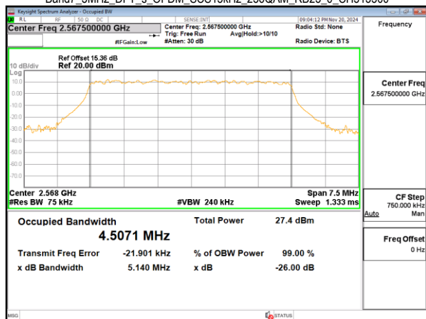
Band7_5MHz_DFT_s_OFDM_SCS15kHz_256QAM_RB25_0_CH513500
