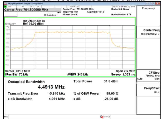
Band12_5MHz_DFT_s_OFDM_SCS15kHz_QPSK_RB25_0_CH141500
