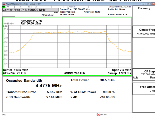
Band12_5MHz_DFT_s_OFDM_SCS15kHz_16QAM_RB25_0_CH142700
