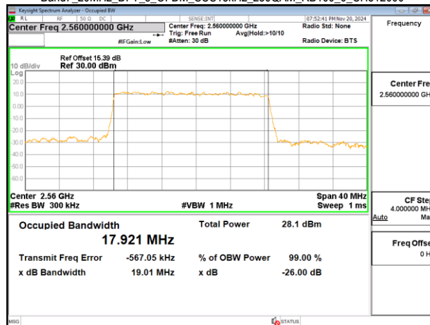
Band7_20MHz_DFT_s_OFDM_SCS15kHz_256QAM_RB100_0_CH512000
