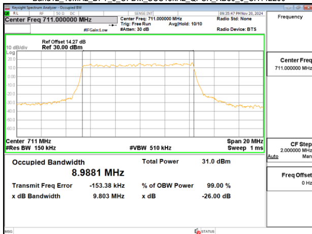
Band12_10MHz_DFT_s_OFDM_SCS15kHz_QPSK_RB50_0_CH142200
