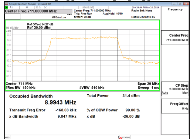
Band12_10MHz_DFT_s_OFDM_SCS15kHz_BPSK_RB50_0_CH142200
