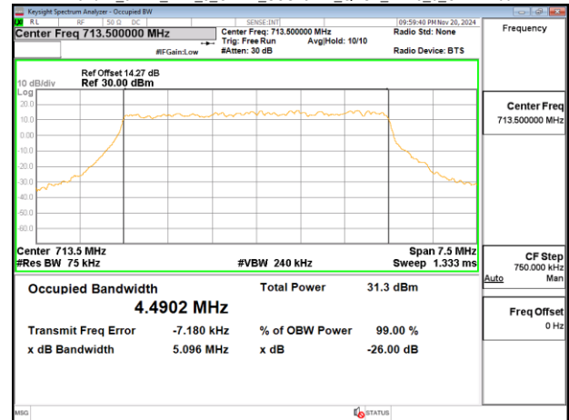
Band12_5MHz_DFT_s_OFDM_SCS15kHz_QPSK_RB25_0_CH142700
