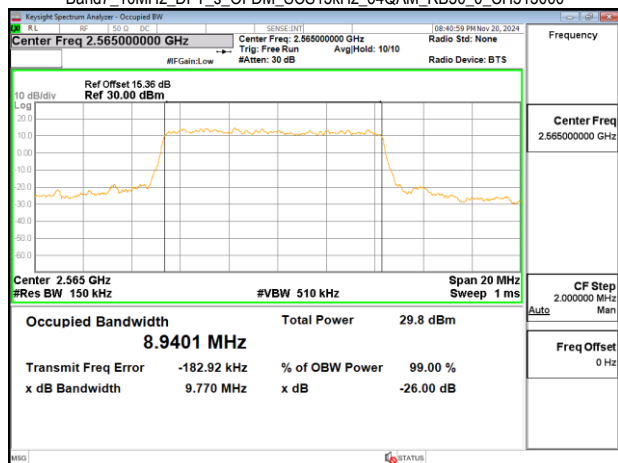
Band7_10MHz_DFT_s_OFDM_SCS15kHz_64QAM_RB50_0_CH513000
