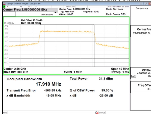
Band7_20MHz_DFT_s_OFDM_SCS15kHz_16QAM_RB100_0_CH512000
