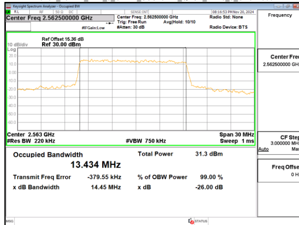
Band7_15MHz_DFT_s_OFDM_SCS15kHz_QPSK_RB75_0_CH512500
