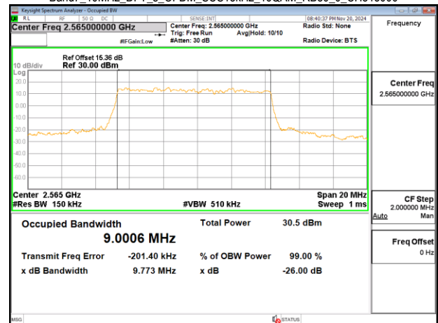
Band7_10MHz_DFT_s_OFDM_SCS15kHz_16QAM_RB50_0_CH513000
