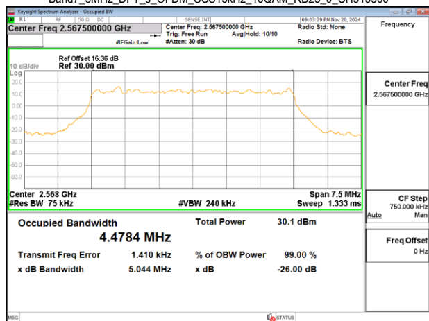
Band7_5MHz_DFT_s_OFDM_SCS15kHz_16QAM_RB25_0_CH513500
