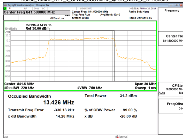
Band5_15MHz_DFT_s_OFDM_SCS15kHz_QPSK_RB75_0_CH168300
