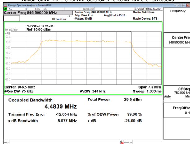
Band5_5MHz_DFT_s_OFDM_SCS15kHz_64QAM_RB25_0_CH169300
