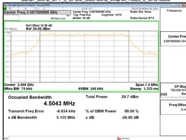
Band7_5MHz_DFT_s_OFDM_SCS15kHz_64QAM_RB25_0_CH513500
