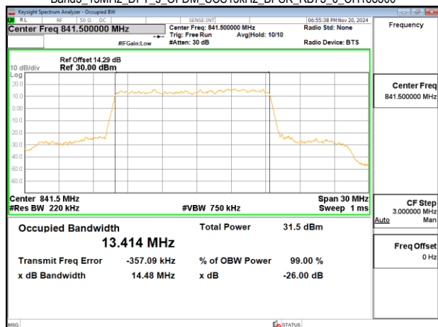
Band5_15MHz_DFT_s_OFDM_SCS15kHz_BPSK_RB75_0_CH168300
