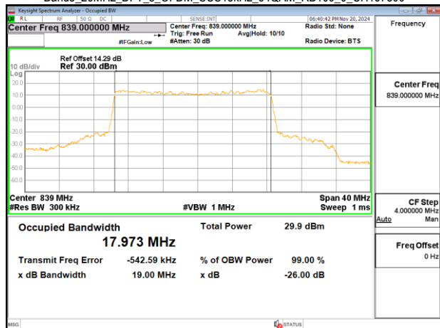
Band5_20MHz_DFT_s_OFDM_SCS15kHz_64QAM_RB100_0_CH167800
