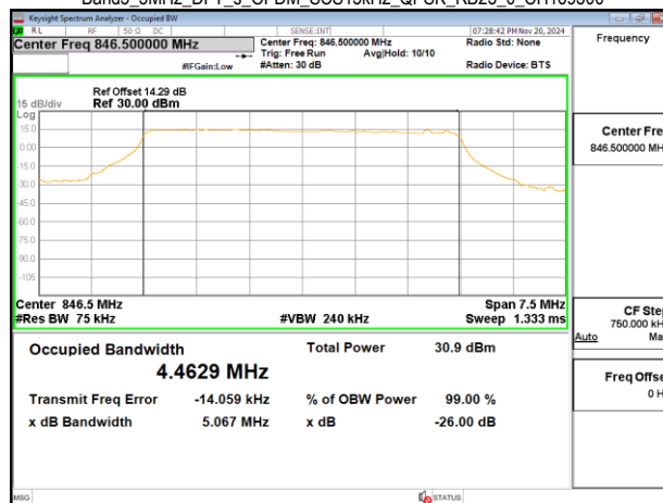
Band5_5MHz_DFT_s_OFDM_SCS15kHz_QPSK_RB25_0_CH169300
