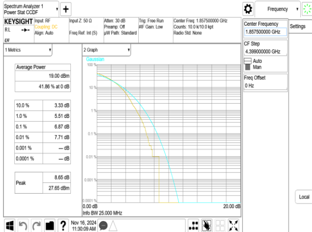
Band25_15MHz_256QAM_RB75_0_CH26115
