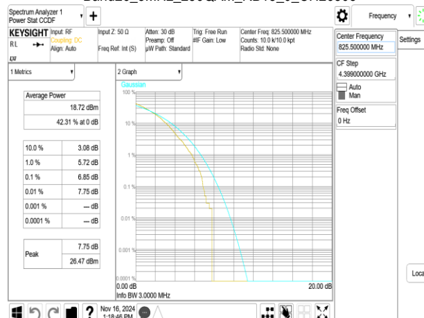
Band26_3MHz_256QAM_RB15_0_CH26805
