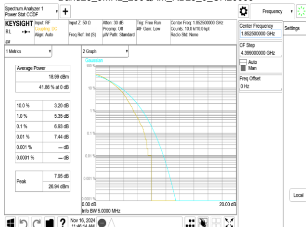
Band25_5MHz_256QAM_RB25_0_CH26065
