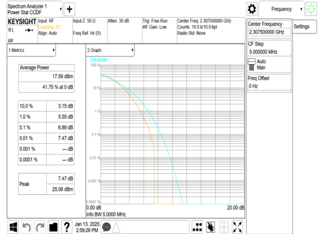
Band30_5MHz_256QAM_RB25_0_CH27710
