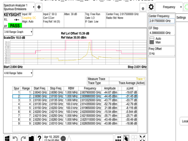
Band38_5MHz_QPSK_RB1_24_CH38225
