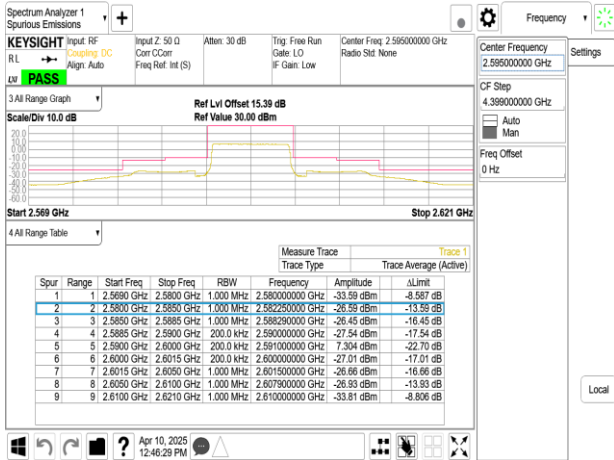
Band38_10MHz_QPSK_RB1_0_CH38200
