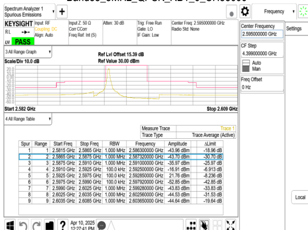
Band38_5MHz_QPSK_RB1_24_CH38000
