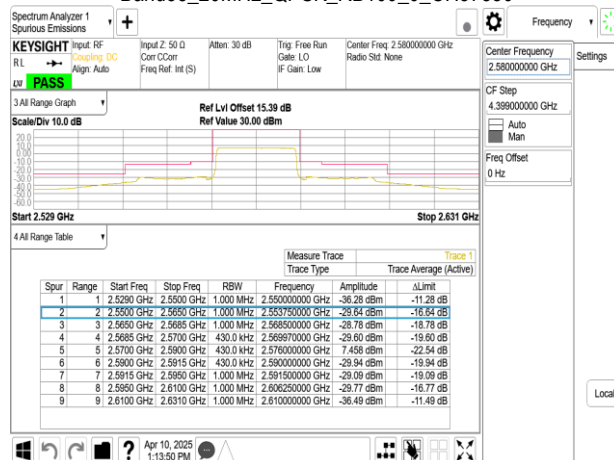
Band38_20MHz_QPSK_RB1_0_CH38000
