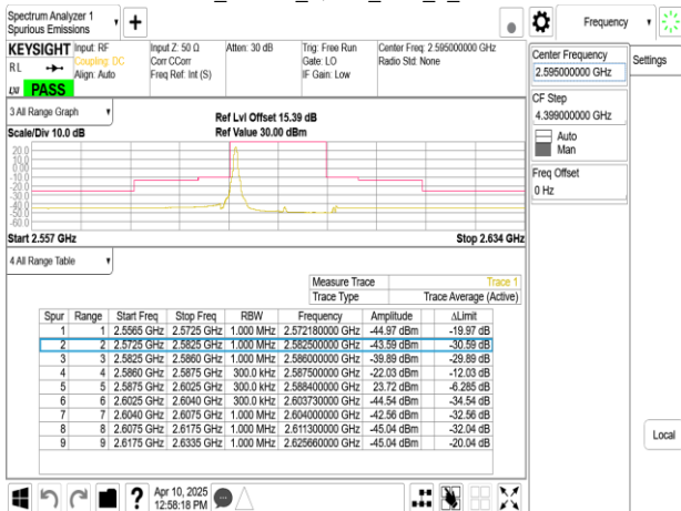
Band38_15MHz_QPSK_RB1_74_CH38000
