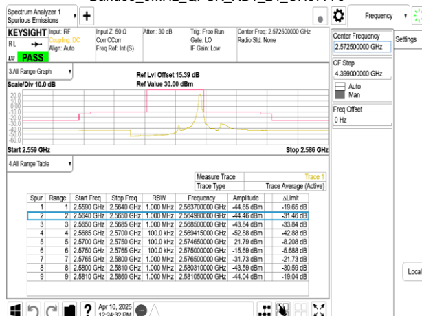
Band38_5MHz_QPSK_RB1_24_CH37775
