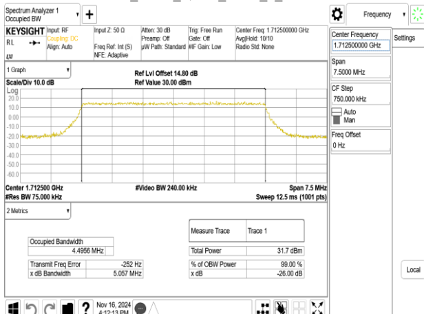
Band66_5MHz_QPSK_RB25_0_CH131997
