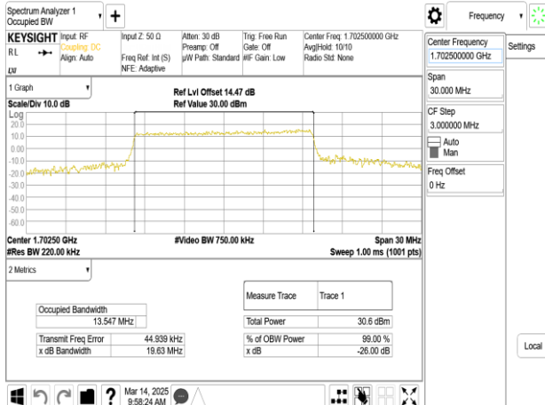
Band70_15MHz_16QAM_75_0_CH133047
