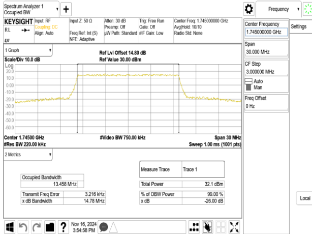
Band66_15MHz_16QAM_RB75_0_CH132322
