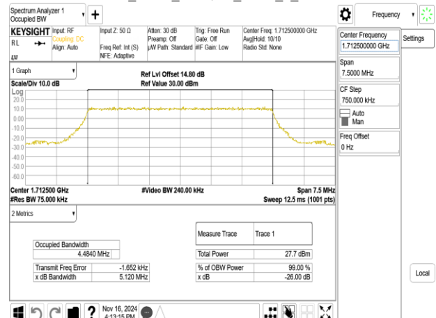
Band66_5MHz_256QAM_RB25_0_CH131997
