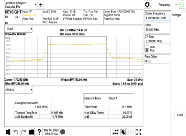
Band70_15MHz_QPSK_75_0_CH133047
