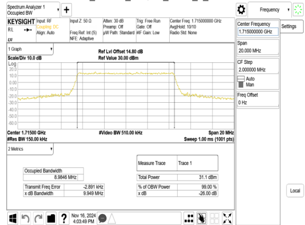
Band66_10MHz_64QAM_RB50_0_CH132022
