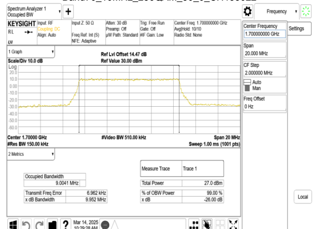
Band70_10MHz_256QAM_50_0_CH133022
