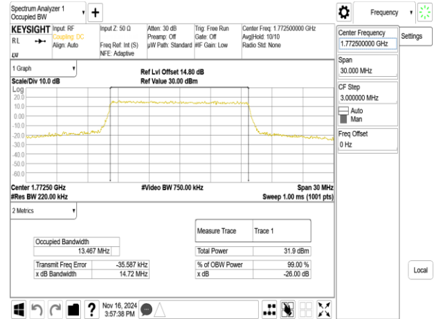
Band66_15MHz_16QAM_RB75_0_CH132597
