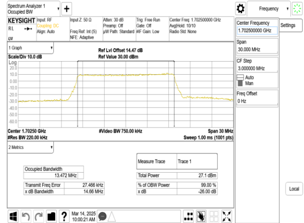
Band70_15MHz_64QAM_75_0_CH133047
