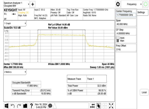
Band66_20MHz_16QAM_RB100_0_CH132572
