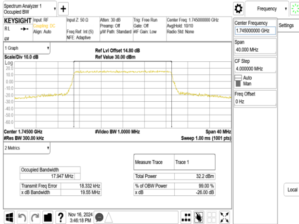
Band66_20MHz_16QAM_RB100_0_CH132322
