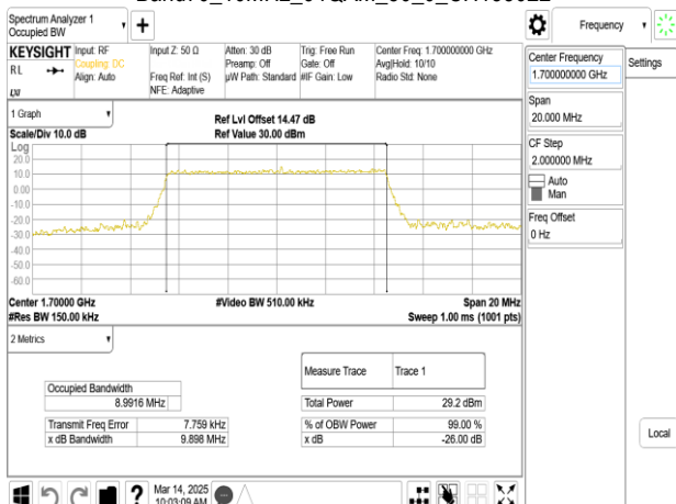
Band70_10MHz_64QAM_50_0_CH133022
