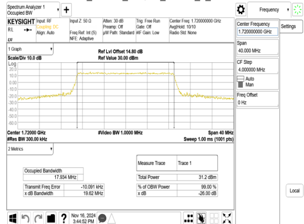
Band66_20MHz_64QAM_RB100_0_CH132072
