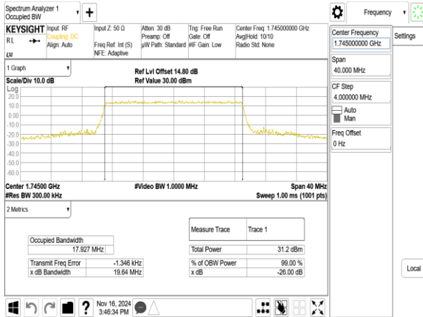
Band66_20MHz_64QAM_RB100_0_CH132322
