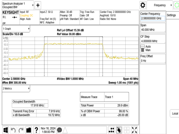
Band38_20MHz_256QAM_RB100_0_CH37850
