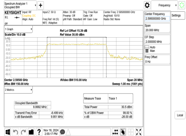
Band38_10MHz_64QAM_RB50_0_CH38000
