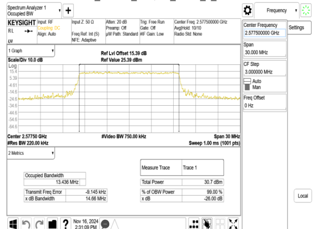
Band38_15MHz_16QAM_RB75_0_CH37825
