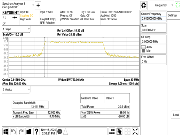
Band38_15MHz_64QAM_RB75_0_CH38175
