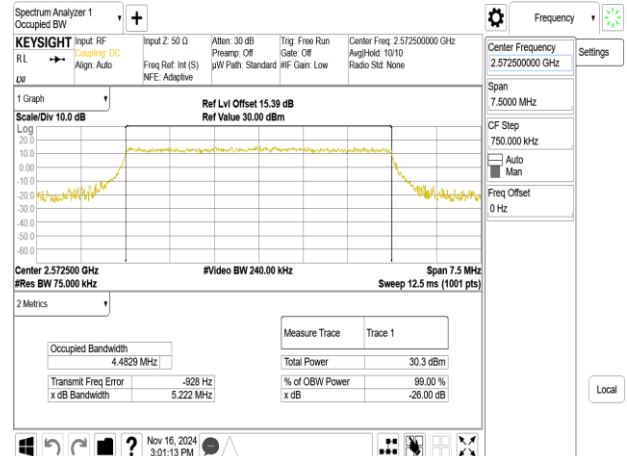
Band38_5MHz_16QAM_RB25_0_CH37775
