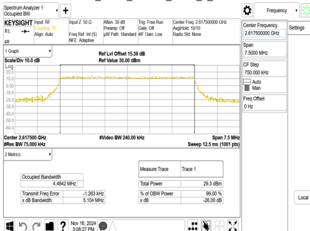
Band38_5MHz_64QAM_RB25_0_CH38225
