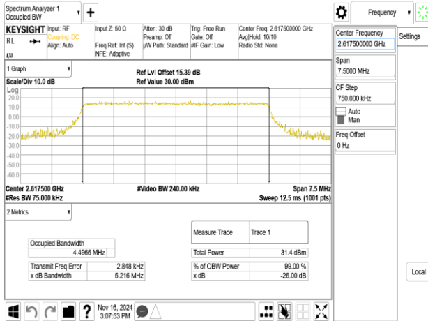
Band38_5MHz_16QAM_RB25_0_CH38225
