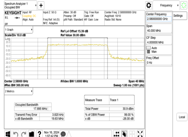
Band38_20MHz_16QAM_RB100_0_CH37850
