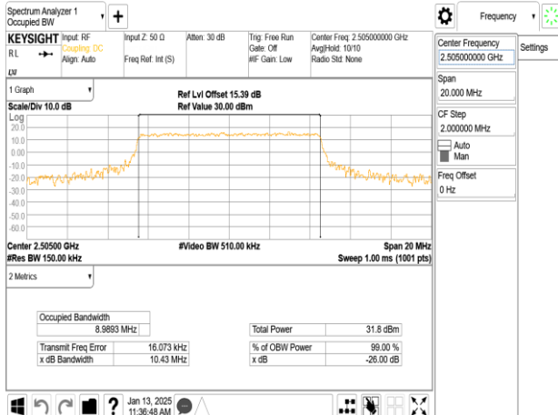
Band41_10MHz_64QAM_RB50_0_CH39740
