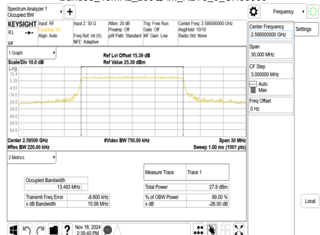
Band38_15MHz_256QAM_RB75_0_CH38000
