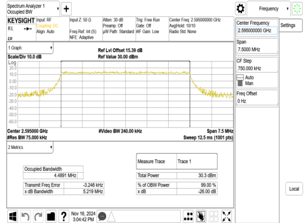
Band38_5MHz_64QAM_RB25_0_CH38000
