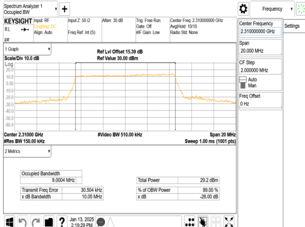
Band30_10MHz_64QAM_RB50_0_CH27710
