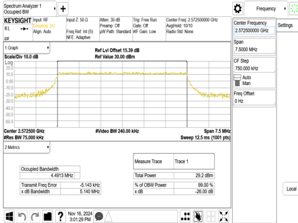
Band38_5MHz_256QAM_RB25_0_CH37775
