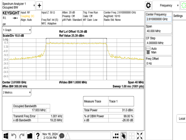
Band38_20MHz_64QAM_RB100_0_CH38150
