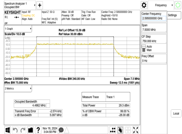
Band38_5MHz_256QAM_RB25_0_CH38000
