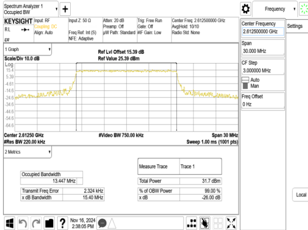
Band38_15MHz_16QAM_RB75_0_CH38175
