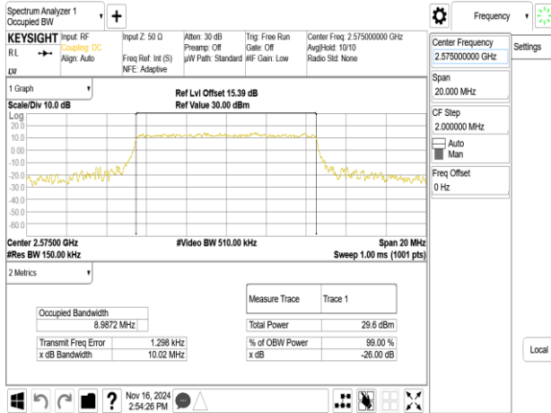
Band38_10MHz_256QAM_RB50_0_CH37800
