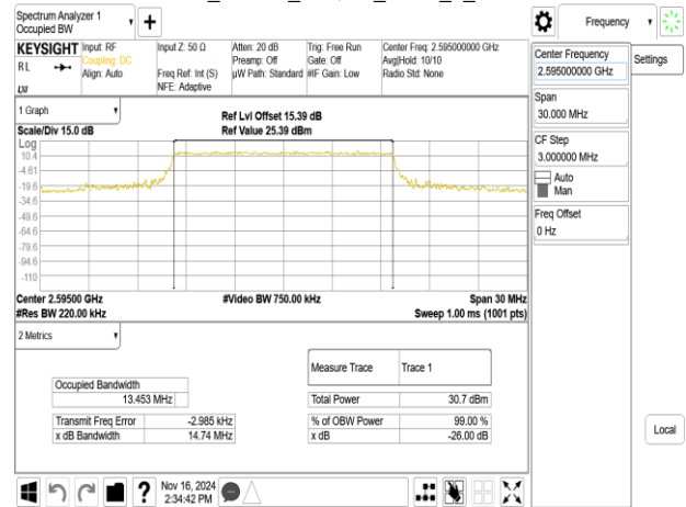
Band38_15MHz_64QAM_RB75_0_CH38000
