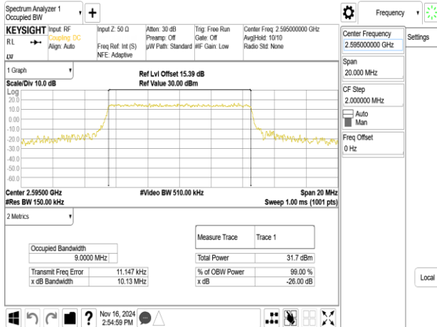
Band38_10MHz_QPSK_RB50_0_CH38000
