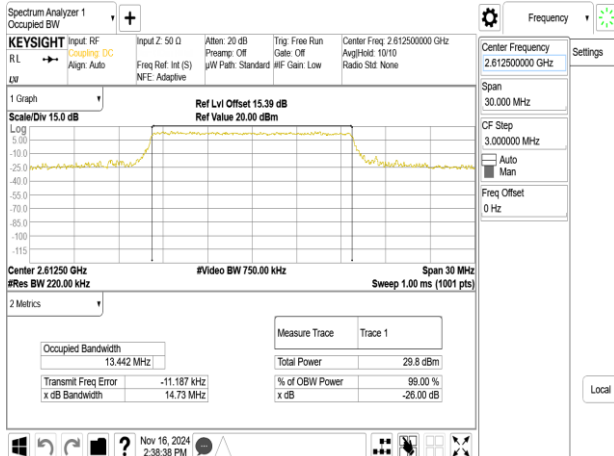
Band38_15MHz_64QAM_RB75_0_CH38175
