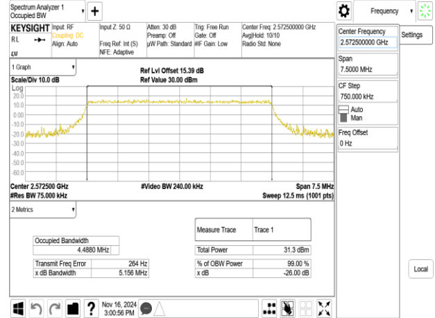
Band38_5MHz_16QAM_RB25_0_CH37775
