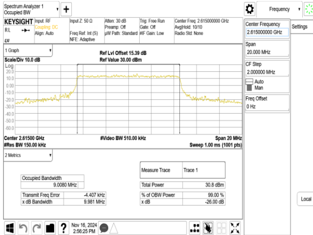
Band38_10MHz_64QAM_RB50_0_CH38200
