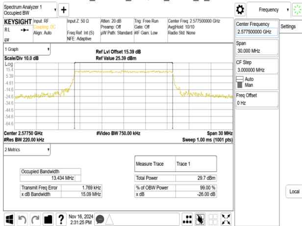
Band38_15MHz_256QAM_RB75_0_CH37825
