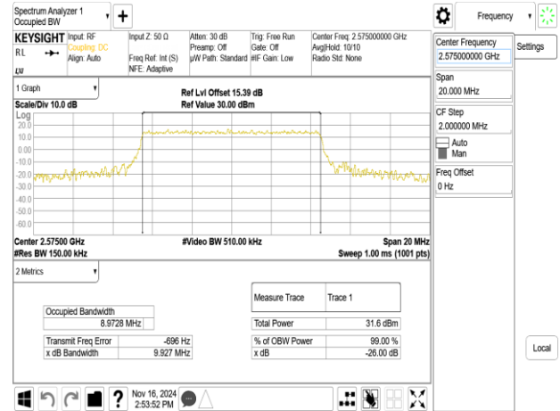
Band38_10MHz_16QAM_RB50_0_CH37800
