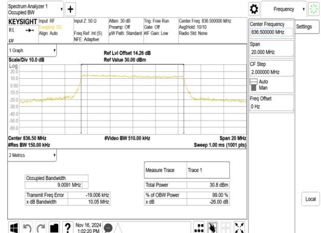
Band26_10MHz_16QAM_RB50_0_CH26915
