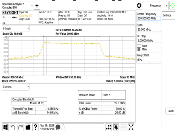
Band26_15MHz_256QAM_RB75_0_CH26915
