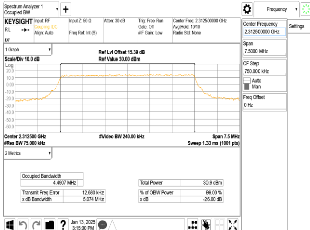
Band30_5MHz_QPSK_RB25_0_CH27735
