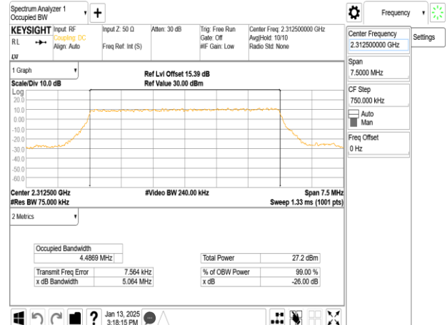
Band30_5MHz_256QAM_RB25_0_CH27735
