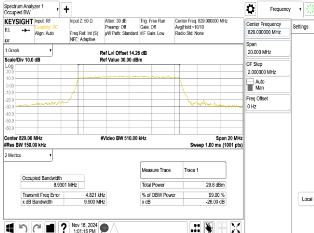
Band26_10MHz_64QAM_RB50_0_CH26840
