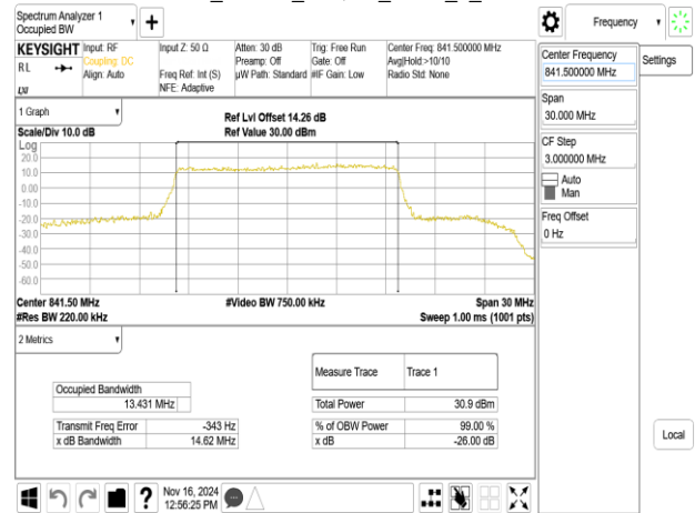
Band26_15MHz_64QAM_RB75_0_CH26965
