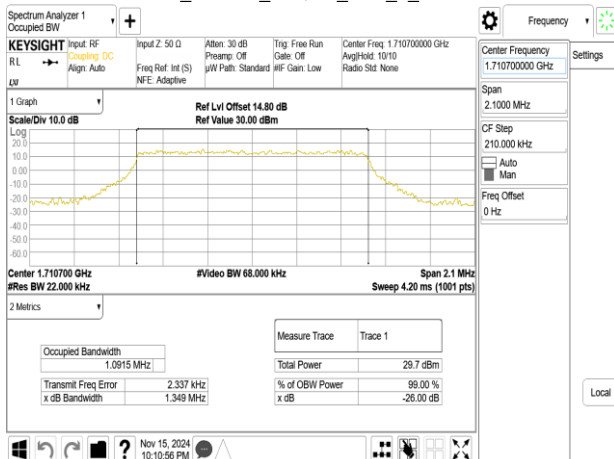
Band4_1.4MHz_64QAM_RB6_0_CH19957
