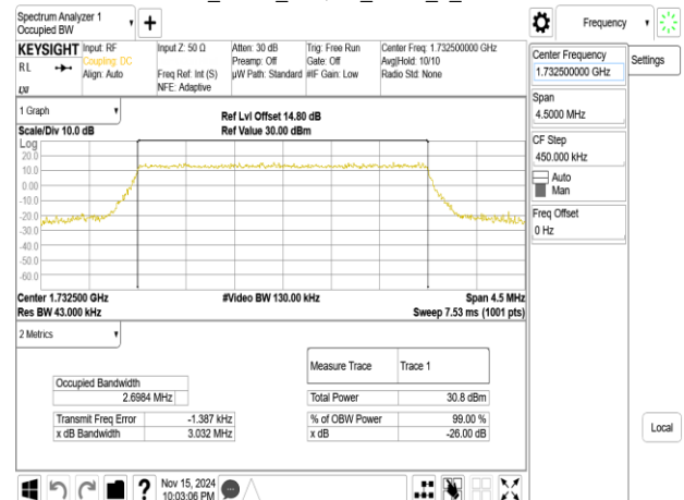
Band4_3MHz_16QAM_RB15_0_CH20175
