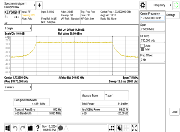
Band4_5MHz_16QAM_RB25_0_CH20175
