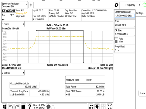
Band4_15MHz_64QAM_RB75_0_CH20025
