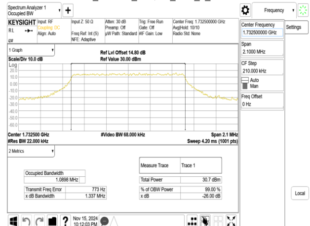
Band4_1.4MHz_16QAM_RB6_0_CH20175
