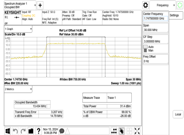
Band4_15MHz_64QAM_RB75_0_CH20325
