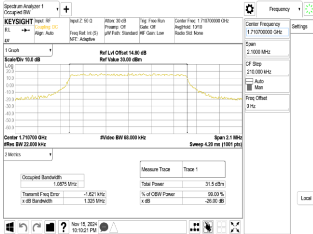
Band4_1.4MHz_16QAM_RB6_0_CH19957
