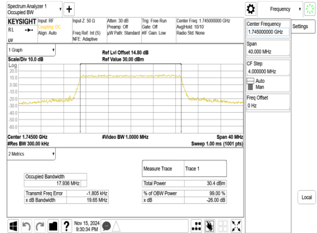
Band4_20MHz_256QAM_RB100_0_CH20300
