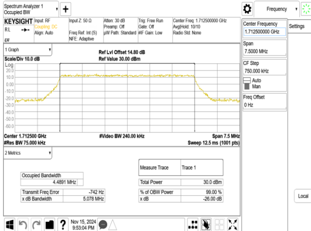
Band4_5MHz_64QAM_RB25_0_CH19975
