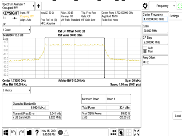
Band4_10MHz_256QAM_RB50_0_CH20175
