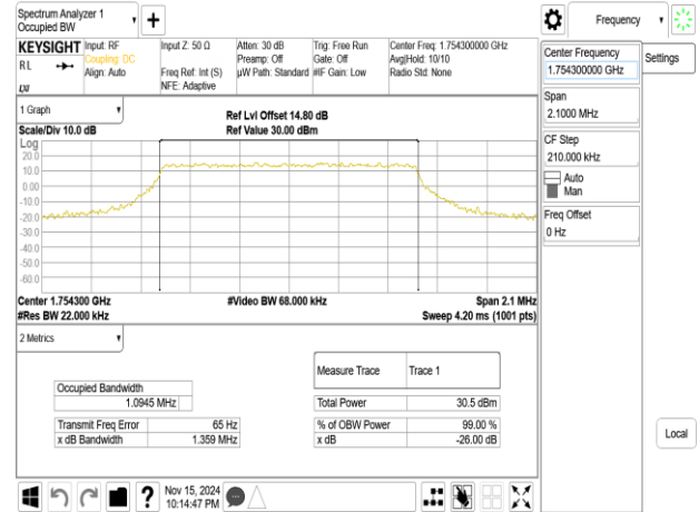
Band4_1.4MHz_64QAM_RB6_0_CH20393
