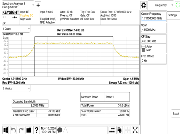
Band4_3MHz_16QAM_RB15_0_CH19965
