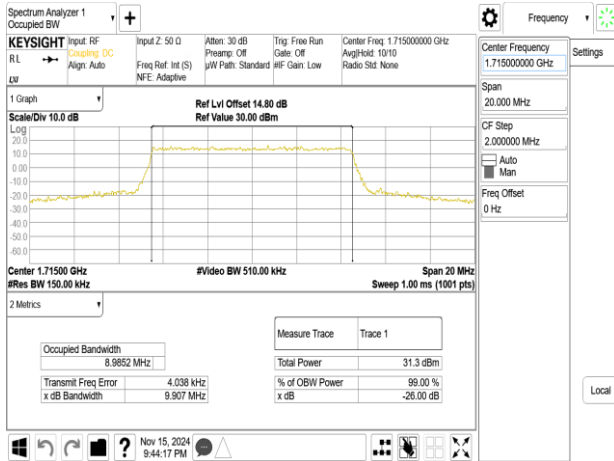
Band4_10MHz_64QAM_RB50_0_CH20000
