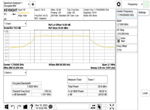
Band4_1.4MHz_256QAM_RB6_0_CH20393
