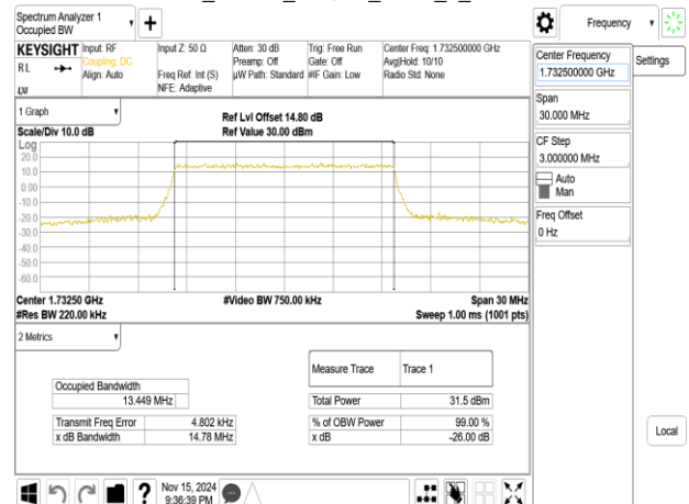
Band4_15MHz_16QAM_RB75_0_CH20175
