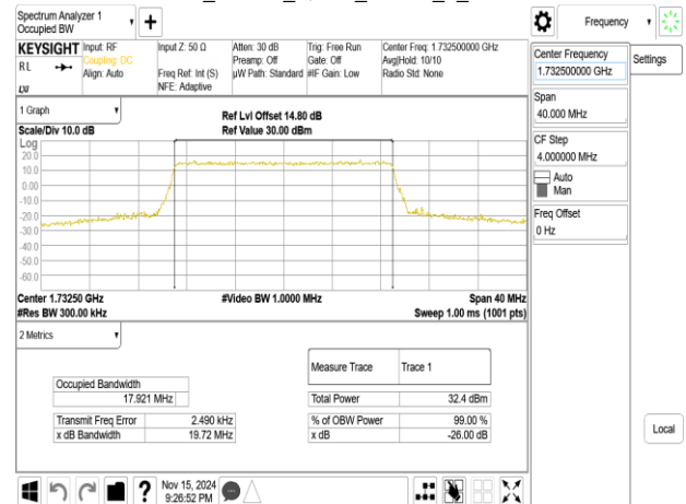
Band4_20MHz_16QAM_RB100_0_CH20175
