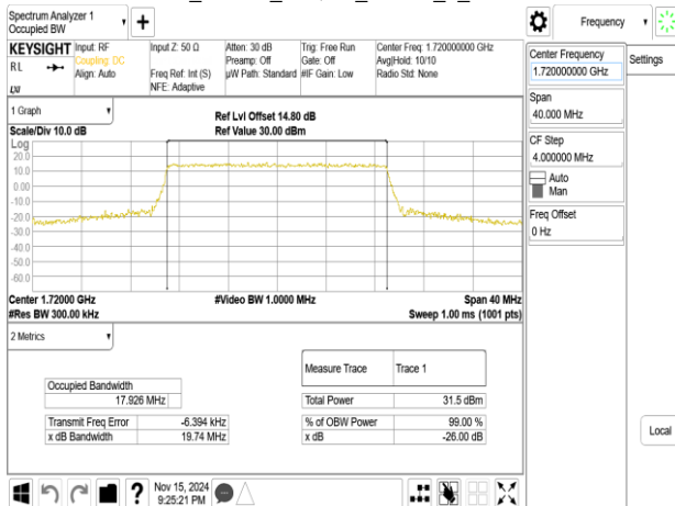
Band4_20MHz_64QAM_RB100_0_CH20050
