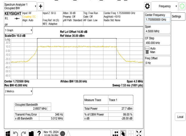
Band4_3MHz_256QAM_RB15_0_CH20385
