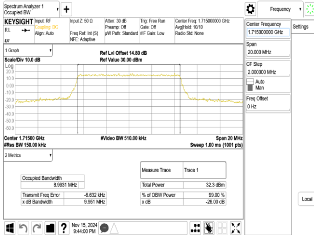
Band4_10MHz_16QAM_RB50_0_CH20000
