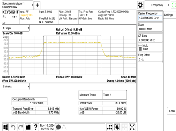
Band4_20MHz_256QAM_RB100_0_CH20175
