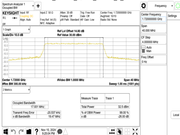
Band4_20MHz_16QAM_RB100_0_CH20050
