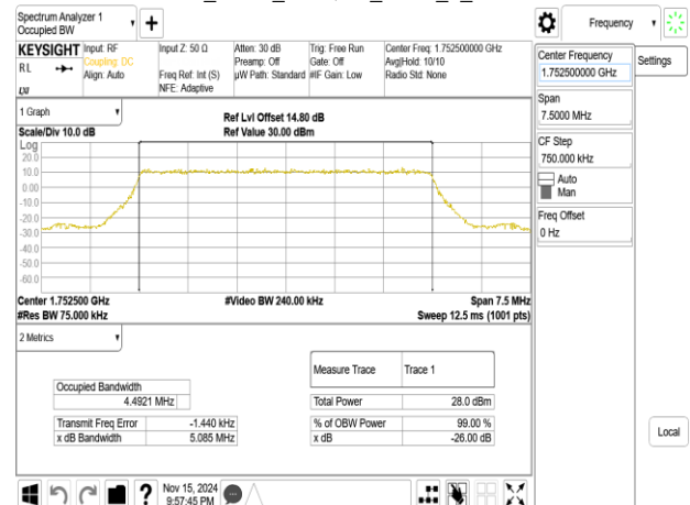
Band4_5MHz_256QAM_RB25_0_CH20375
