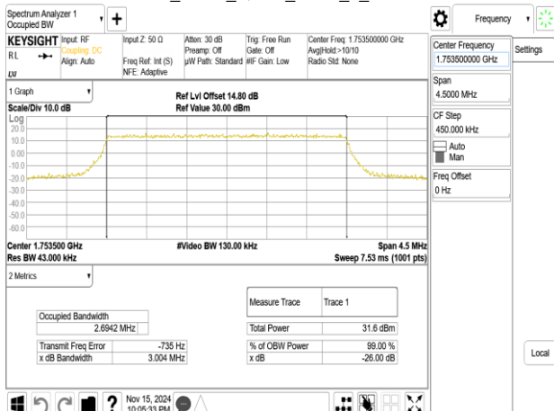
Band4_3MHz_QPSK_RB15_0_CH20385
