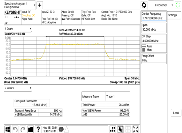
Band4_15MHz_256QAM_RB75_0_CH20325
