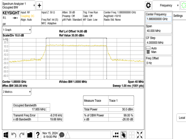
Band2_20MHz_256QAM_RB100_0_CH18900
