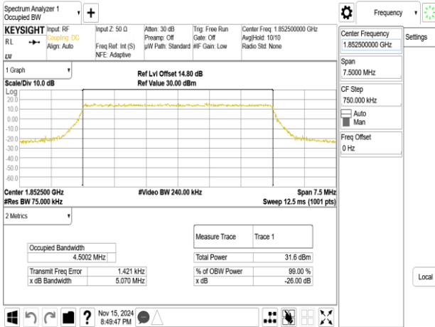
Band2_5MHz_16QAM_RB25_0_CH18625
