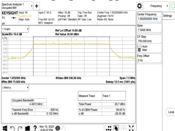
Band2_5MHz_64QAM_RB25_0_CH18625
