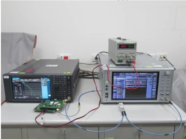
LTE_Conducted_Setup(2)
