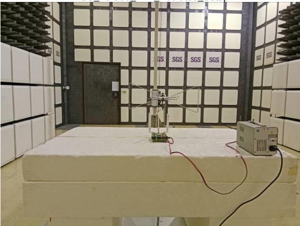
FCC Part 96 FR1 Radiated Setup
