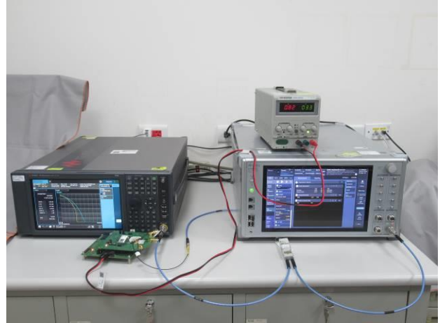
FCC_Part 96_LTE_Conducted_Setup(2)
