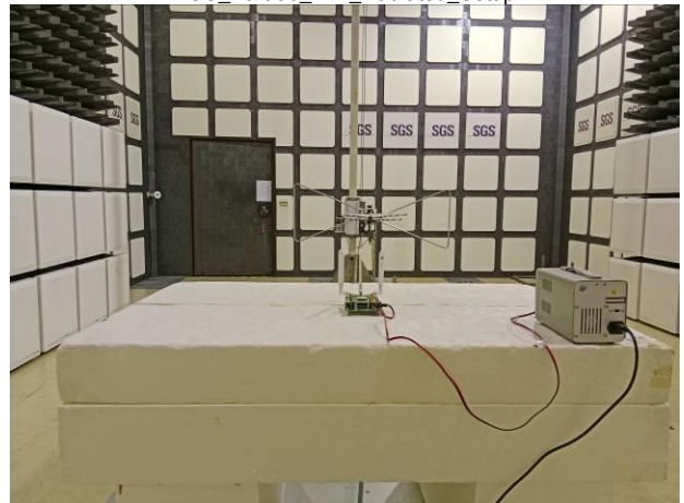
FCC Part 96 LTE Radiated Setup
