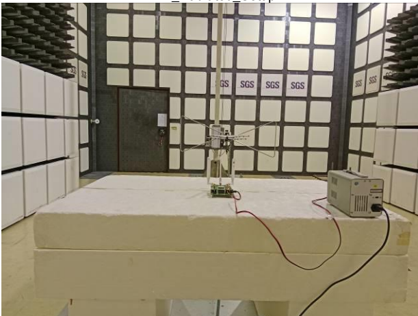
FR1_Radiated_Setup
