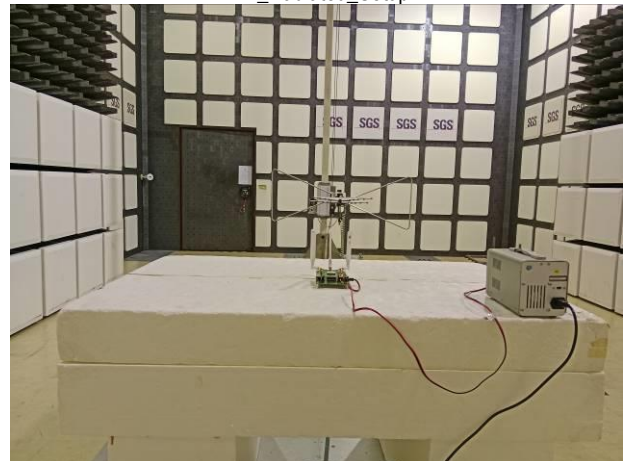
LTE_Radiated_Setup
