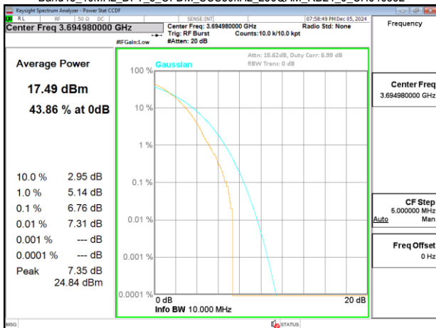
Band48_10MHz_DFT_s_OFDM_SCS30kHz_256QAM_RB24_0_CH646332
