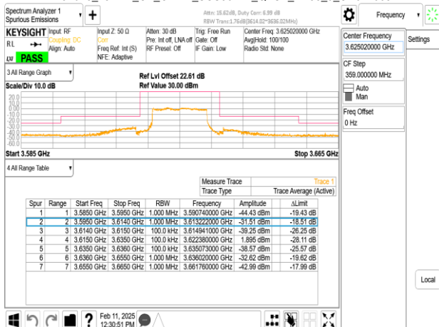
Band48_15MHz_CP_OFDM_SCS30kHz_QPSK_RB38_0_CH641668
