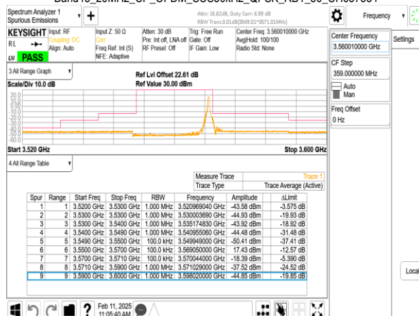
Band48_20MHz_CP_OFDM_SCS30kHz_QPSK_RB51_0_CH637334
