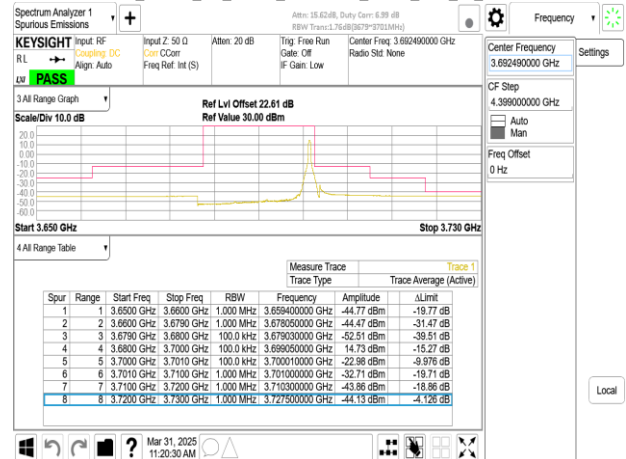
Band48_15MHz_CP_OFDM_SCS30kHz_QPSK_RB38_0_CH646166
