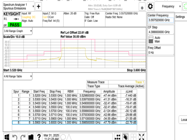
Band48_15MHz_CP_OFDM_SCS30kHz_QPSK_RB38_0_CH637168
