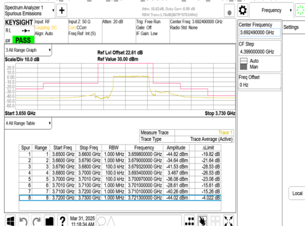
Band48_15MHz_DFT_s_OFDM_SCS30kHz_BPSK_RB36_0_CH646166
