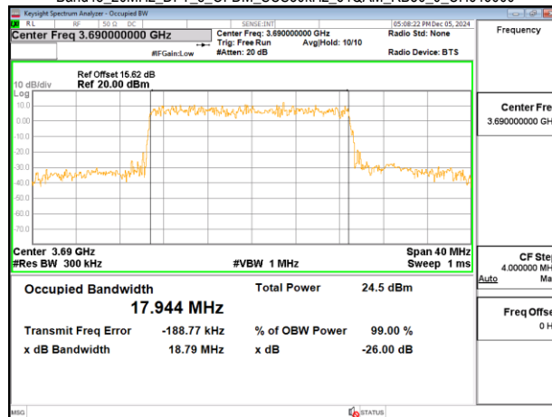
Band48_20MHz_DFT_s_OFDM_SCS30kHz_64QAM_RB50_0_CH646000
