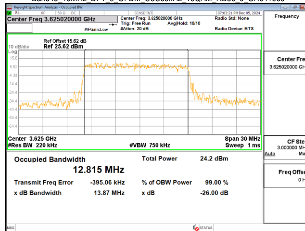
Band48_15MHz_DFT_s_OFDM_SCS30kHz_16QAM_RB36_0_CH646166
