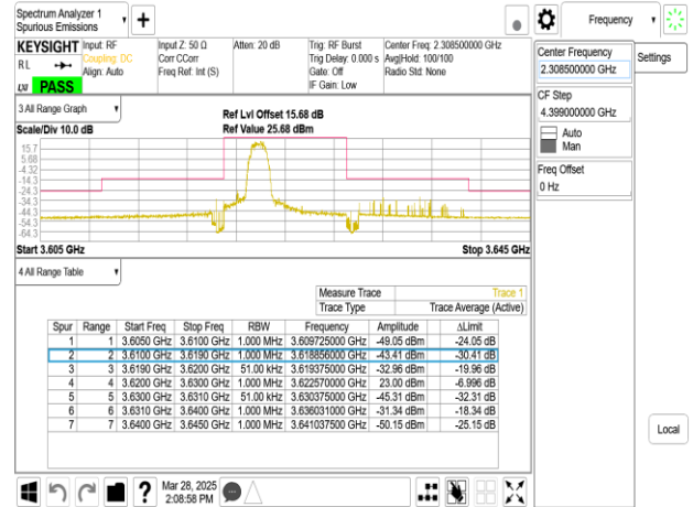
Band48_5MHz_QPSK_RB1_24_CH55990
