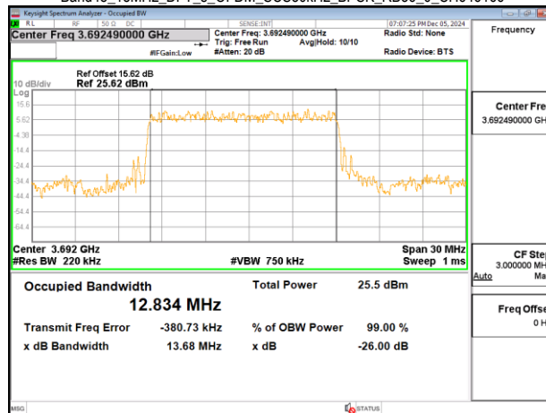
Band48_15MHz_DFT_s_OFDM_SCS30kHz_BPSK_RB36_0_CH646166
