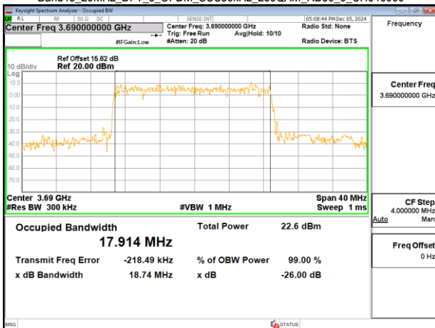
Band48_20MHz_DFT_s_OFDM_SCS30kHz_256QAM_RB50_0_CH646000
