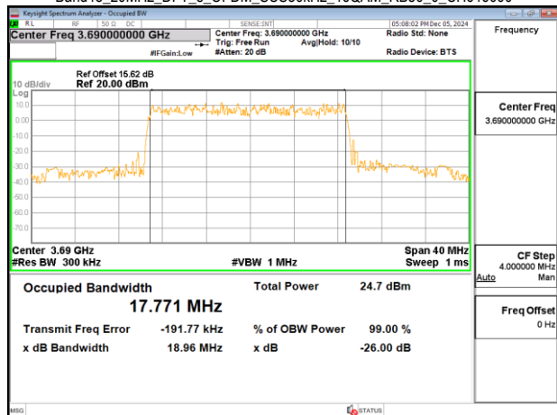
Band48_20MHz_DFT_s_OFDM_SCS30kHz_16QAM_RB50_0_CH646000
