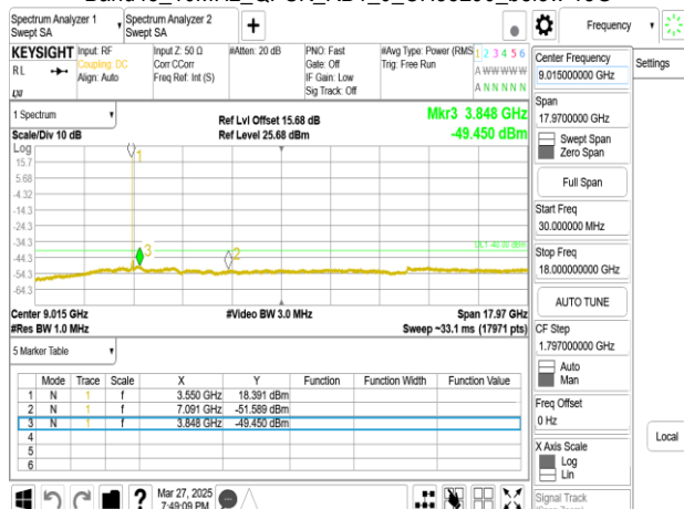
Band48_10MHz_QPSK_RB1_0_CH55290_upper 18G
