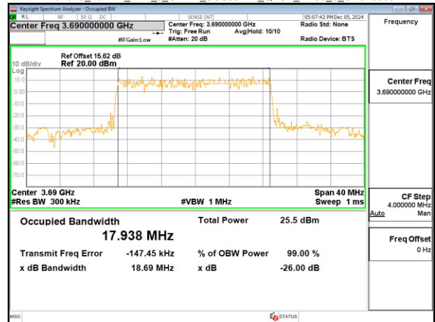
Band48_20MHz_DFT_s_OFDM_SCS30kHz_QPSK_RB50_0_CH646000
