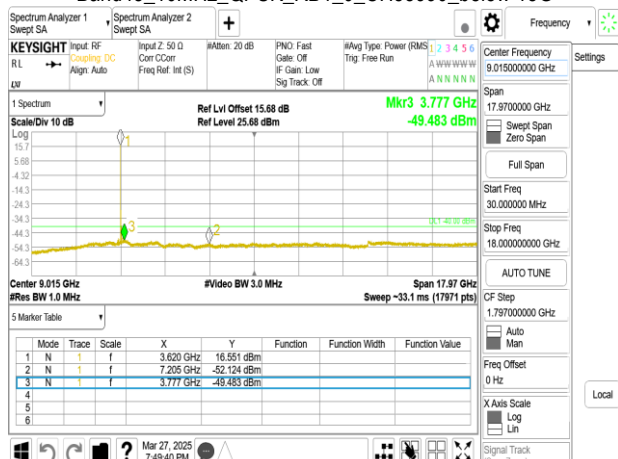
Band48_10MHz_QPSK_RB1_0_CH55990_below 18G
