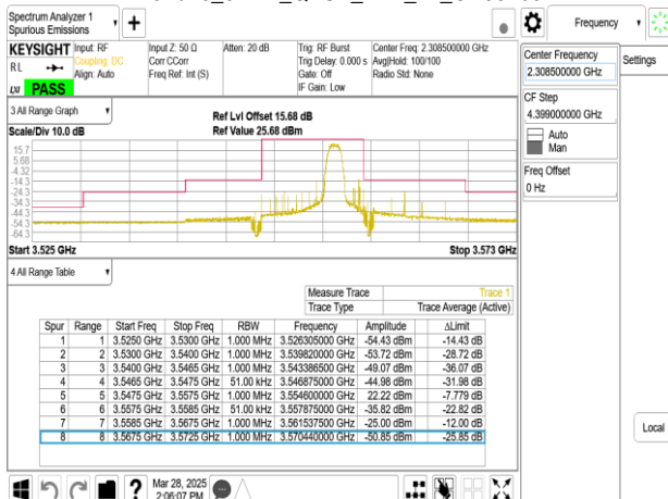
Band48_5MHz_QPSK_RB25_0_CH55265
