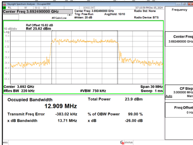
Band48_15MHz_DFT_s_OFDM_SCS30kHz_64QAM_RB36_0_CH646166
