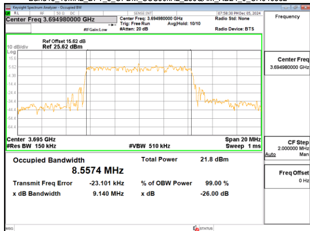
Band48_10MHz_DFT_s_OFDM_SCS30kHz_256QAM_RB24_0_CH646332
