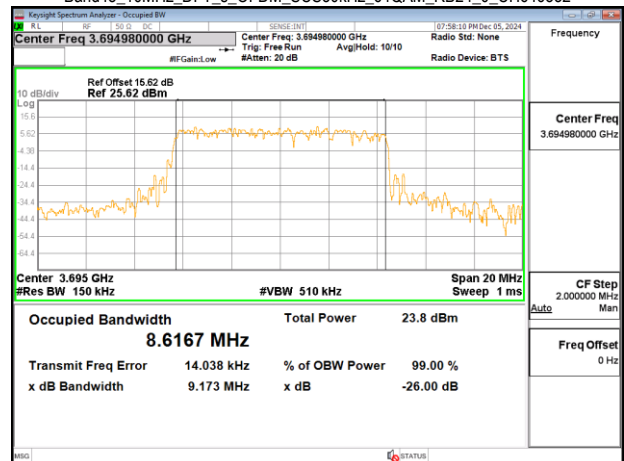
Band48_10MHz_DFT_s_OFDM_SCS30kHz_64QAM_RB24_0_CH646332
