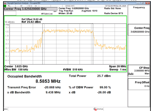
Band48_10MHz_DFT_s_OFDM_SCS30kHz_QPSK_RB24_0_CH646332
