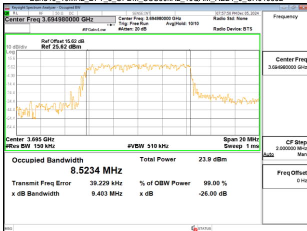
Band48_10MHz_DFT_s_OFDM_SCS30kHz_16QAM_RB24_0_CH646332
