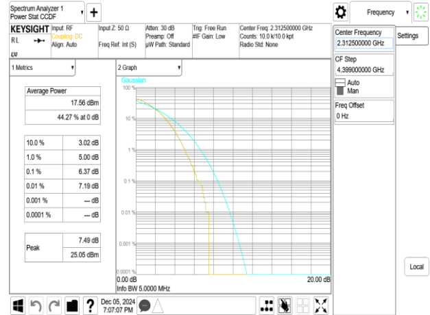
Band30_10MHz_256QAM_RB50_0_CH27710
