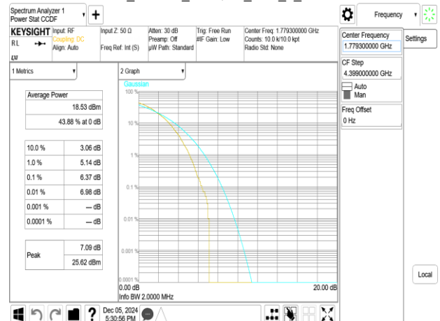
Band66_1.4MHz_256QAM_RB6_0_CH132665
