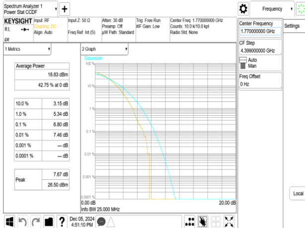
Band66_20MHz_256QAM_RB100_0_CH132572
