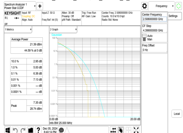
Band41_20MHz_256QAM_RB100_0_CH39750
