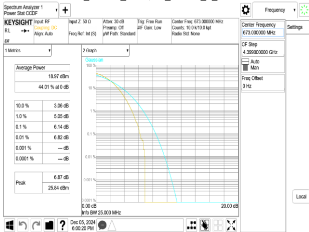
Band71_20MHz_256QAM_RB100_0_CH133297
