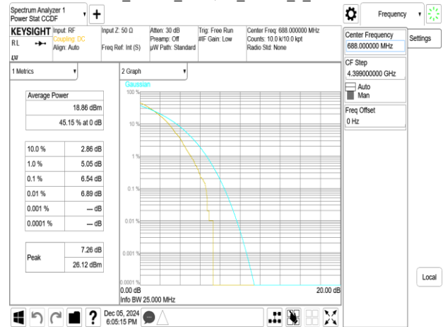
Band71_20MHz_256QAM_RB100_0_CH133372
