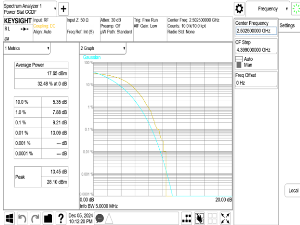
Band41_5MHz_256QAM_RB25_0_CH40620
