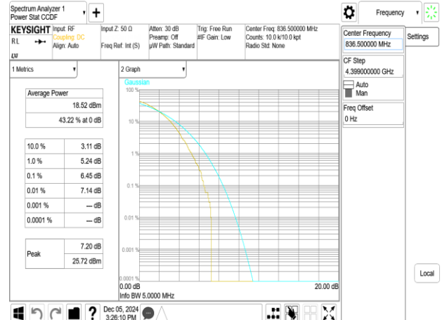
Band26_5MHz_256QAM_RB25_0_CH26915
