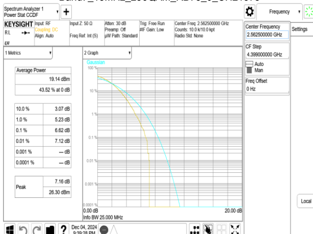
Band7_15MHz_256QAM_RB75_0_CH21375
