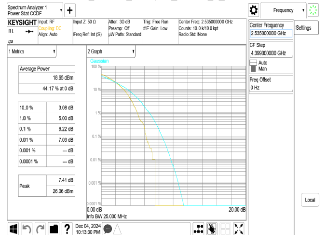
Band7_20MHz_256QAM_RB100_0_CH21350
