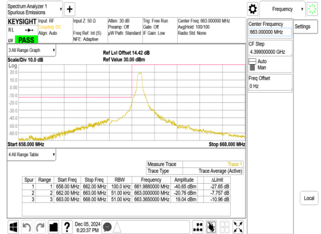
Band71_5MHz_QPSK_RB25_0_CH133147
