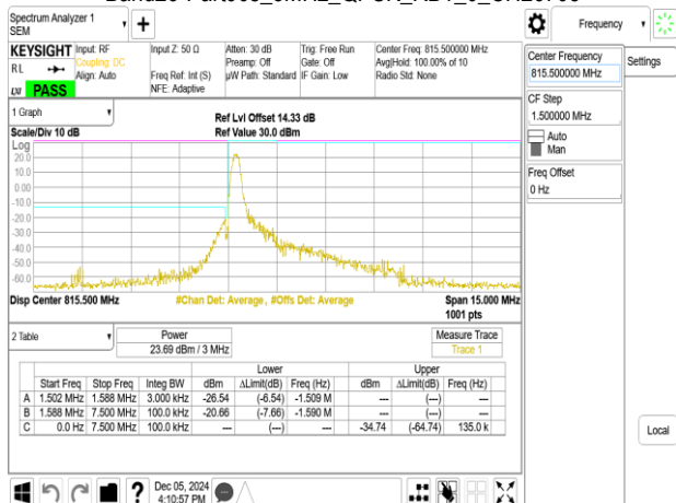
Band26-Part90s_3MHz_QPSK_RB15_0_CH26705
