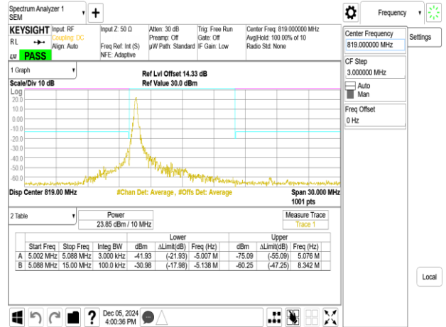
Band26-Part90s_10MHz_QPSK_RB1_49_CH26740
