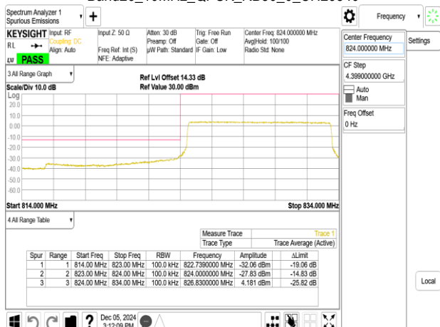
Band26_10MHz_QPSK_RB50_0_CH26840
