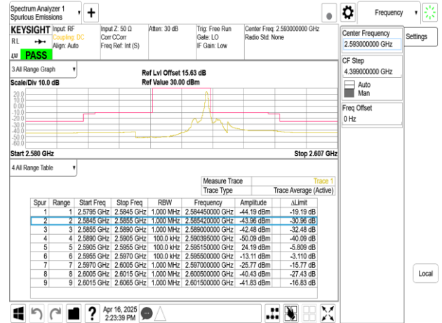
Band41_5MHz_QPSK_RB25_0_CH40620
