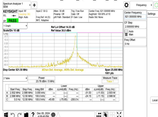
Band26-Part90s_5MHz_QPSK_RB25_0_CH26765
