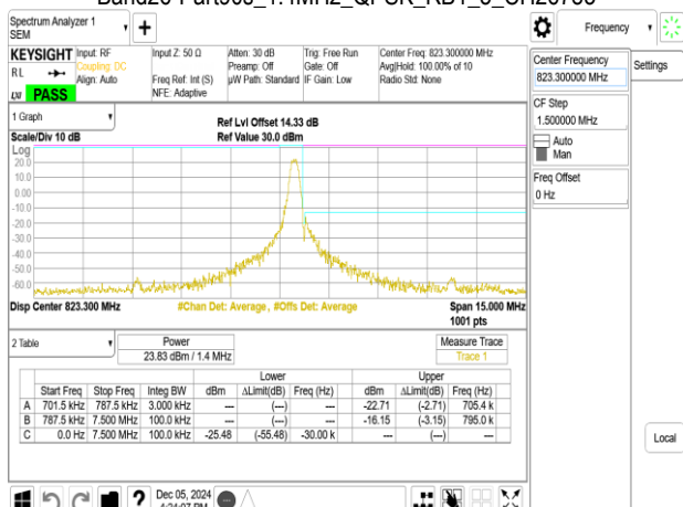
Band26-Part90s_1.4MHz_QPSK_RB6_0_CH26783
