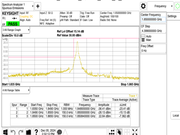
Band25_15MHz_QPSK_RB1_0_CH26115
