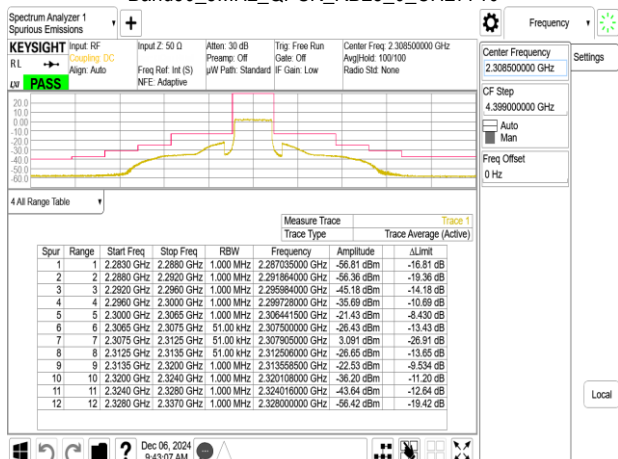
Band30_5MHz_QPSK_RB25_0_CH27710
