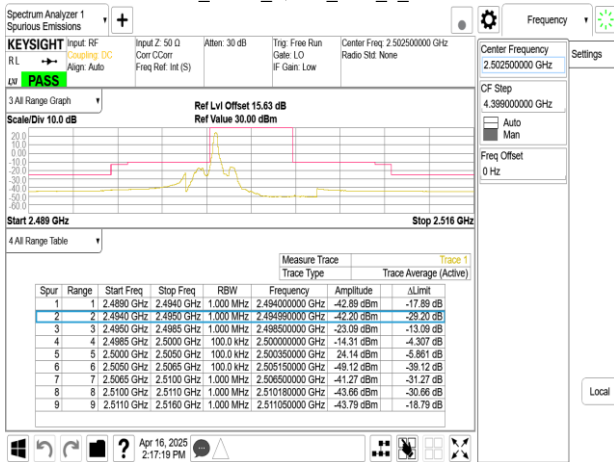
Band41_5MHz_QPSK_RB1_24_CH39715
