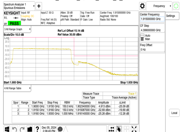
Band25_15MHz_QPSK_RB75_0_CH26615
