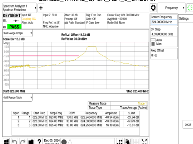
Band26_1.4MHz_QPSK_RB1_0_CH26797
