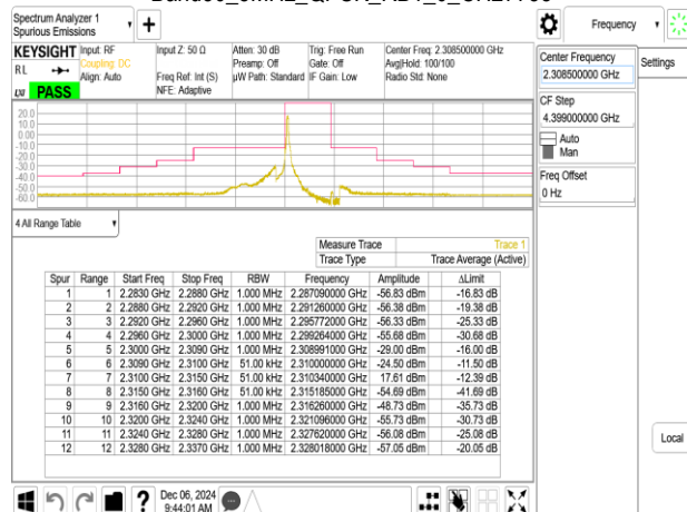
Band30_5MHz_QPSK_RB1_24_CH27735
