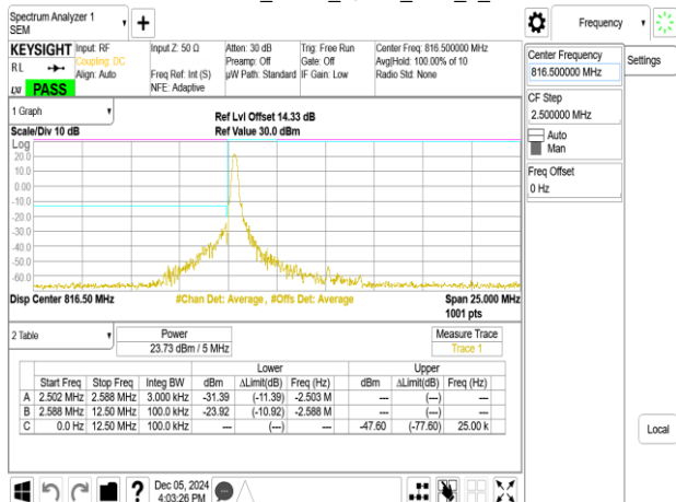
Band26-Part90s_5MHz_QPSK_RB1_0_CH26715
