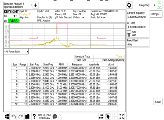
Band30_5MHz_QPSK_RB1_24_CH27685
