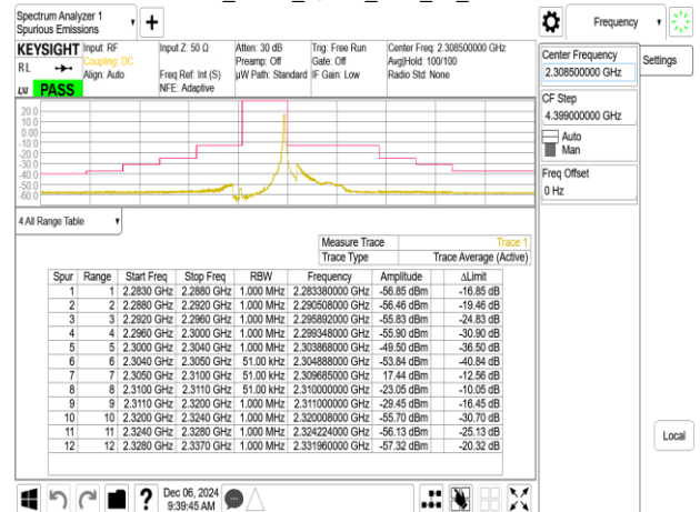
Band30_5MHz_QPSK_RB25_0_CH27685
