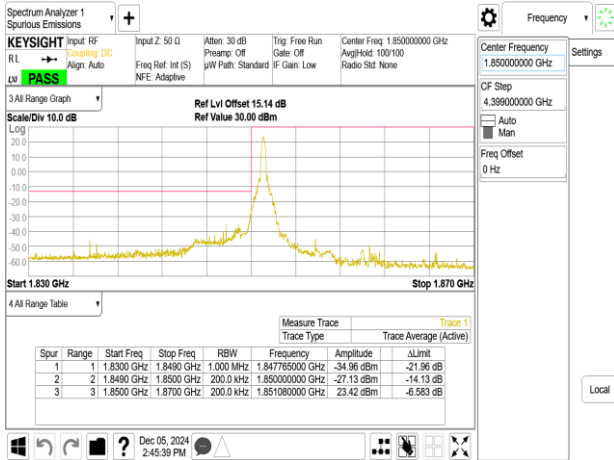
Band25_20MHz_QPSK_RB100_0_CH26140
