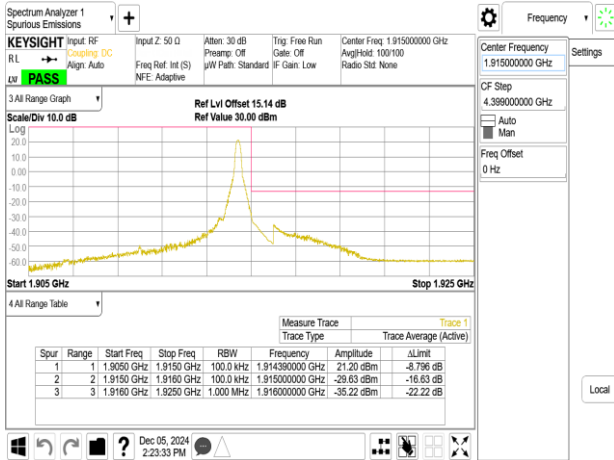
Band25_10MHz_QPSK_RB50_0_CH26640
