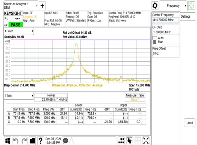
Band26-Part90s_1.4MHz_QPSK_RB6_0_CH26697
