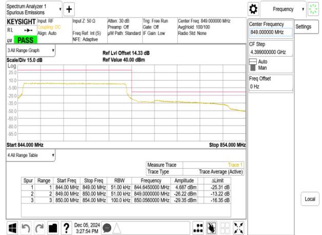
Band26-Part90s_10MHz_QPSK_RB1_0_CH26740
