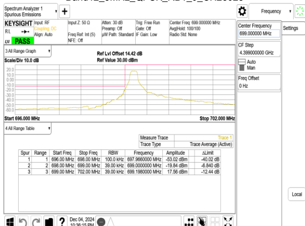
Band12_3MHz_QPSK_RB1_0_CH23025
