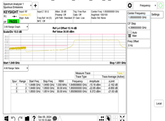
Band25_1.4MHz_QPSK_RB6_0_CH26047
