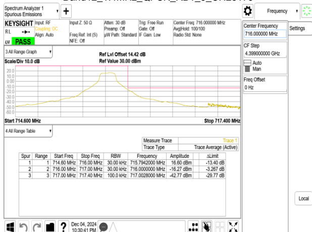
Band12_1.4MHz_QPSK_RB6_0_CH23173
