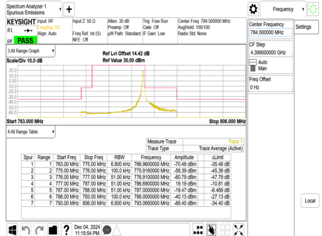
Band13_5MHz_QPSK_RB25_0_CH23255
