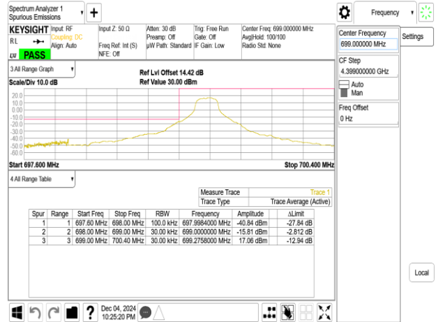
Band12_1.4MHz_QPSK_RB6_0_CH23017
