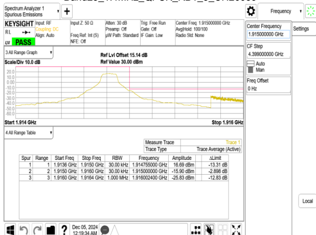
Band25_1.4MHz_QPSK_RB6_0_CH26683
