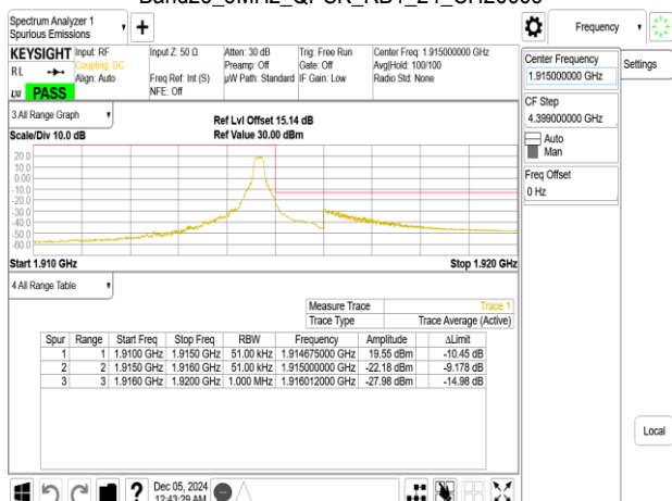
Band25_5MHz_QPSK_RB1_24_CH26665
