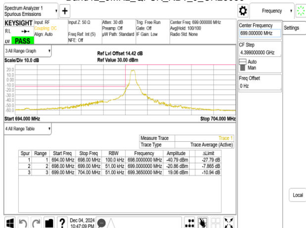
Band12_5MHz_QPSK_RB25_0_CH23035
