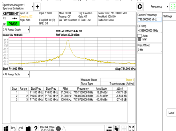
Band12_5MHz_QPSK_RB1_24_CH23155
