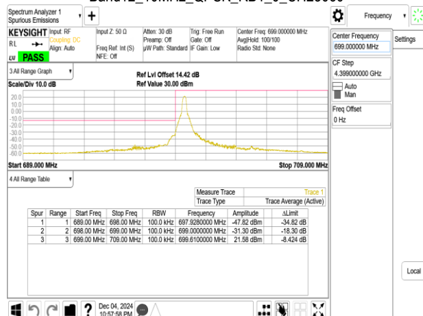
Band12_10MHz_QPSK_RB50_0_CH23060
