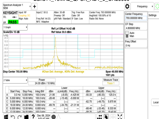
Band14_10MHz_QPSK_RB1_0_CH23330
