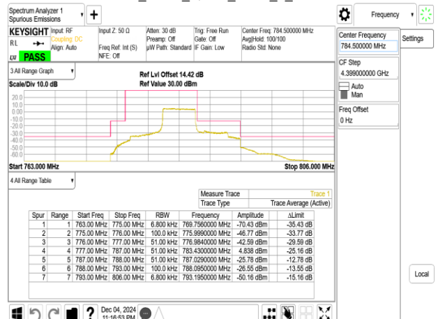
Band13_5MHz_QPSK_RB25_0_CH23255
