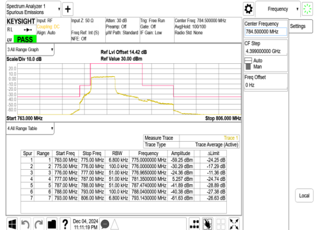
Band13_5MHz_QPSK_RB1_24_CH23255
