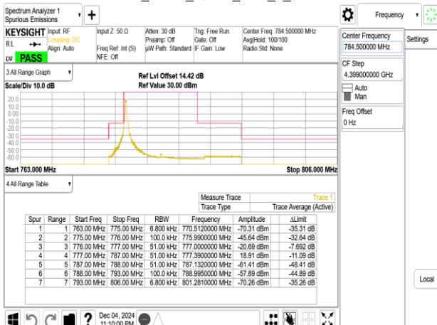
Band13_5MHz_QPSK_RB1_0_CH23205
